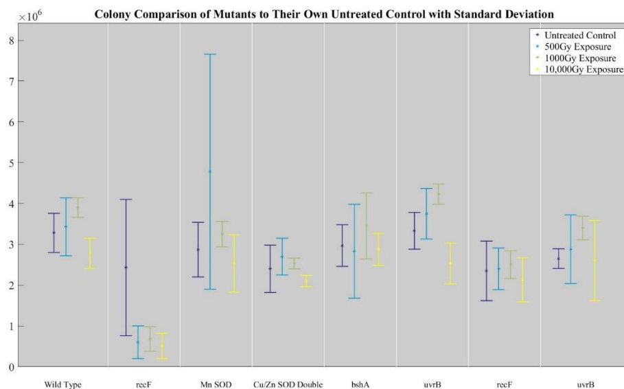
Figure 27. Colony comparison of mutants to their own untreated control with standard deviation
