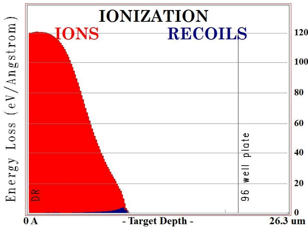
Figure 13. Energy loss of the bombarding particles due to ionizations in \text{eV } \text{\AA}^{-1} . Recoils are the secondary ions created from knock-on collisions from the incident particles. The method of ionization is irrelevant to this research.
