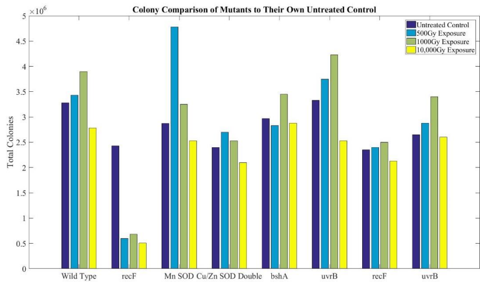
Figure 26. Colony comparison of mutants to their own untreated control
