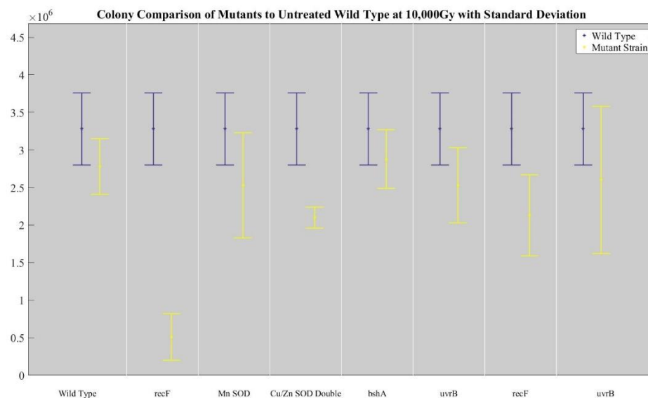
Figure 25. Colony omparison of mutants to untreated wild type at 10,000Gy with standard deviation
