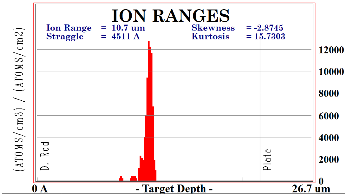
Figure 7. Chart showing the penetration depth of 15 MeV silicon ions into Dr. It is approximately 10.7um.
