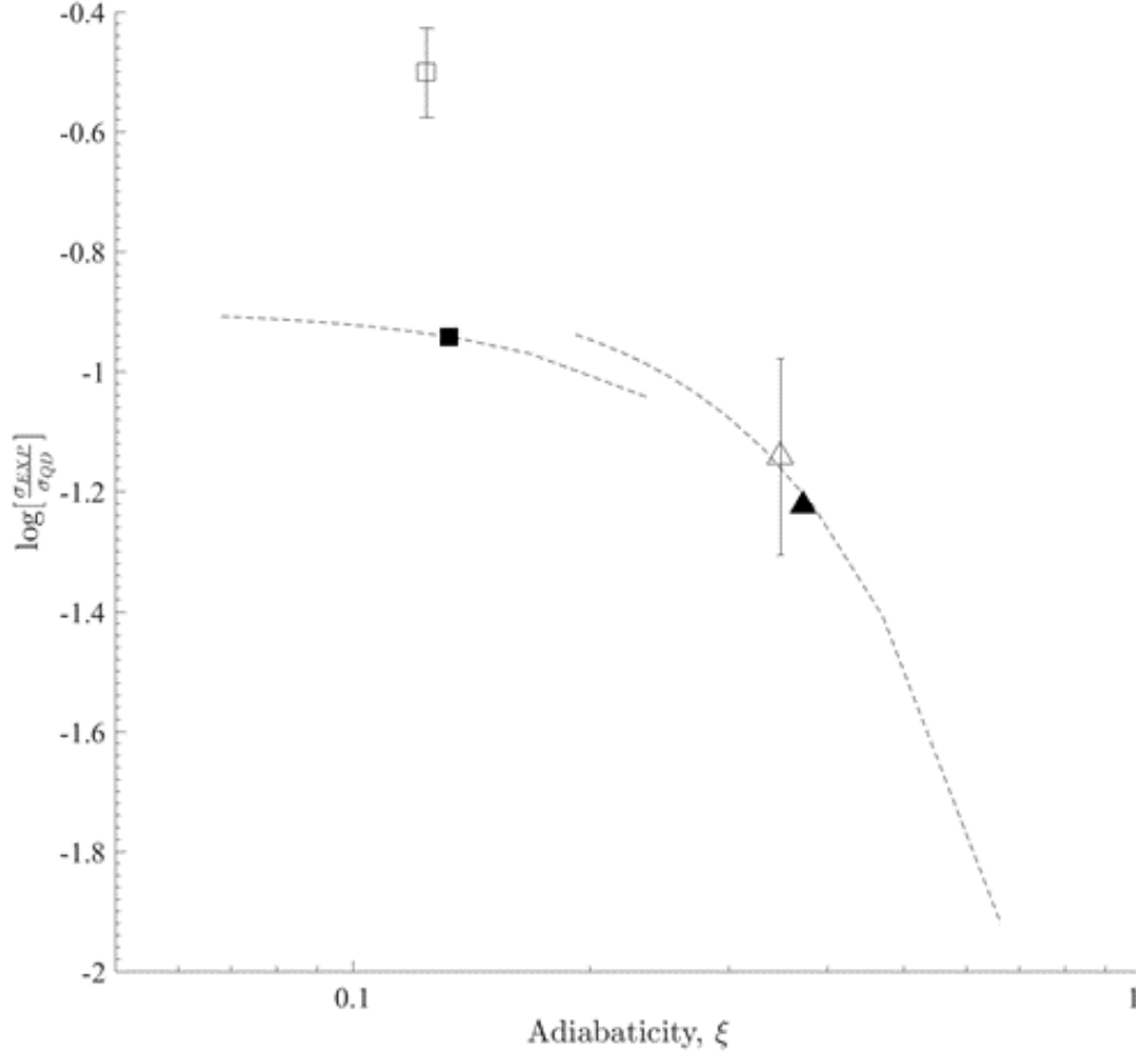
Figure 4.8: Temperature scaling for Cs 8^2D fine structure mixing rates for: ( \blacksquare, \square ) He and ( \blacktriangle, \triangle ) Ar from: ( \square, \triangle ) Reference [55] and ( \blacksquare, \blacktriangle ) present work. (---) Prediction from perturbation theory of Equation (4.12) using L = 5\text{\AA} , w = 3\text{\AA} , V_o = 0.1119 Hartree for He and 0.1221 H for Ar and temperatures T = 100 - 1200 K.
