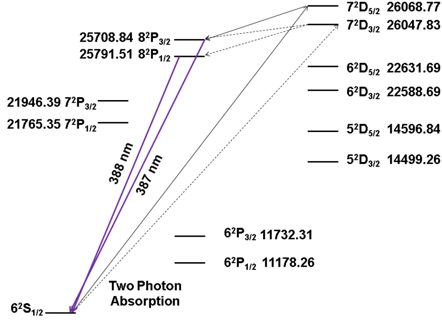
Figure 5.14: Cs ultraviolet 8^2P_{3/2, 1/2} \rightarrow 6^2S_{1/2} emissions after pulsed laser pumping of 6^2S_{1/2} \rightarrow 7^2D_{3/2} .
