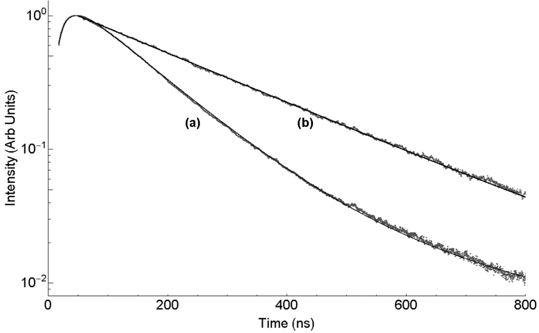
Figure 4.3: Emission on 8^2D_{3/2} \rightarrow 6^2P_{1/2} at 601 nm after excitation on 8^2D_{5/2} for Ar pressures of (a) 200 Torr and (b) 0.6 Torr. A fit to Equation (4.1) is also provided.
