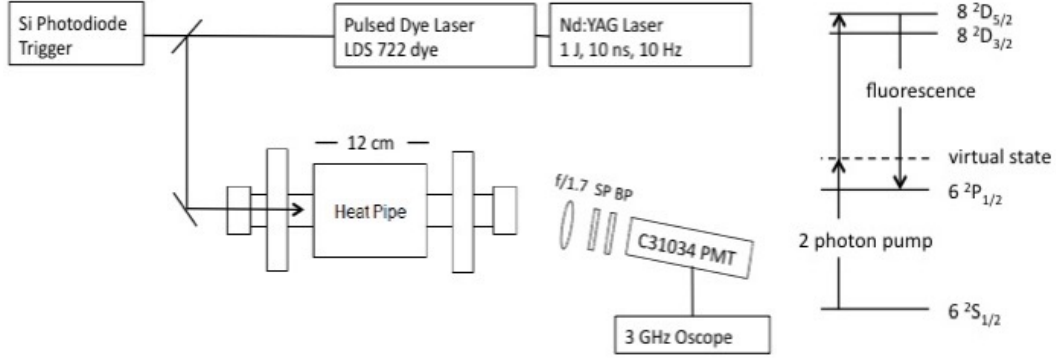
Figure 4.1: Temporally-resolved laser induced fluorescence apparatus and cesium energy levels for the 8^2D fine structure collisional mixing.
