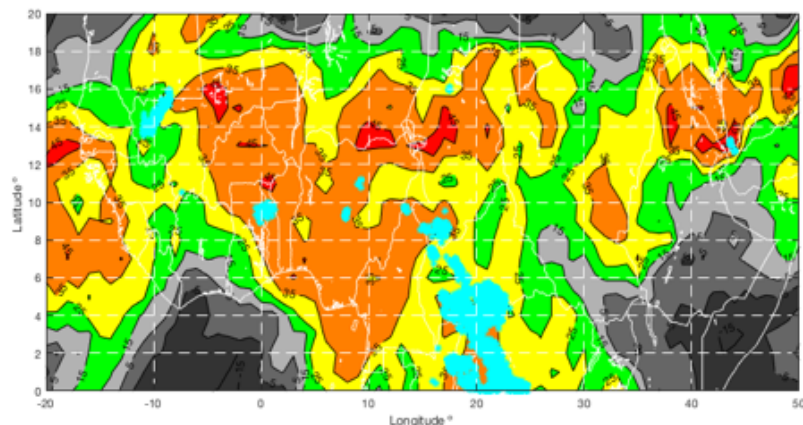
Figure 3.3: GDI values (colored contours) at 15 August 2016 at 06Z, with Sferics lighting data (cyan asterisks) from 15 August 2016 from 05-07Z.
