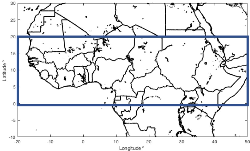
Figure 1.1: The blue rectangle outlines the region of interest, 0^{\circ} - 20^{\circ} N latitude and 20^{\circ} W- 50^{\circ} E longitude.
