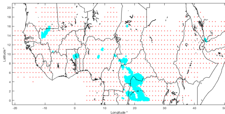
Figure 3.7: KI values 30 and above (red dots) and lightning data (cyan asterisks) on 15 August 2016 at 06Z.
