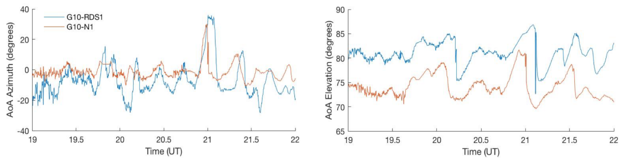
Figure 3. Example plot of AoA measurements for G10-RDS1 and G10-N1. Left: AoA azimuth angle versus time. Right: AoA elevation angle versus time.
