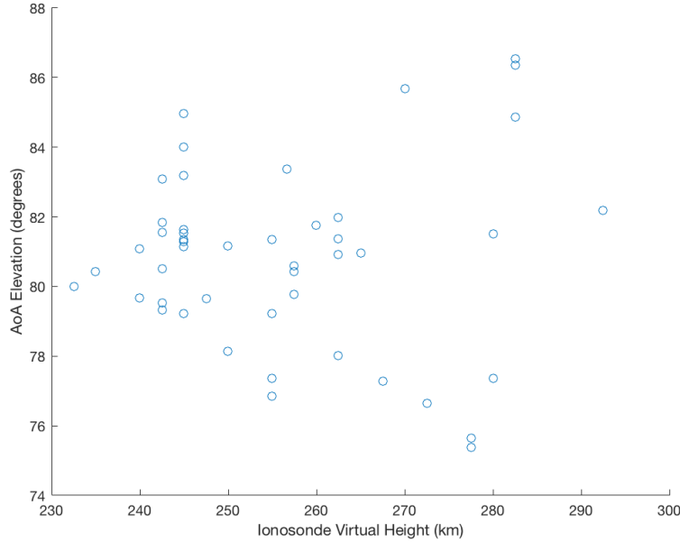
Figure 23. TID period scatter plot of Figure 22, G10-RDS1 AoA elevation angle and Squirt ionosonde virtual height measurements during a TID. The correlation values are: r=0.03 and p\text{-value}=0.84 .
