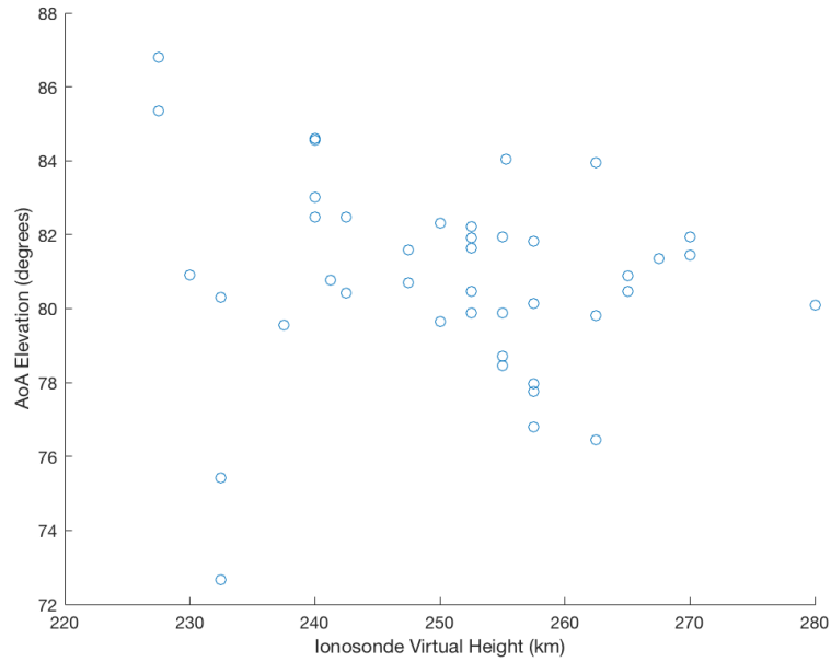
Figure 27. TID period scatter plot of Figure 26, G10-RDS1 AoA elevation angle and Kirtland ionosonde virtual height measurements during a TID. The correlation values are: r=-0.13 and p\text{-value}=0.40 .
