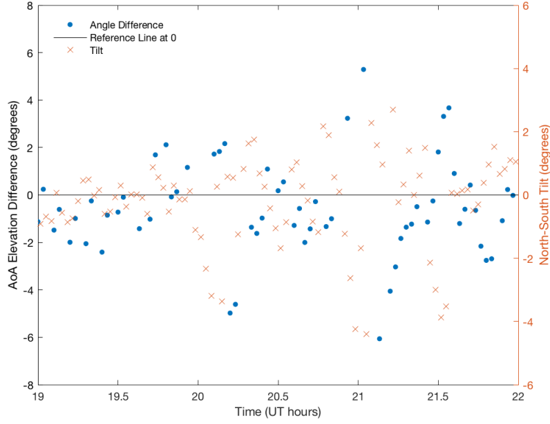
Figure 54. Plot to compare the simple MM for G10-POL with the time shifted Munyo ionosonde North-South tilt measurements. When the tilt is near 0^\circ (horizontal reference line), the angle difference in the MM and actual AoA elevation angles is small which suggests the simple MM performs well. However, as the tilt increases, so too does the angle differences and the simple MM should not be considered.
