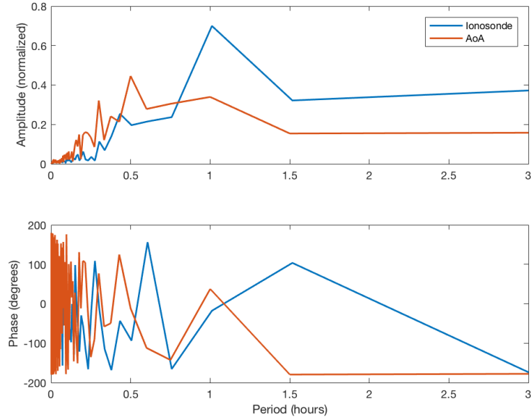
Figure 35. DFT of G10-RDS1 AoA and Squirr ionosonde measurements. The peak wave amplitude of the TID at G10-RDS1 AoA occurs at a 30 minute period, and at Squirr occurs at a 1 hour period.
