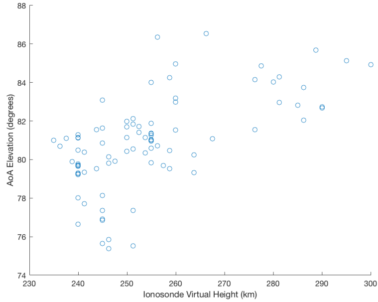
Figure 21. TID period scatter plot of Figure 20, G10-RDS1 AoA elevation angle and Cherry ionosonde virtual height measurements during a TID. The correlation values are: r=0.61 and p\text{-value}=0.00 .
