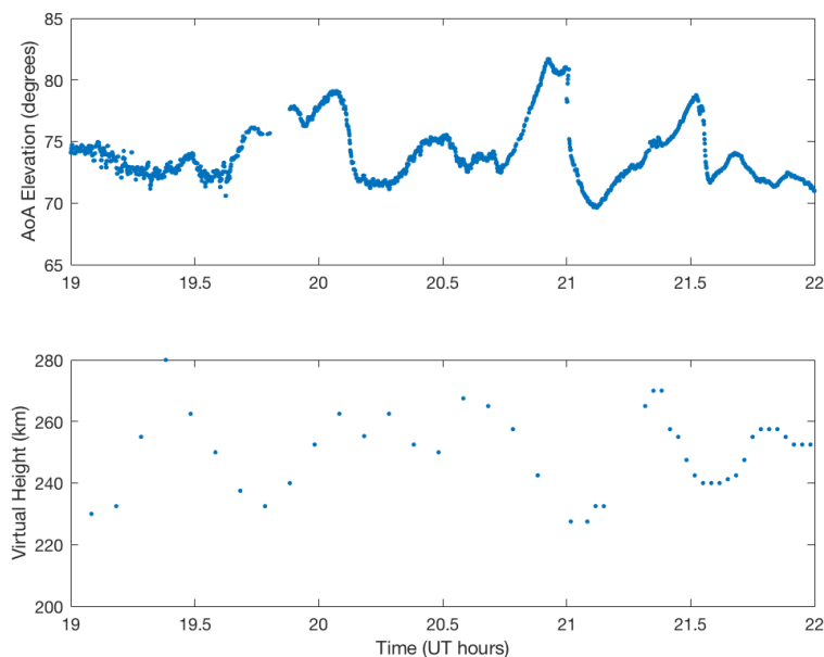
Figure 30. Measurements of G10-N1 AoA elevation angle and Kirtland ionosonde virtual height for 5.34 MHz frequency on 26 Jan 2014 from 1900-2200 UT.
