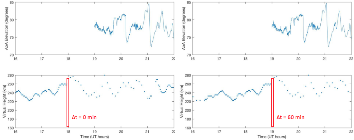
Figure 43. Two figures of G10-POL AoA elevation angle and Kirtland ionosonde virtual height measurements during TID period. The figure on the left is the ionosonde virtual height measurements observed at Kirtland with no time shift, and the figure on the right are the same measurements after a +60 minute time shift is applied to the virtual heights.
