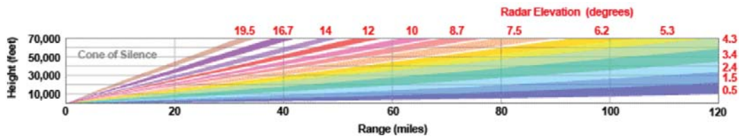
Figure 5. An example of the elevation angles utilized in one of the precipitation mode VCPs. Public domain image from NWS 2017b.
