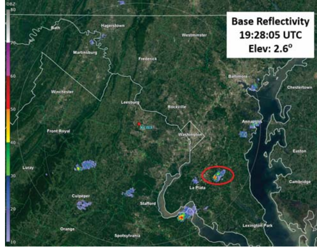
Figure 26. Radar image of the base reflectivity for Case 1 (red oval) used in the analysis. The image was from 19:28:05 UTC at an elevation angle of 2.6^\circ .
