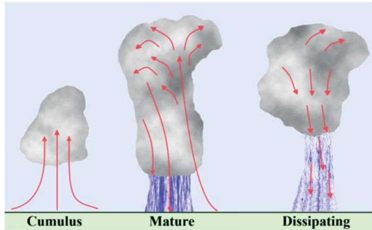
Figure 1. A depiction of the three stages of single-cell thunderstorm development. The mature stage clearly shows the upward and downward flow of the updraft and downdraft. Image from Travis (2015).
