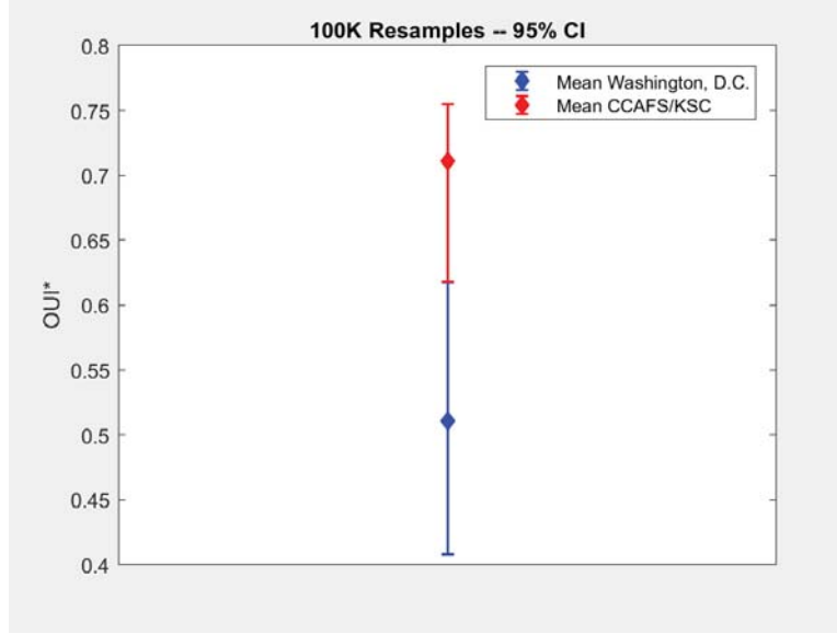
Figure 30. 95% confidence intervals of the mean OUI* for Travis (2015) and this study. The confidence intervals were created using the bootstrap technique with 100,000 resamples and values from the original sample, identified by the closed circles. It is important to note that the MATLAB bootstrap code used randomly samples the cases to generate new POD, TSS, and PFA values (in addition to lead times changing) for each OUI* resample to generate the OUI* plot. The confidence interval shows that 95% of the time the values will fall within these error bars. Results for CCAFS/KSC are given in red and Washington, D.C. in blue. Graphic created using MATLAB.
