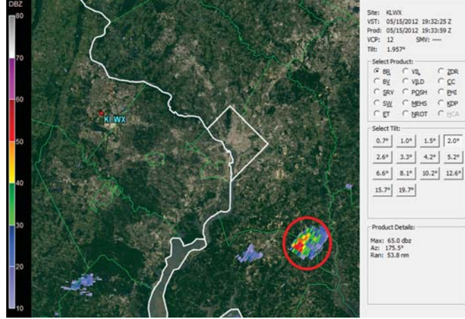
Figure 18. Example of a case used in the analysis as it met the set criteria for an isolated convective cell. Image generated using GR2Analyst.
