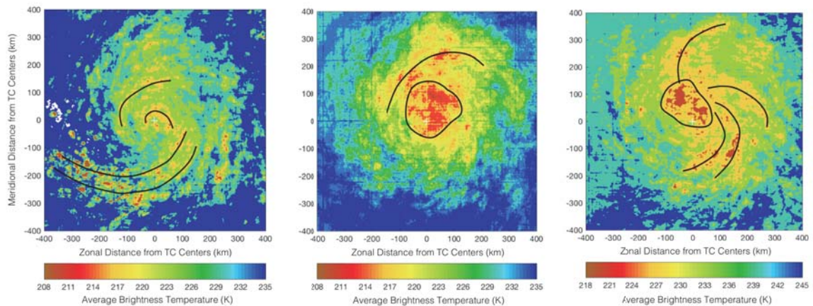
Figure 37: Composite average T_B as in Figure 35, except for Category 2.
