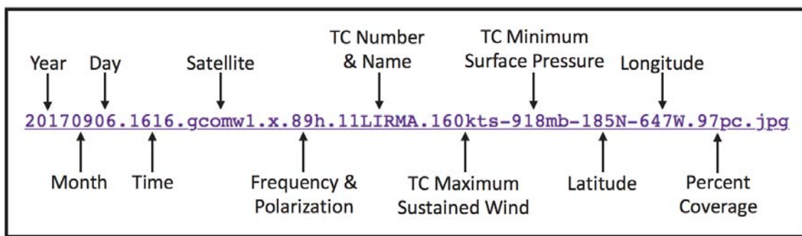
Figure 16: Sample of file name metadata for NRL rasters. This file name contains AMSR2 horizontally polarized 89 GHz imagery for Hurricane Irma (2017) from 6 September at 1616 UTC (from NRL 2017).
