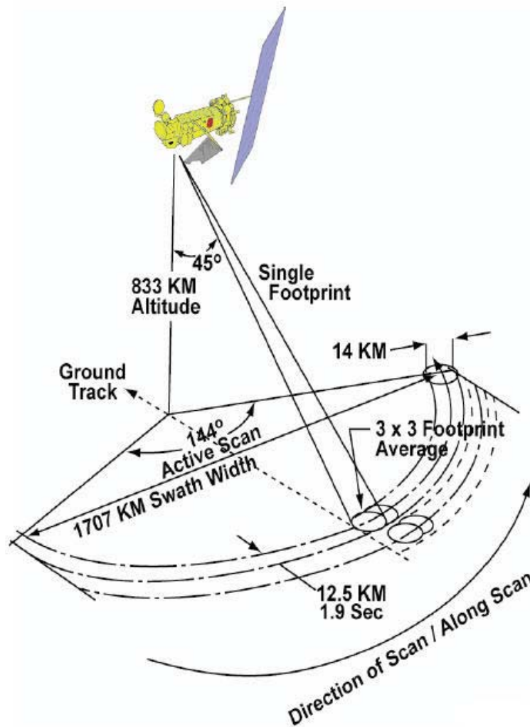
Figure 4: SSMI/S scan geometry (Poe et al. 2001).
