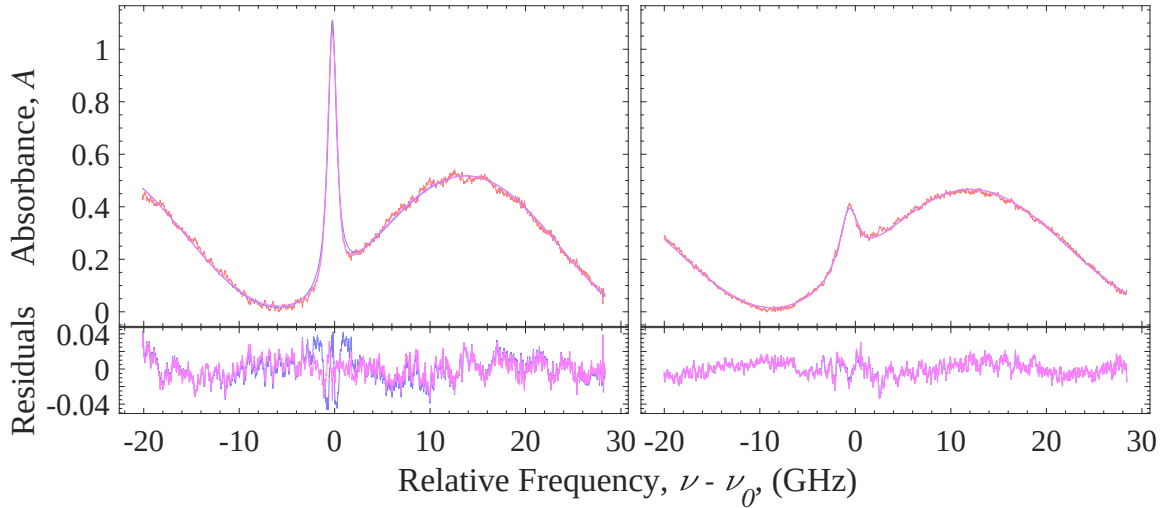
Figure 17. Voigt (magenta) and Lorentzian (blue) line shape fit comparison at 37 Torr (left) and 100 Torr (right). At 37 Torr there is a distinct difference between a Voigt and Lorentzian, but at 100 Torr the two are nearly identical.
