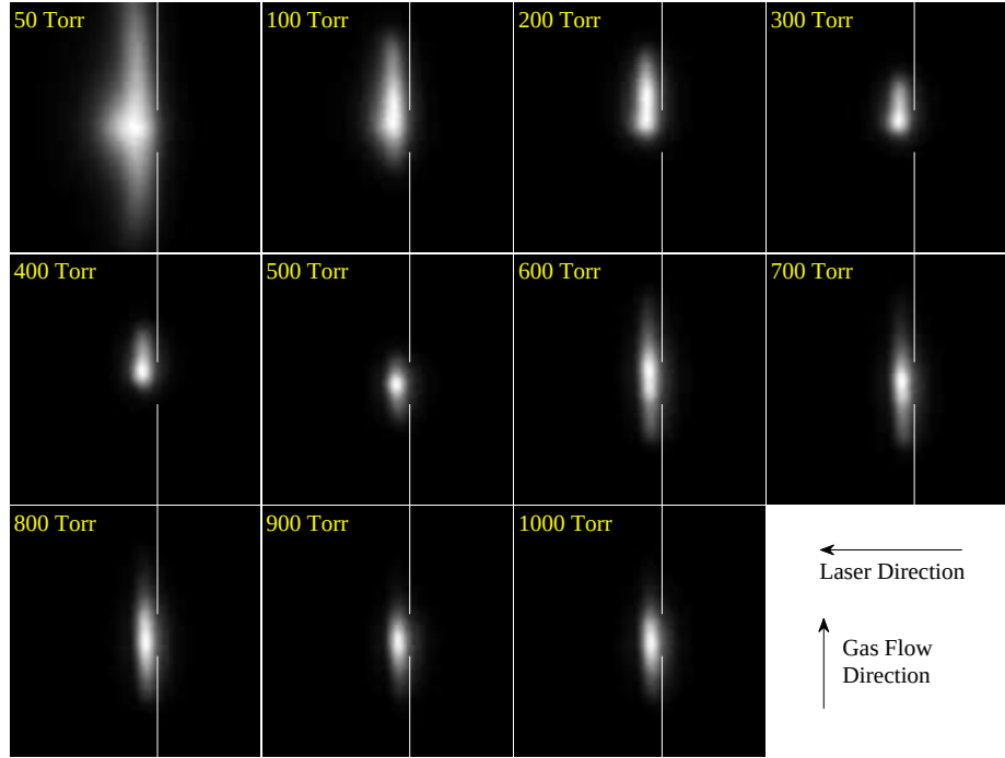
Figure 21. Side fluorescence from a 127\ \mu\text{m} thick dielectric, 200\ \mu\text{m} diameter hole MHCD. The white lines show the approximate left plate edge and hole location. The fluorescence constricts toward the plate surface as expected when pressure is increased. The asymmetry in the plasma is not expected and could be the result of plate defects such as scratches in the surface.
