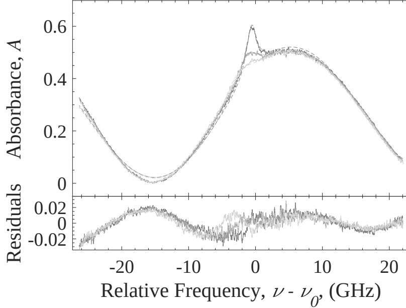
Figure 48. Absorbance data, fits, and residuals for a MHCD with a 254 \mu\text{m} thick dielectric and 400 \mu\text{m} hole diameter. The pressures ranges from 100-300 Torr in 100 Torr increments from darkest to lightest. A Lorentzian and sine function with a linear baseline were fit concurrently.
