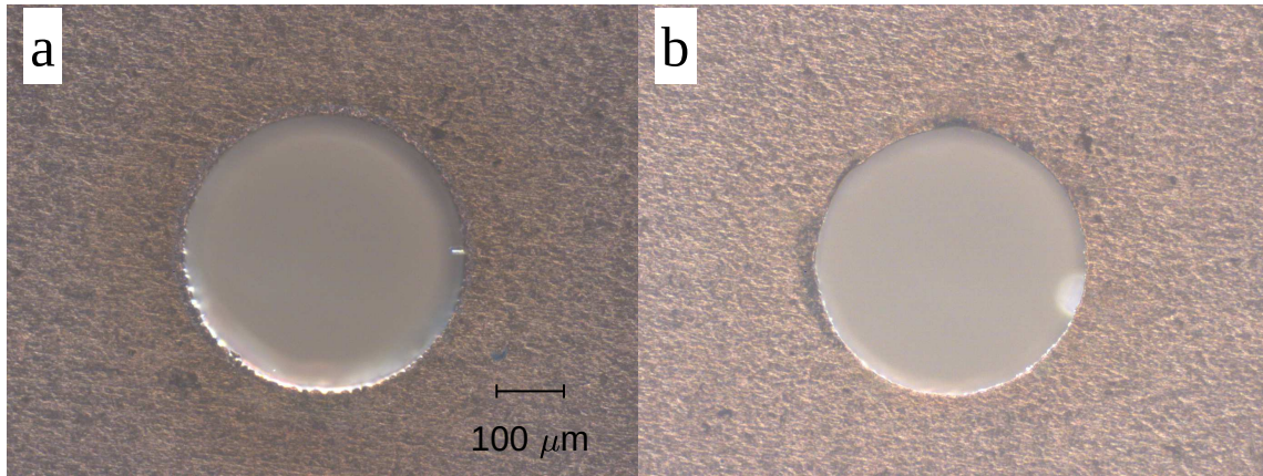
Figure 39. Images of both sides of a 400 \mu\text{m} hole before use. Actual measured diameters were (a) 423 \mu\text{m} and (b) 407 \mu\text{m} . Image (a) is the side where the laser drilling occurred. (a) There are no large jagged edges but the hole edge does appear to be rough, especially in the lower half. (b) There are few dark regions on the edge of the hole which appear burned.
