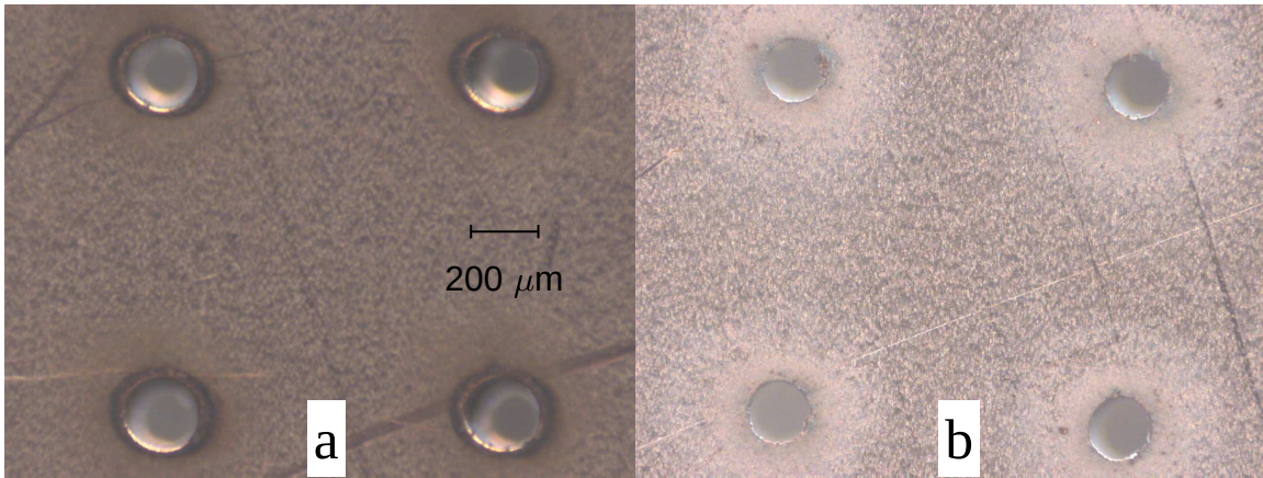
Figure 35. Images of part of an array of 200\text{ }\mu\text{m} diameter holes. Image (a) is the side where the laser drilling occurred. The plate was flipped so that the holes on the left of image (b) are the back of the holes on the right of image (a). The holes are noticeably non-circular in parts, and have jagged edges in the hole. Scratches in the copper surface can also be seen on both sides of the plate.
