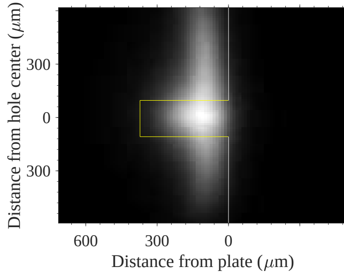
Figure 23. Side florescence from a 127 \mu\text{m} thick dielectric, 200 \mu\text{m} diameter MHCD at 50 Torr. The white lines show the approximate plate and hole location. The yellow lines show the region used to determine the maximum path length.
