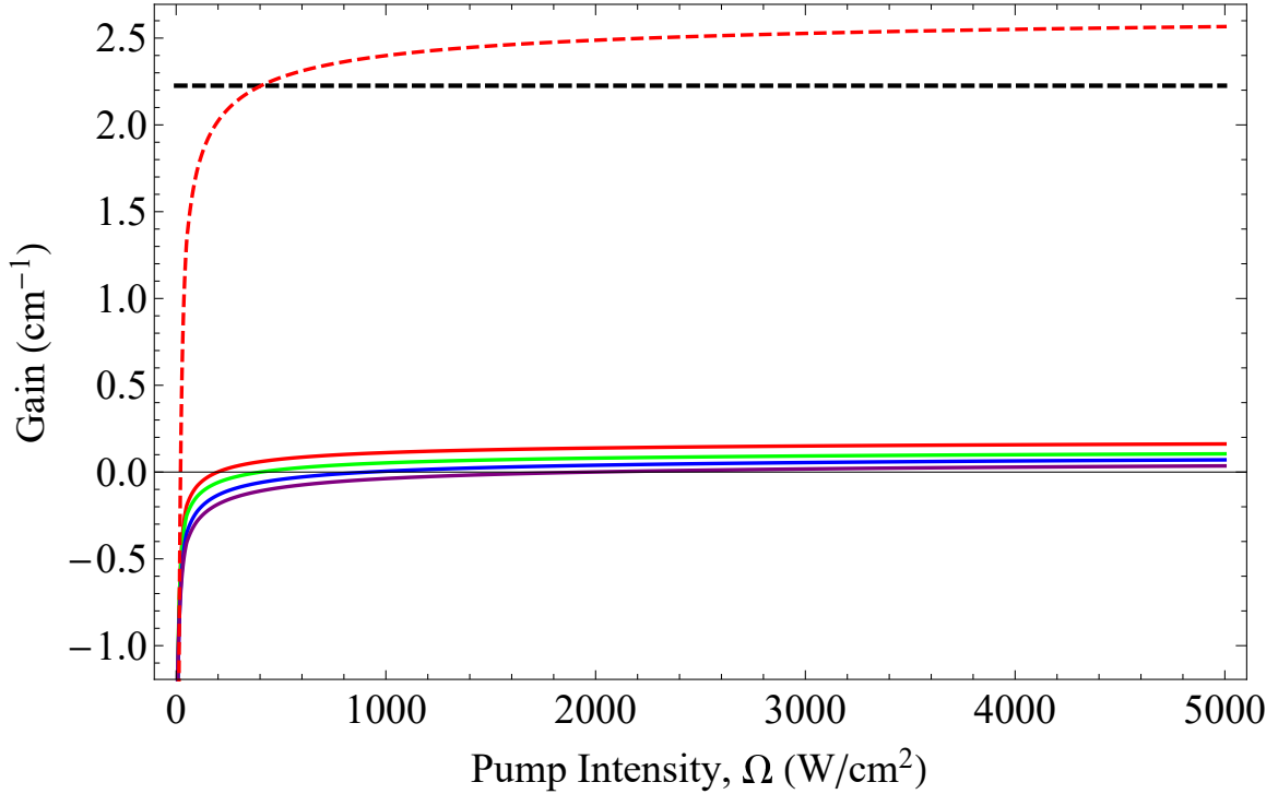
Figure 34. Predicted gain at 100 (red), 200 (green), 300 (blue), and 400 (purple) Torr as a function of the longitudinally averaged pump intensity for a 254 \mu\text{m} thick dielectric and 100 \mu\text{m} hole diameter plate. The corresponding measured Ar 1s_5 number densities were 0.87 \times 10^{13} , 1.07 \times 10^{13} , 1.28 \times 10^{13} , and 1.33 \times 10^{13} \text{ cm}^{-3} . Threshold is marked by the black dashed line. The red dashed line shows what the gain to reach threshold, which would require a number density of 7 \times 10^{13} \text{ cm}^{-3} at 100 Torr.
