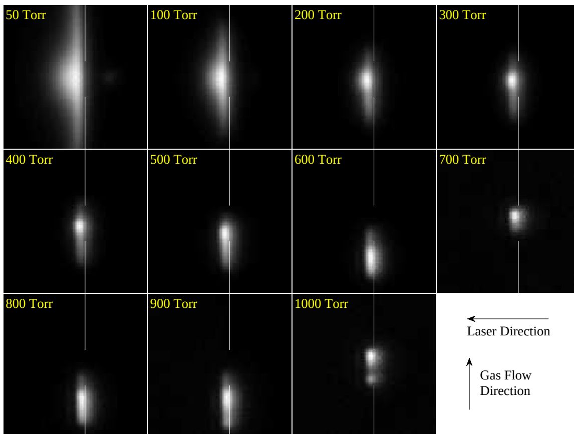
Figure 53. Side florescence from a 254\ \mu\text{m} thick dielectric and 300\ \mu\text{m} diameter hole. The approximate location of the left plate edge is shown with the white line, with the gap representing the hole location. At 50 and 100 Torr the plasma is symmetric and a slight bit of florescence can be seen on the opposite side of the plate (right of the white lines). At 200 Torr and above the plasma is asymmetric and forms in line with or below the hole.
