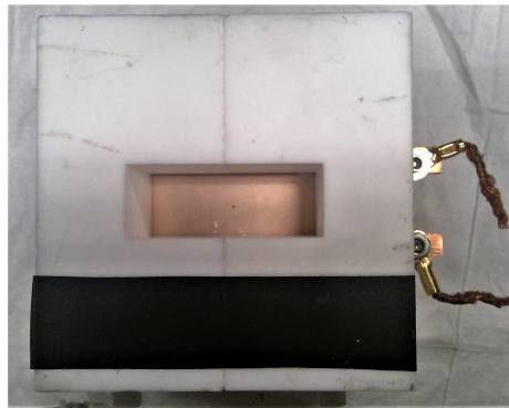
Figure 8. End on view of the assembled plate and mount. The black strip is electrical tape used to help hold the mount together while it was placed in the vacuum chamber.
