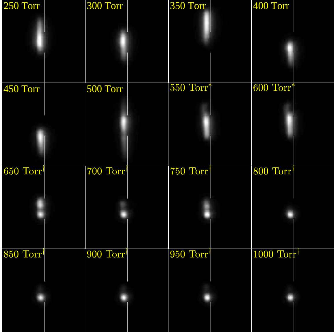
Figure 50. Side florescence from 127 \mu\text{m} thick dielectric and 300 \mu\text{m} hole diameter plates. The * (550 and 600 Torr) and † (650-1,000 Torr) indicate when different plates were used. The approximate location of the left plate edge is shown with the white line, with the gap representing the hole location. The plasma formation for each of the three plates used is slightly different. With the first plate (250-500 Torr) the plasma formation jumps up and down, the cause of which is unknown. With the second plate there is a small tail like structure on the upper side. With the third plate there are one or two smaller circular regions instead of one larger elongated region.
