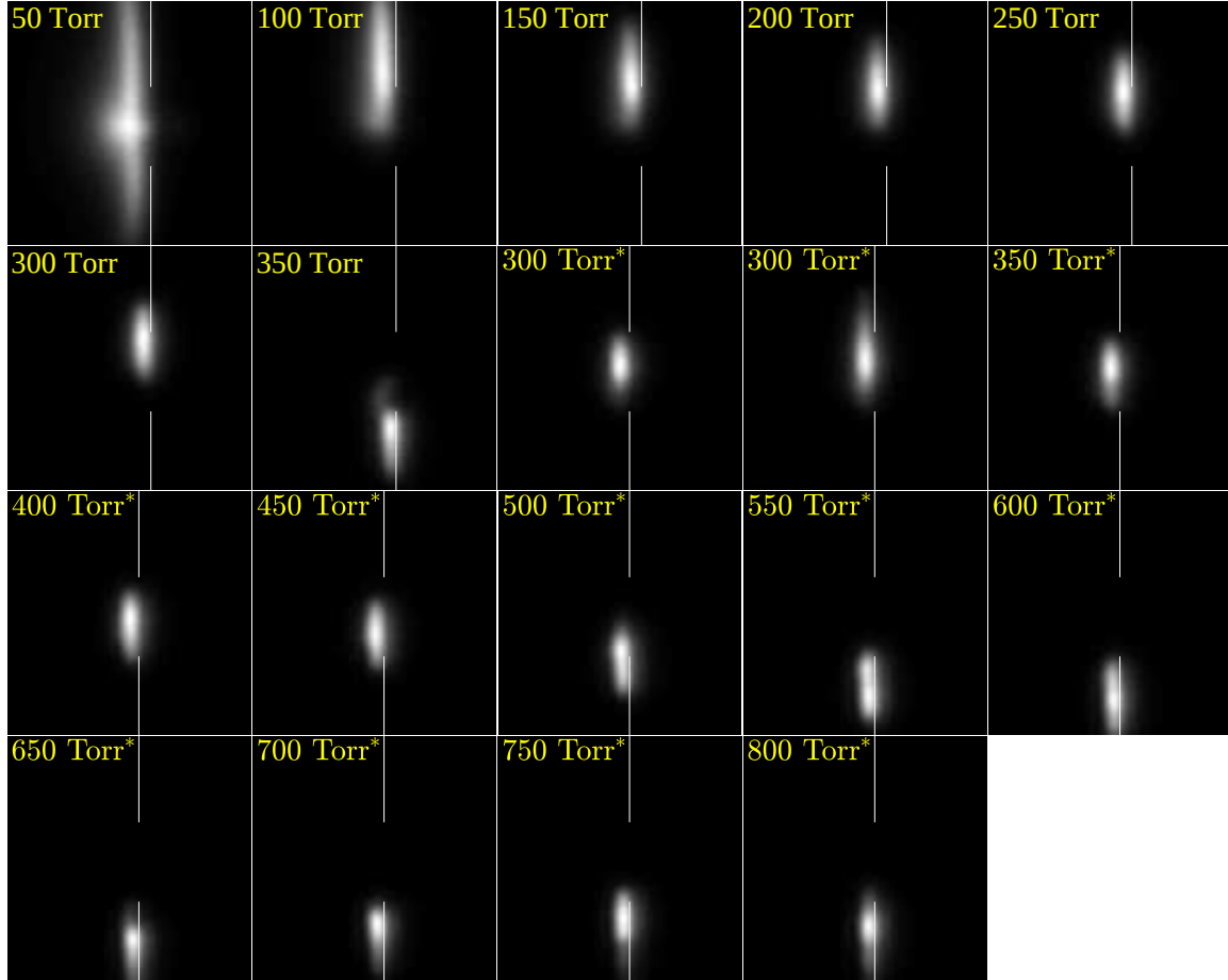
Figure 51. Side florescence from 127 \mu\text{m} thick dielectric and 400 \mu\text{m} hole plates. The * indicates when a different plate was used. The approximate location of the left plate edge is shown with the white line, with the gap representing the hole location. A symmetric plasma formation similar to the one at 50 Torr is desirable. With the first plate the plasma tended to form mostly above the hole, except for at 350 Torr where it was almost completely below it. With the second plate the plasma was initially centered on the hole and then moved below the hole. The difference in the plasma location is likely due to difference in the plate surface.
