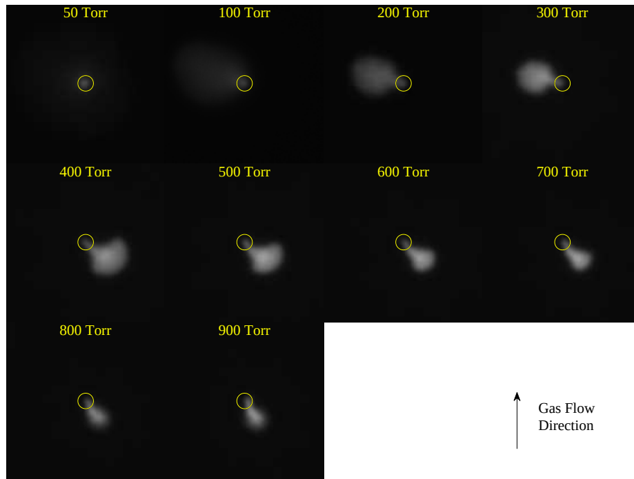
Figure 22. End-on images of a 127\ \mu\text{m} thick dielectric, 200\ \mu\text{m} diameter MHCD. The circle shows the approximate location of the hole. The plasma is symmetric at 50 Torr, but becomes asymmetric as pressure is increased. It is unknown what causes the location of the plasma to change, but could be a result of changes to the hole and plate during operation.
