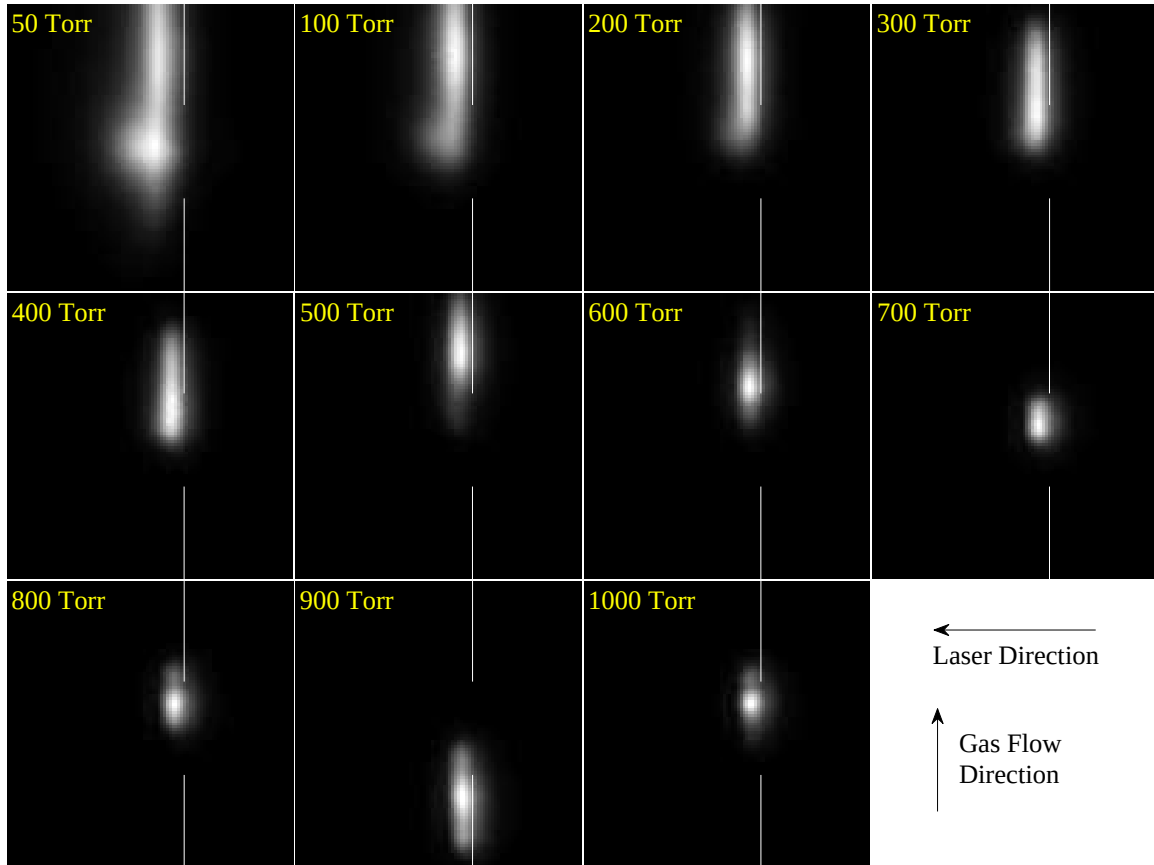
Figure 54. Side fluorescence from a 254\ \mu\text{m} thick dielectric and 400\ \mu\text{m} diameter hole. The approximate location of the left plate edge is shown with the white line, with the gap representing the hole location. The plasma formation is always asymmetric but its location varies. While it mostly forms near the upper edge of the hole and extends upward, at 500 and 900 Torr the plasma is mostly above and below the hole respectively. Excluding 900 Torr the plasma constricts to the upper hole region as the pressure increases. It is not known why the upper region of the hole was the favored location for this plate.
