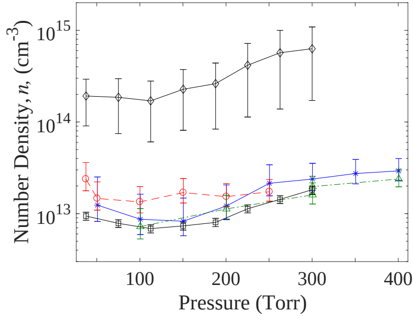
Figure 27. Calculated number density from a (*) 100 \mu\text{m} and (○) 200 \mu\text{m} diameter MHCD, both with a 127 \mu\text{m} thick dielectric and a (△) 300 \mu\text{m} hole, 254 \mu\text{m} thick dielectric MHCD. The data in black are the number densities determined by Penache et al. using a 50 \mu\text{m} thick dielectric and 300 \mu\text{m} hole diameter [28, 29].
