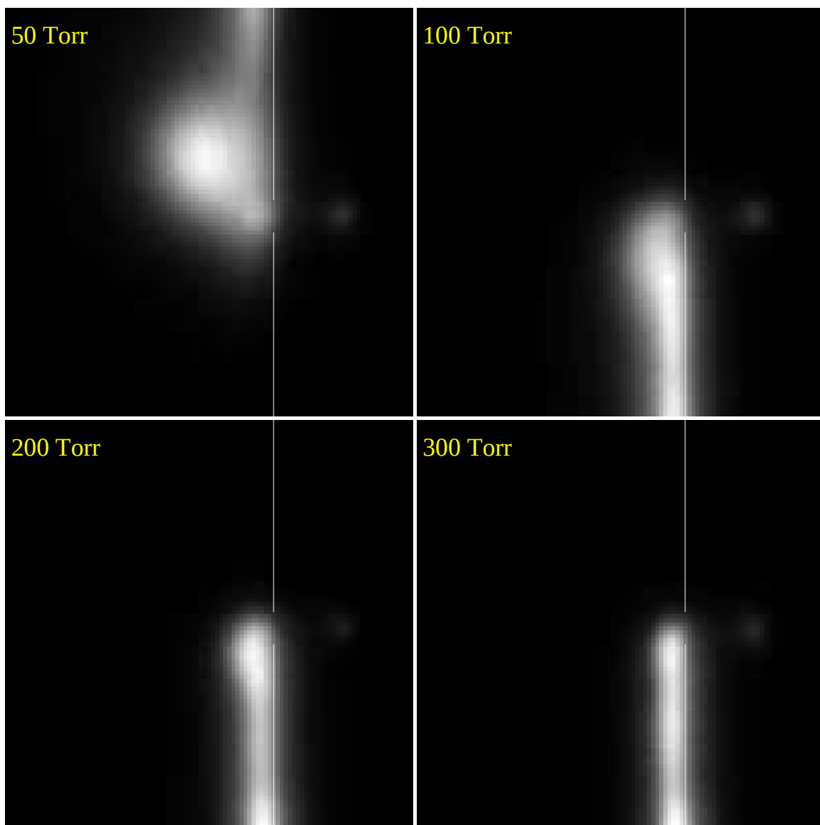
Figure 52. Side fluorescence from a 254\ \mu\text{m} thick dielectric and 100\ \mu\text{m} diameter hole. The approximate location of the left plate edge is shown with the white line, with the gap representing the hole location. There is a small circular fluorescence spot on the right in each image and is the fluorescence on the right side of the plate (the right edge of the plate is not marked). The plasma extends along the plate surface up away from the hole at 50 Torr, and down from the hole at 100-300 Torr. It is not known why there is a change in direction.
