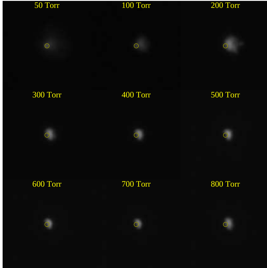
Figure 55. End-on images of a 127\ \mu\text{m} thick dielectric, 100\ \mu\text{m} diameter MHCD. The circle shows the approximate location of the hole. The gas flow is from the bottom to the top. At 50 Torr there is a slight asymmetry, which becomes more prominent as the pressure increases. It is unknown what caused the asymmetry, but it could be the hole structure or defects in the plate surface.
