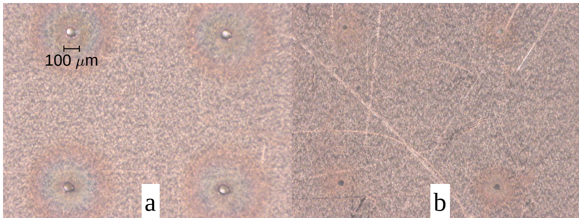
Figure 37. Images of both sides of a 50\ \mu\text{m} array before use. Image (a) is the side where the laser drilling occurred. The discoloration around the plates indicates heating during the drilling process. The lines in the images are scratches in the copper. The plate was flipped so that the holes on the left of image (b) are the back of the holes on the right of image (a). Despite the same laser drilling settings, the burn marks and hole shapes are noticeably different.
