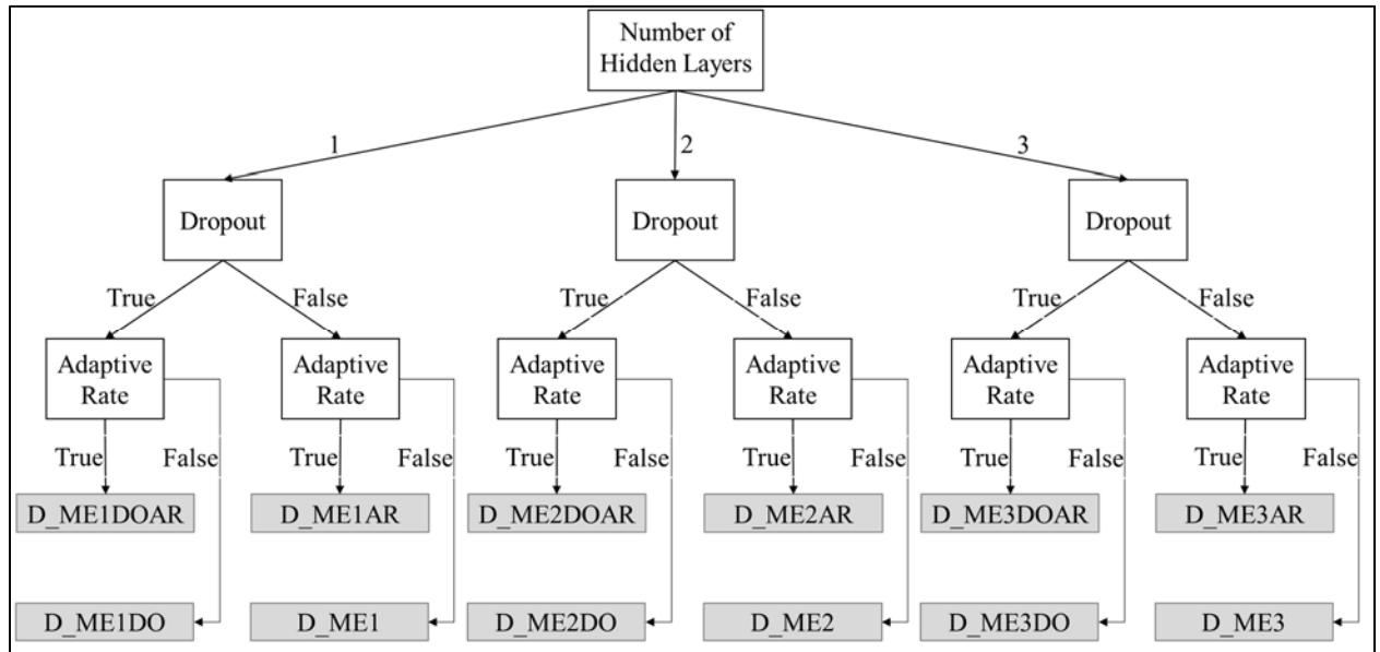
Figure 16. Hyperparameter Dependencies
