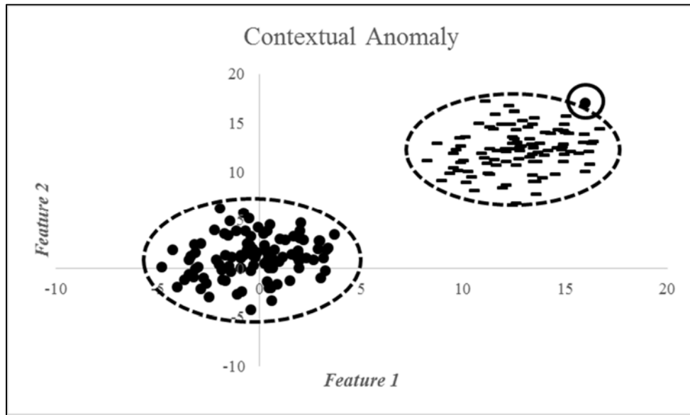
Figure 2. Contextual Anomaly
