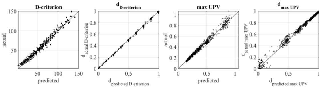
Figure 33. Actual by Predicted Design Performance
