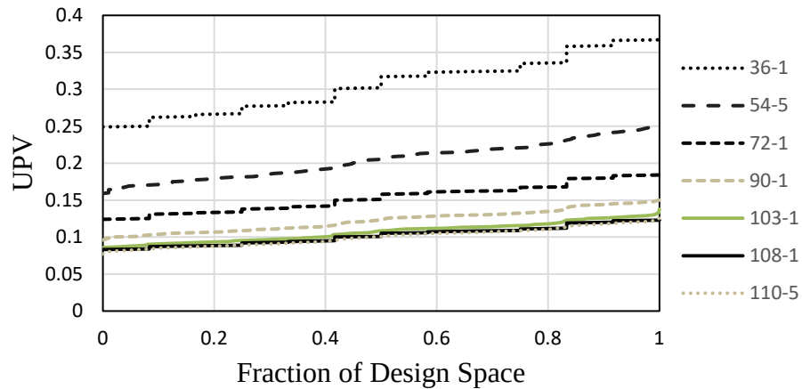
Figure 12. Fraction of Design Space (FDS) Plot for UPV
