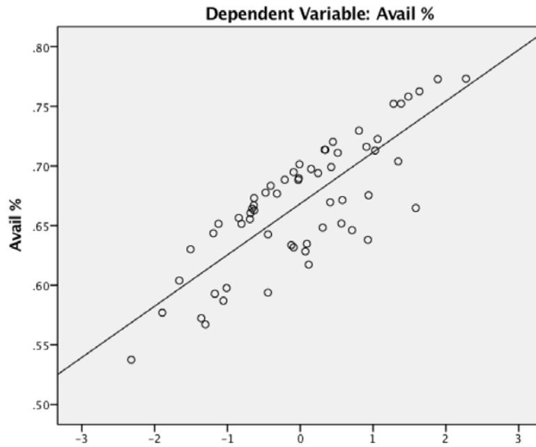
Figure 10. Kadena AB AA regression residuals scatterplot
