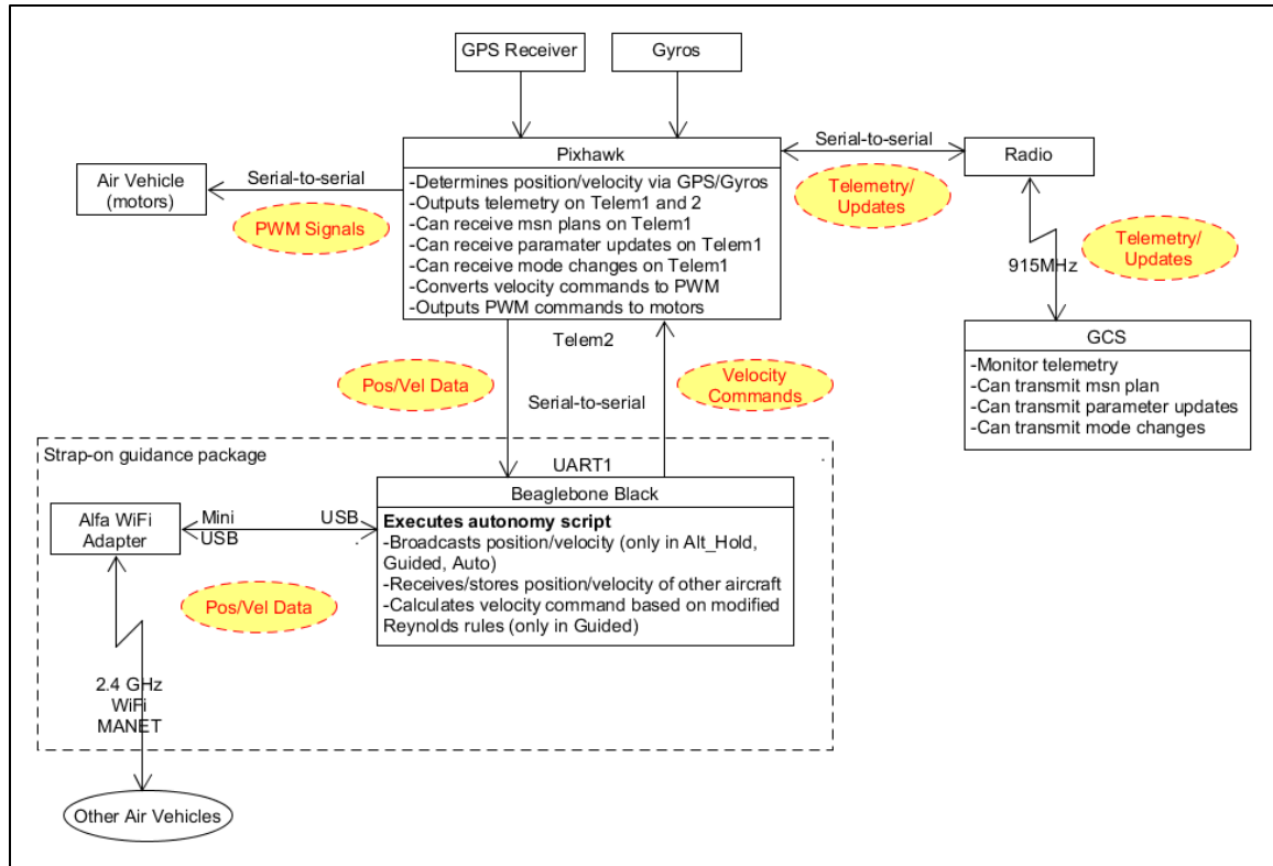
Figure 16. Block Diagram
