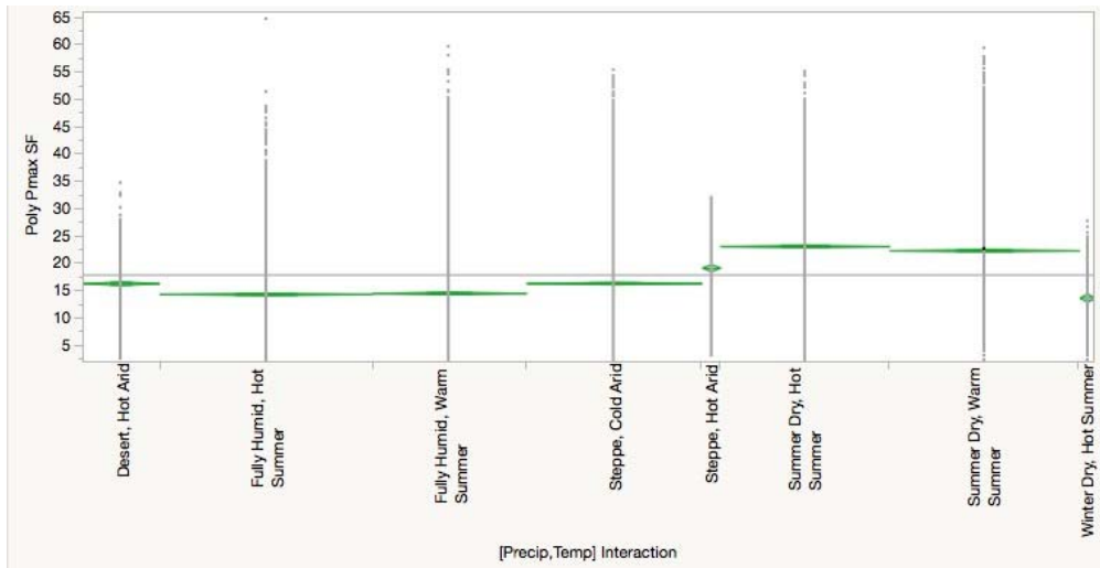
Figure 4.4: Poly - Precipitation/Temperature Interactions
