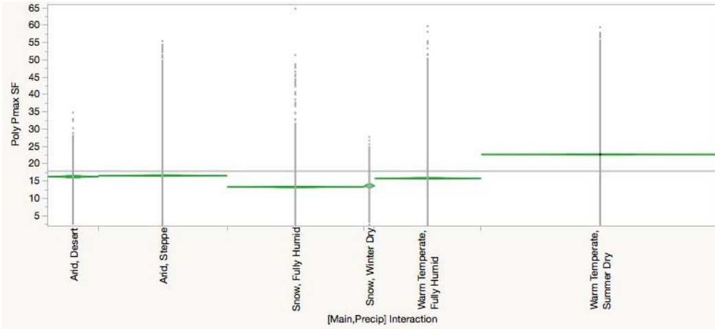
Figure 4.3: Poly - Main/Precipitation Interactions
