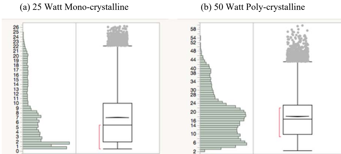
Figure 4.1: Data Distribution Box Plots
