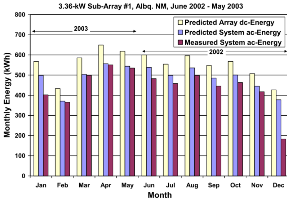
Figure 2.4: PV Model Annual Performance - Actual vs Predicted [25]
