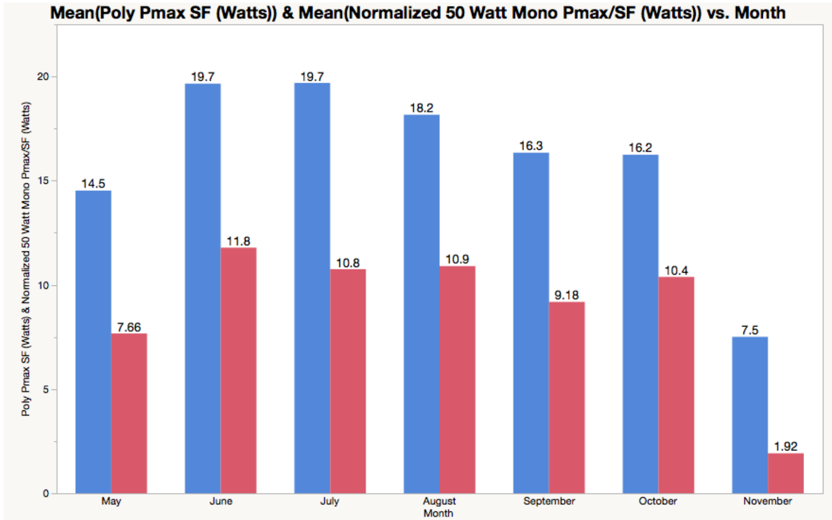
Figure 4.2: Normalized Monthly 50 Watt Power Averages - Monocrystalline vs. Polycrystalline
