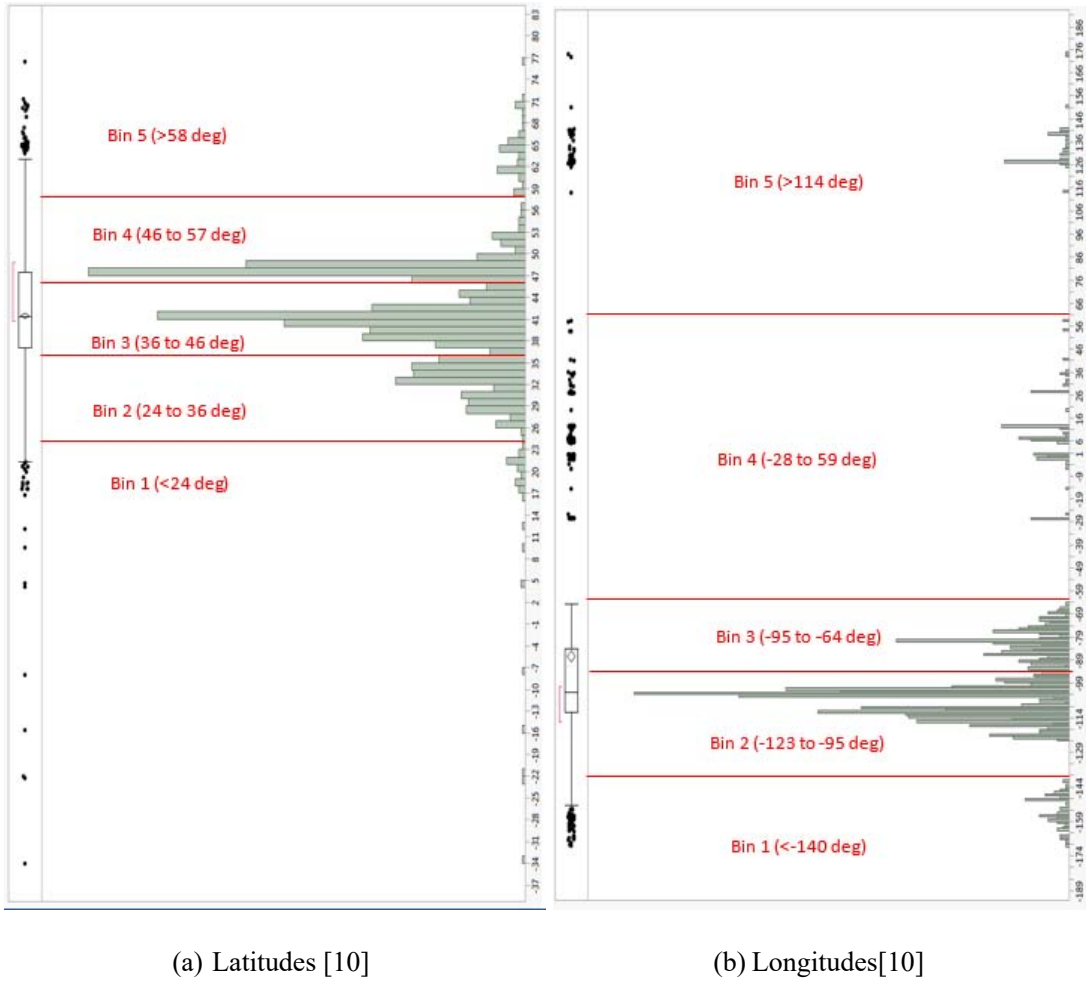
Figure 3.4: Histogram Breakdown of Air Force Installation Coordinates
