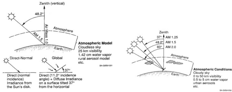
(a) Air Mass Spectrum [42]
