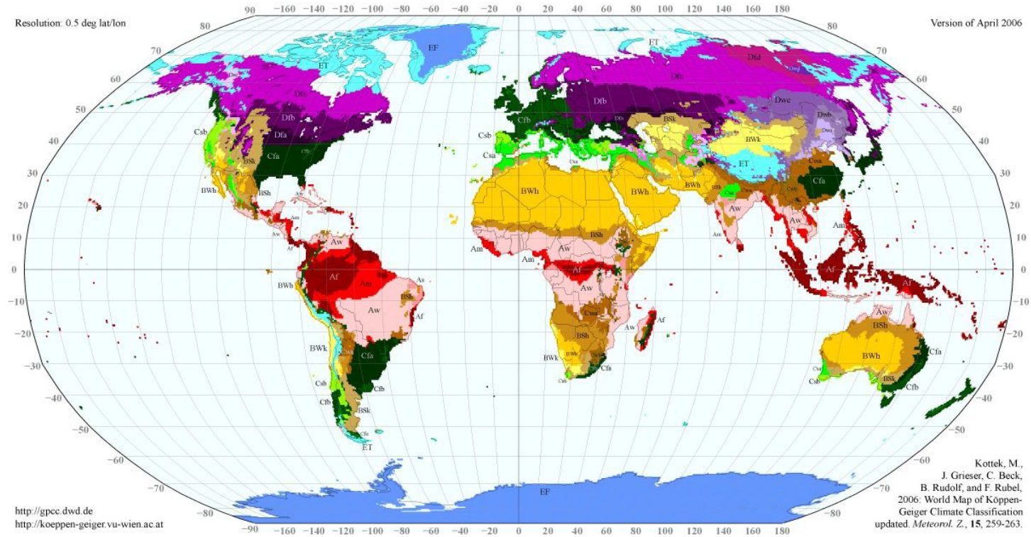
Figure 2.10: Köppen-Geiger Climate Classification World Map [28]
