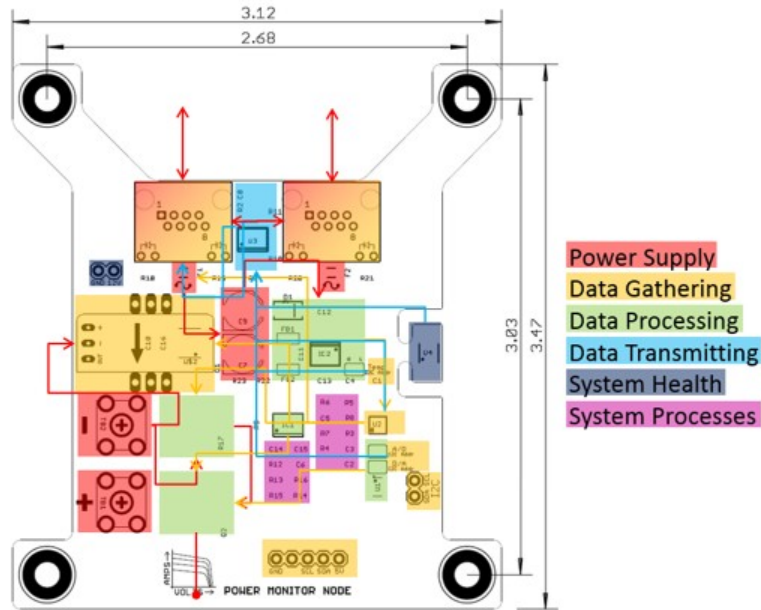
Figure 3.1: Node Chip Diagram [10]
