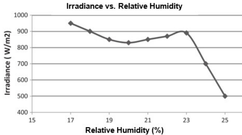
Figure 2.7: Irradiance vs. Humidity Data [34]
