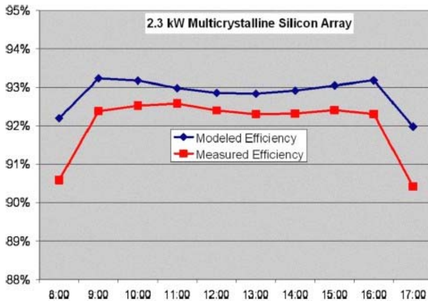
Figure 2.5: PV Model Efficiency Study - DOE [26]
