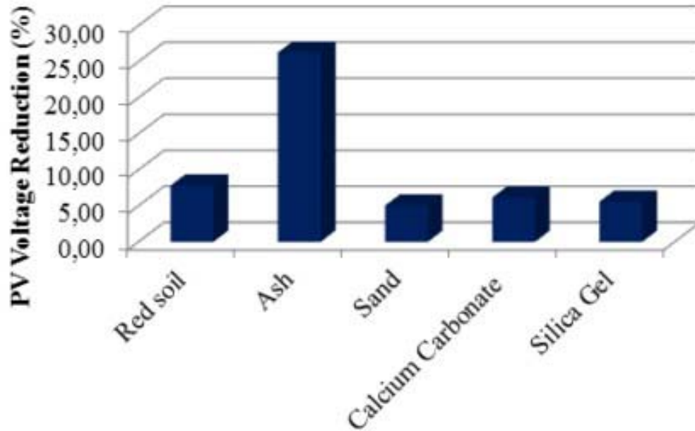
Figure 2.9: Dust Effects on Production [24]
