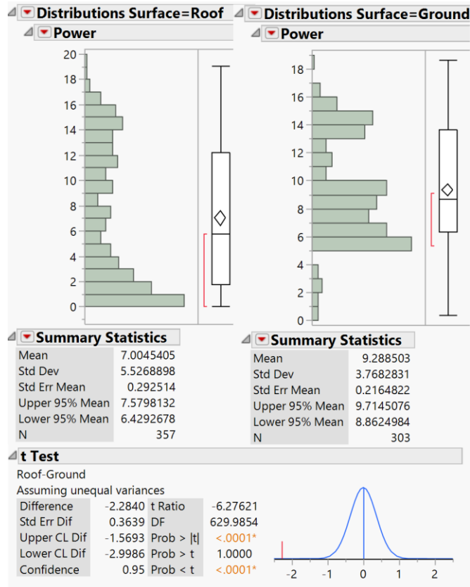
Figure 30. two-sample t-test comparing ground and roof system output
