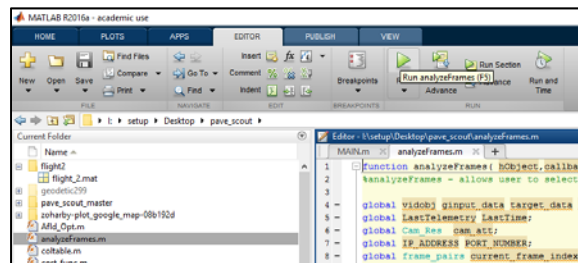
Figure 27. Step 5. - Loading & Running analyzeFrames.m
