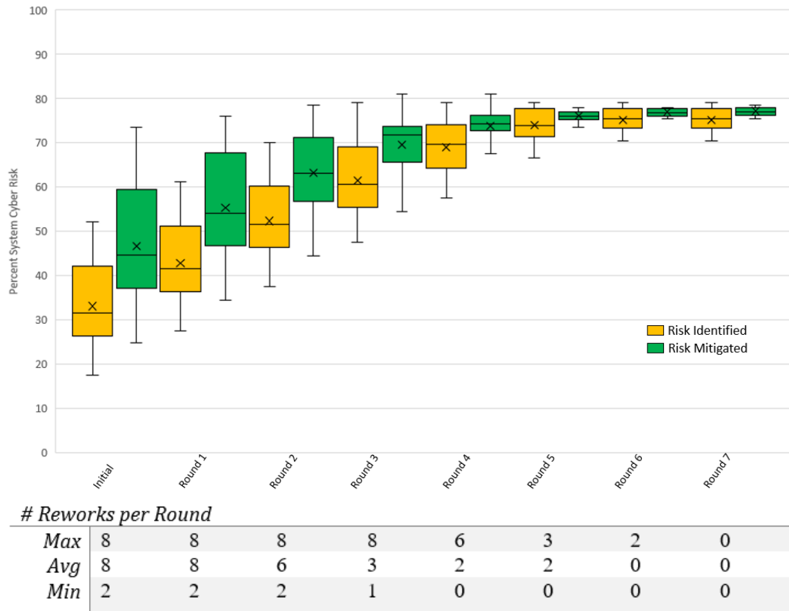
Figure 9. Validation Risk Identification/Mitigation vs Reworks
