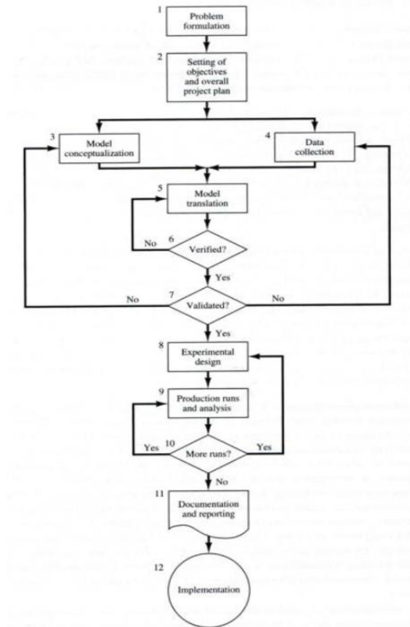
Figure 4. Steps in a Simulation Study [27]
