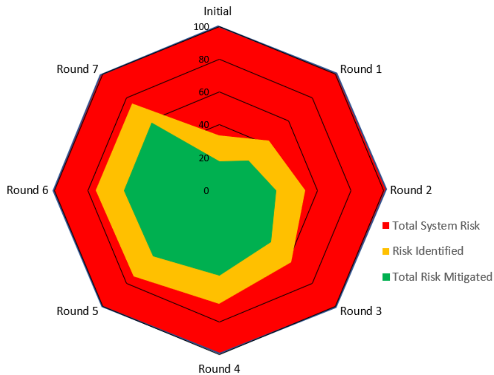
Figure 11. Baseline Radar Risk Identified and Total Risk Mitigated
