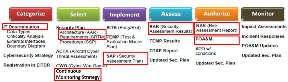
Figure 3. PIT A&A Process Deliverables [25]
