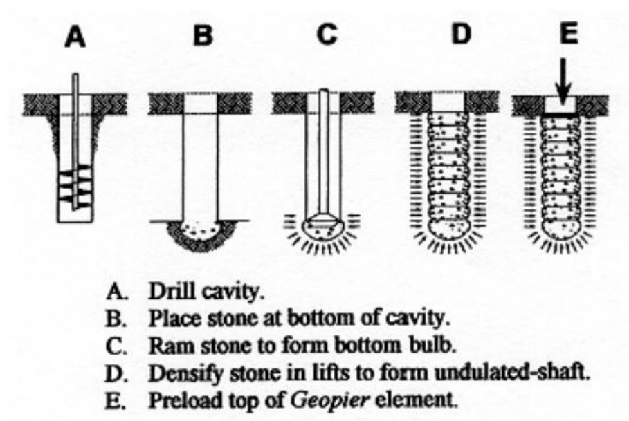
Figure 5. Geopier Condensed Installation Guide (American Society of Professional Estimators, 2010)
