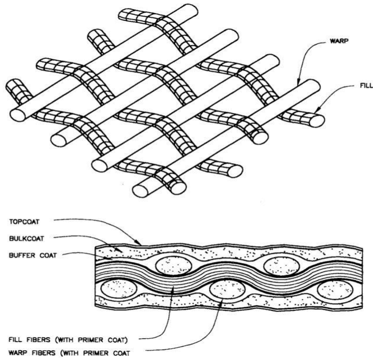
Figure 1. Top image shows scrim with woven yarns of the warp and fill directions. Bottom image shows a typical cross section of a tensile fabric with the arrangement of coatings and scrim ( C. G. Huntington ).
