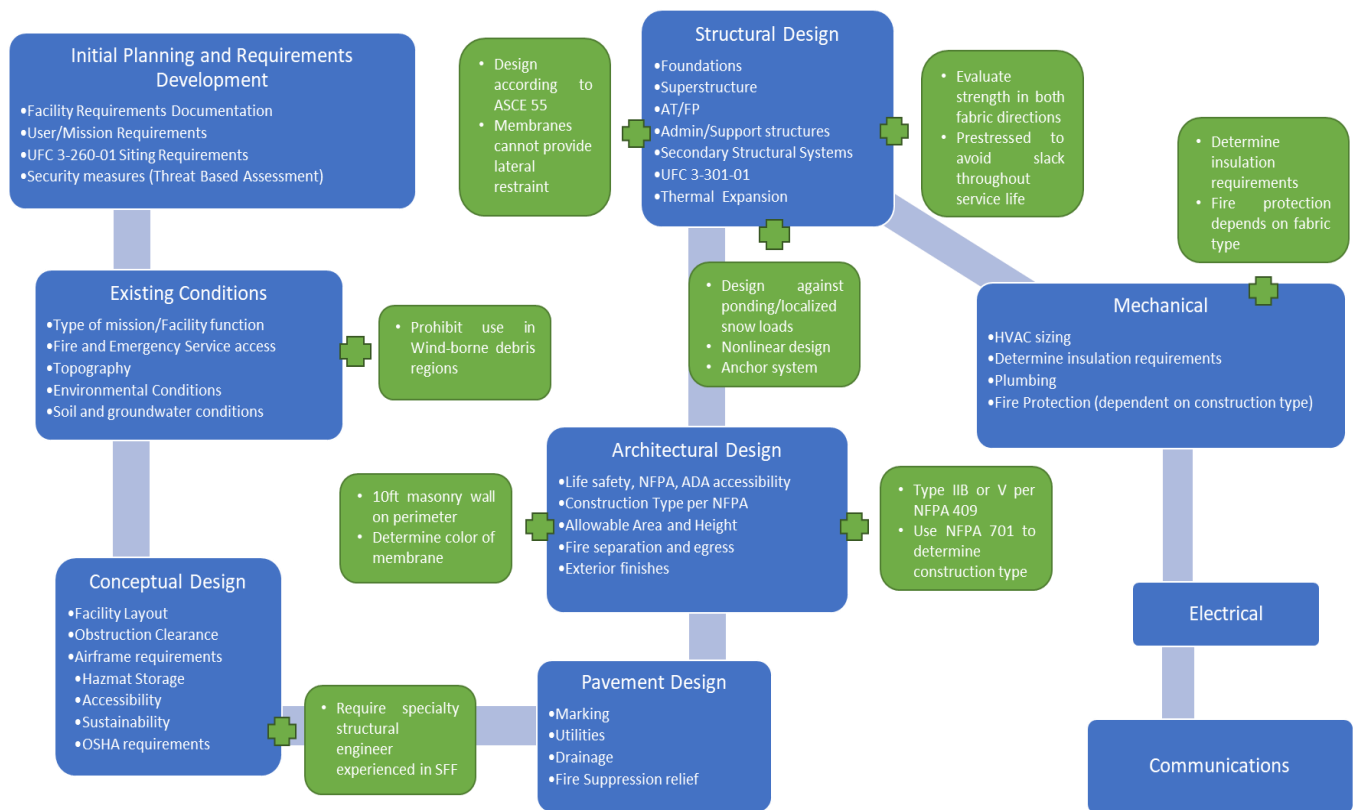
Figure 20. UFC 4-211-01 design process including recommendation for steel framed fabric hangars.
