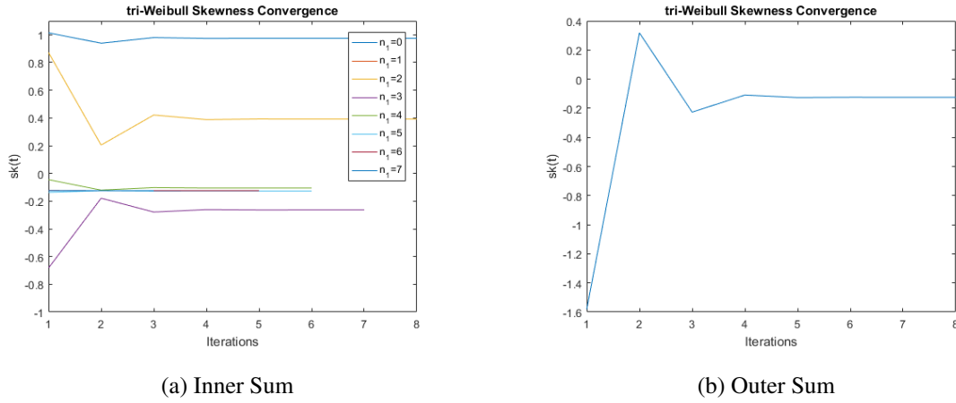
Figure 4.6: Convergence of tri-Weibull Inner & Outer Sum Skewness
