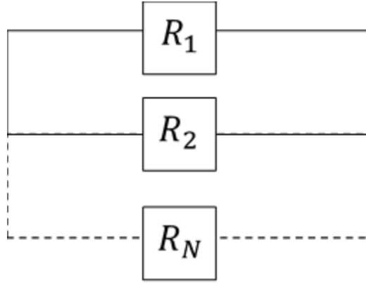
Figure 1.2: Parallel Example
