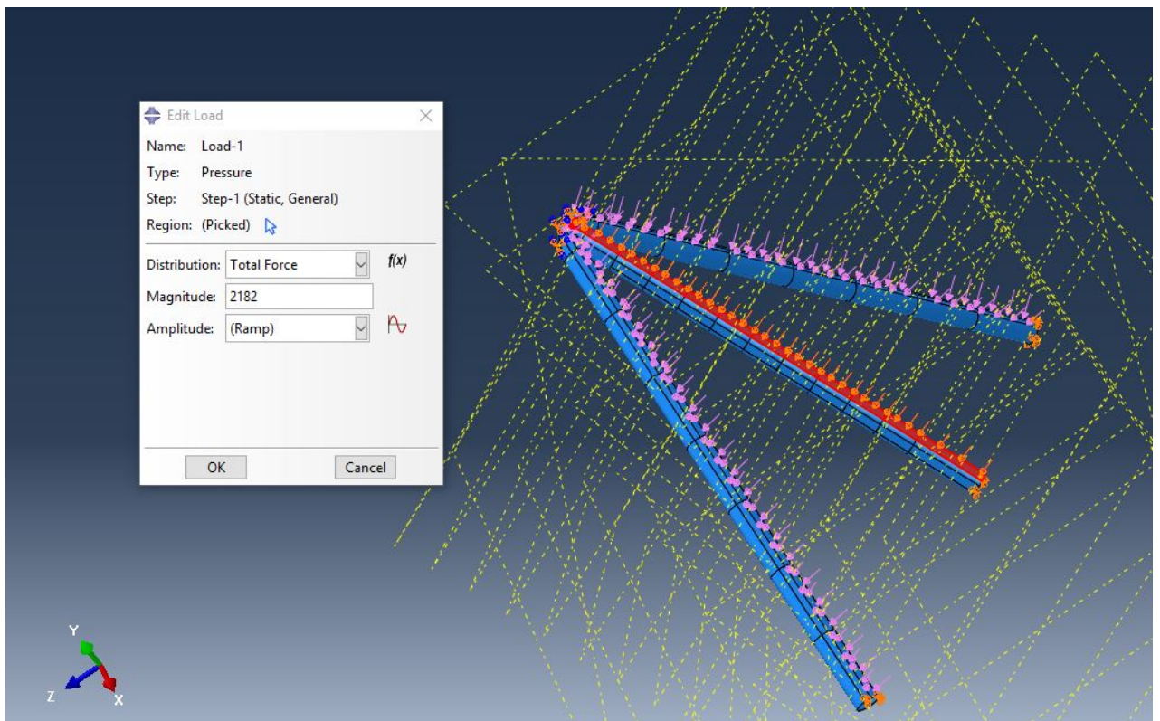
Figure C.4. Applying pressure load in 3D model with total force options in Abaqus CAE
