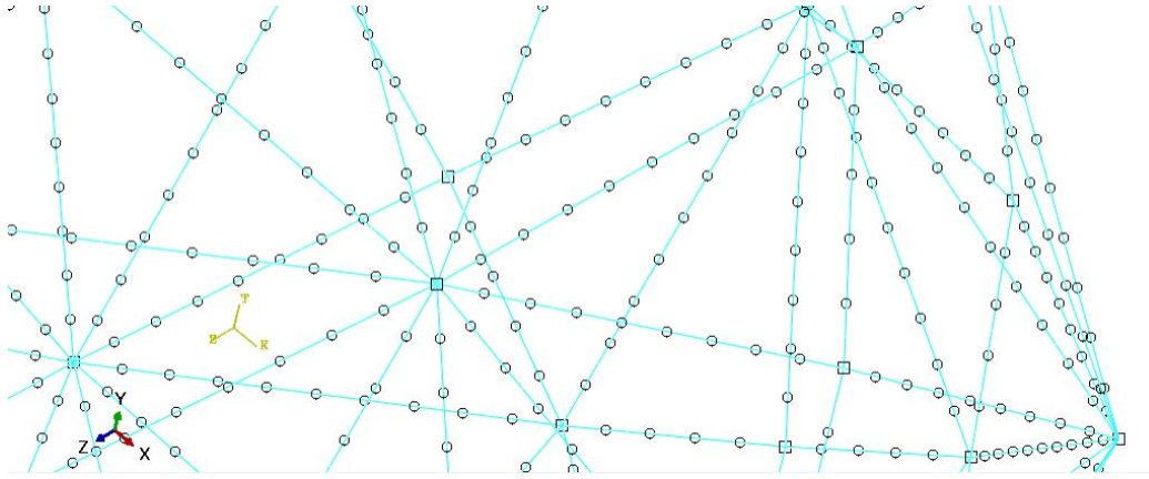
Figure 3.8. Hexakis Icosahedron frame mesh-1440 B32 beam elements - zoomed in
