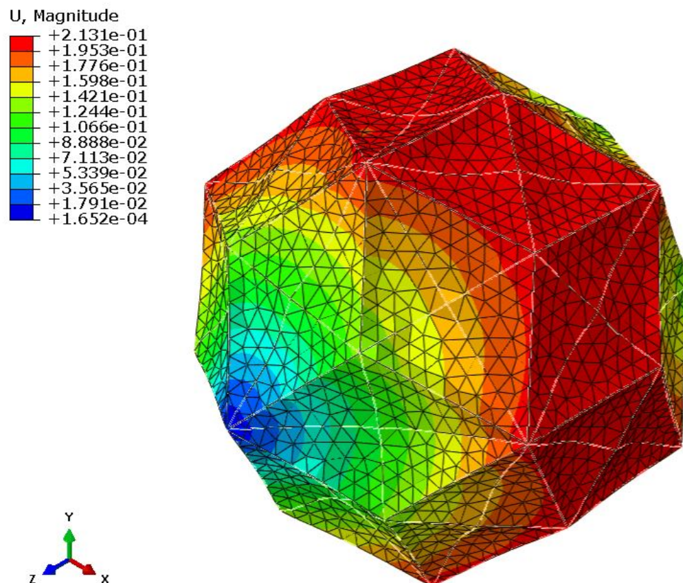
Figure 4.10. Model II ( \phi=0.3408 m, f/s, 1 mm beams, none), Deformation visualization of 0.3408 m hexakis icosahedron
