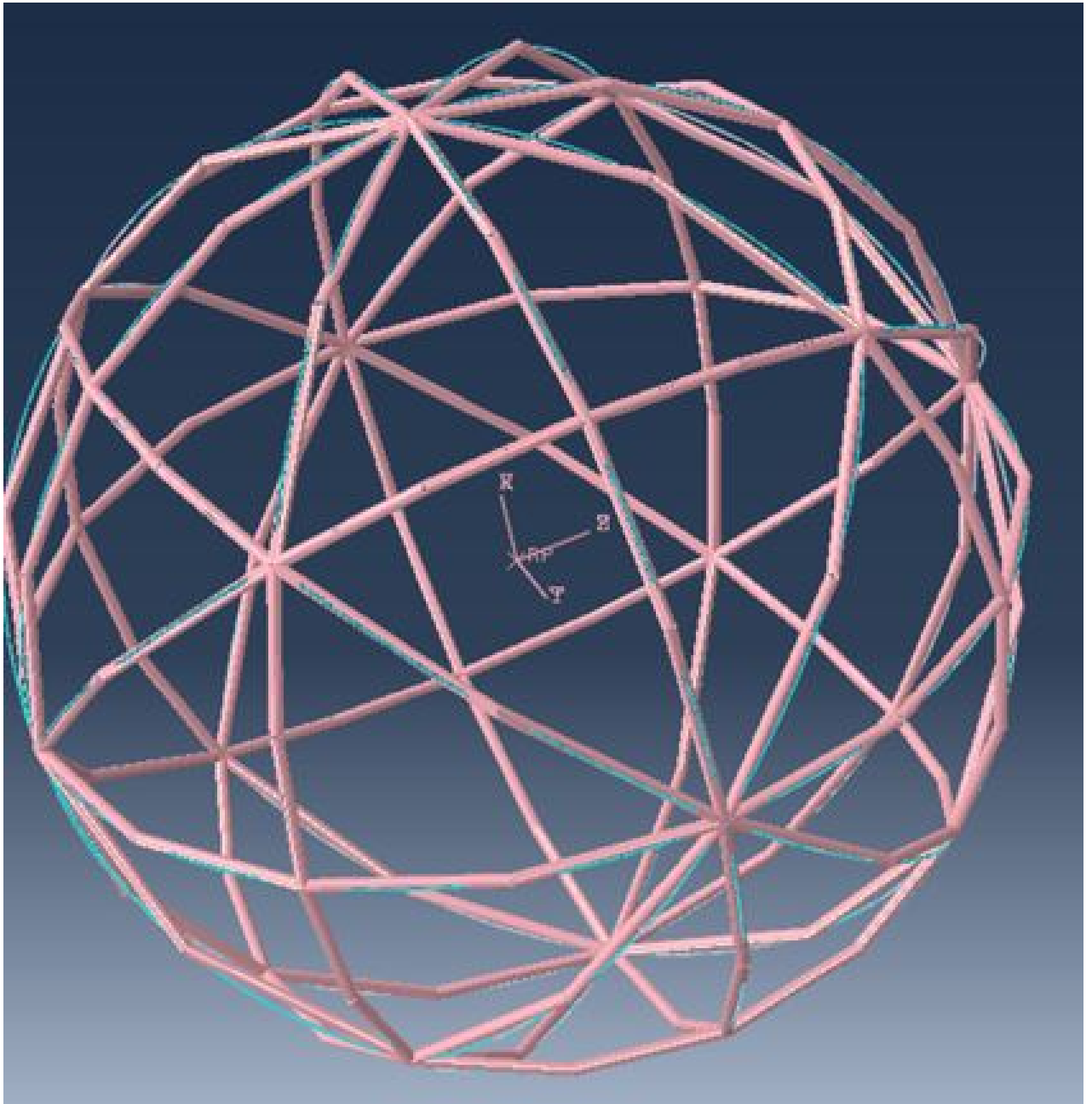
Figure 5.1. Celestial frame
