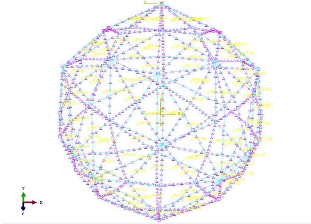
Figure 3.7. Hexakis Icosahedron frame mesh-1440 B32 beam elements
