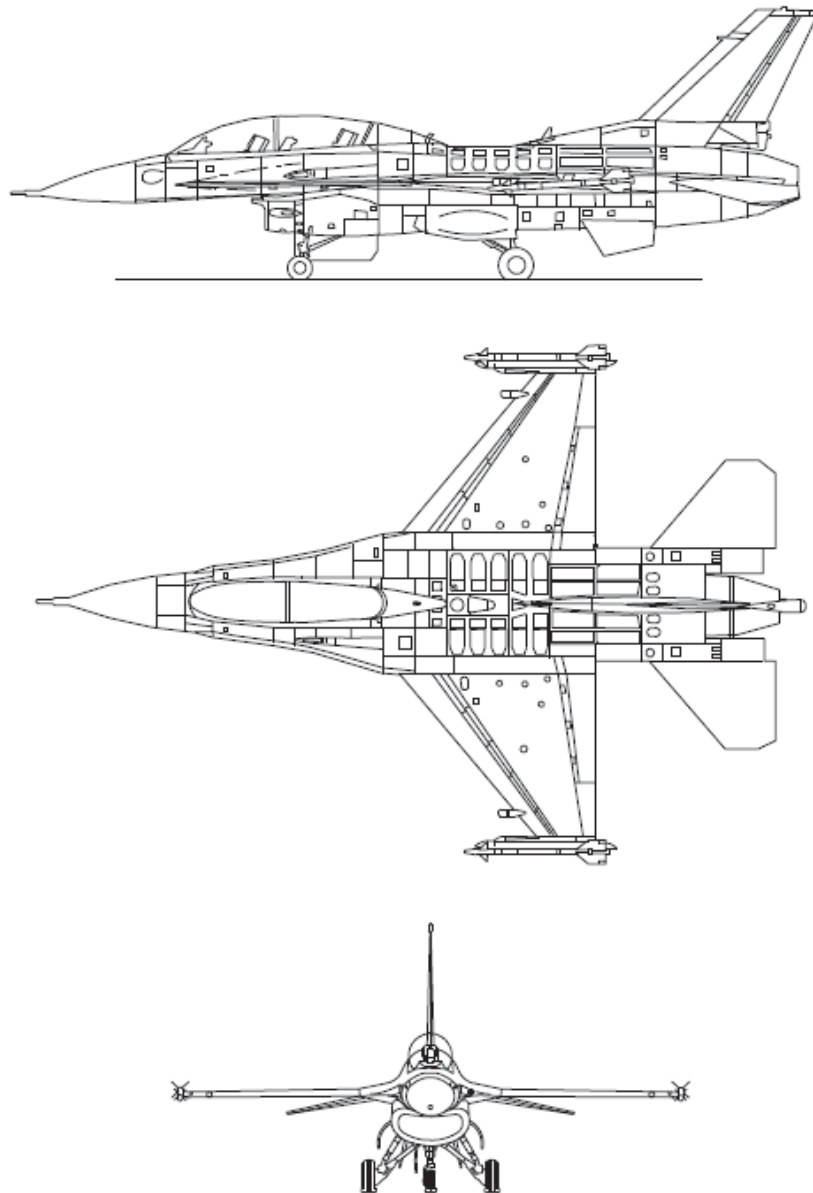
Figure 24: F-16DM 3-View
