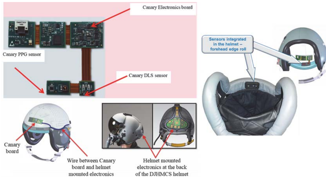
Figure 13: Elbit Layout
