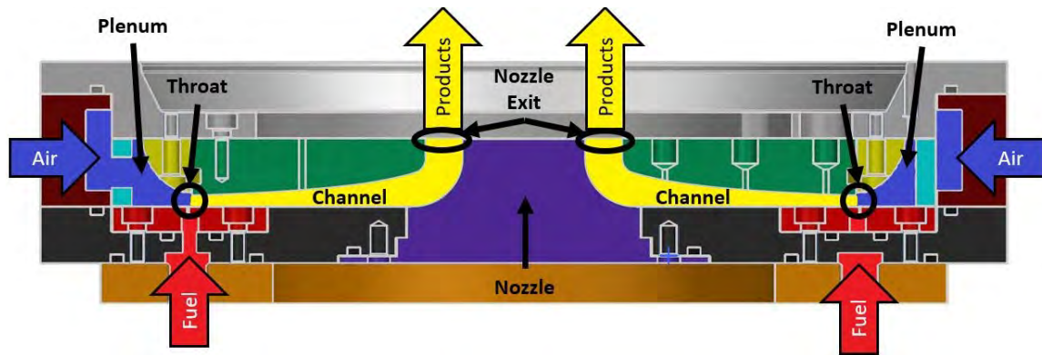
Figure 33. Cross Sectional Cut Away of the Final Radial RDE Design with Flowpath Highlighted.
