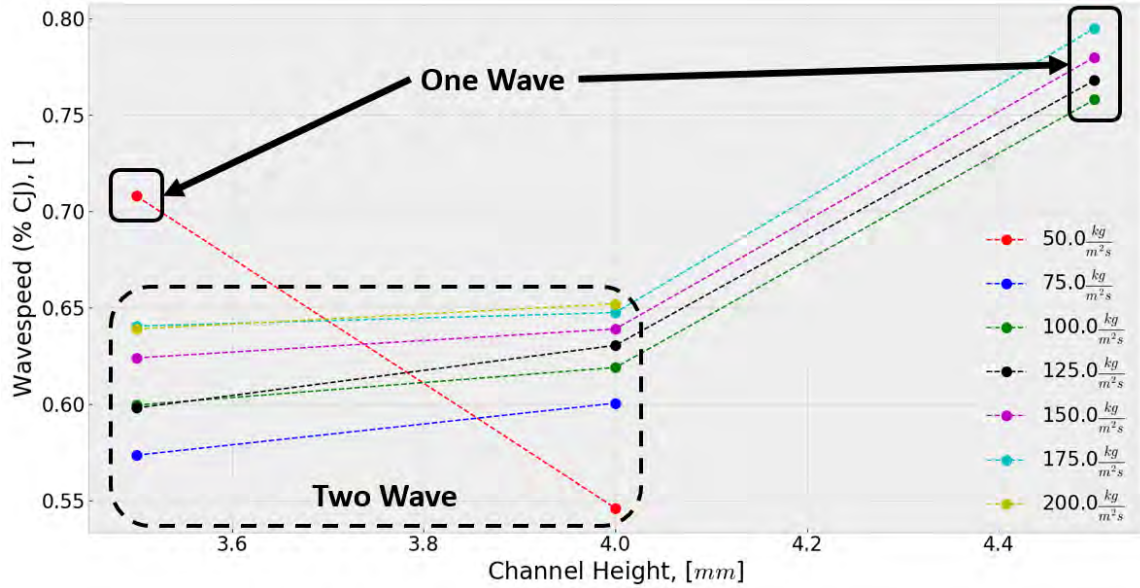
Figure 92. Wavespeed versus Channel Height: AR_t = 0.2 , AR_n = 1.0 , \phi = 0.7 .
