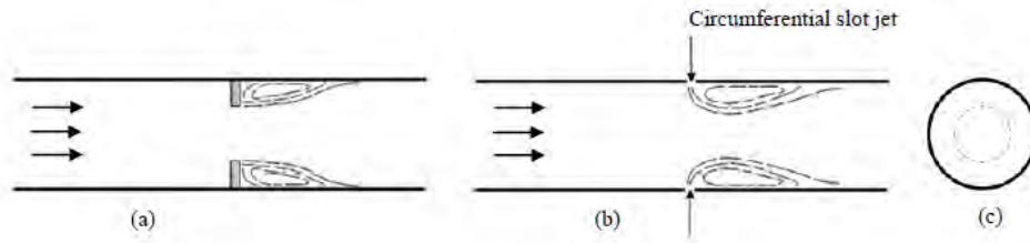
Figure 11. Conventional and Fluidic DDT Devices.[10]
