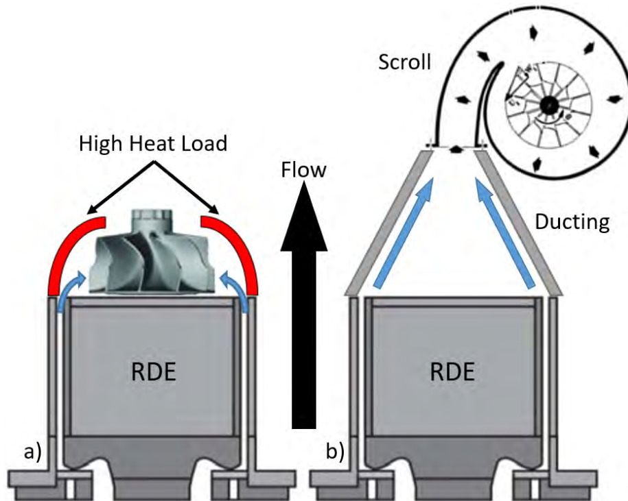
Figure 2. Conventional RDE with a Radial Inflow Turbine. (a) conventional RDE direct mount & (b) conventional RDE ducted mount
