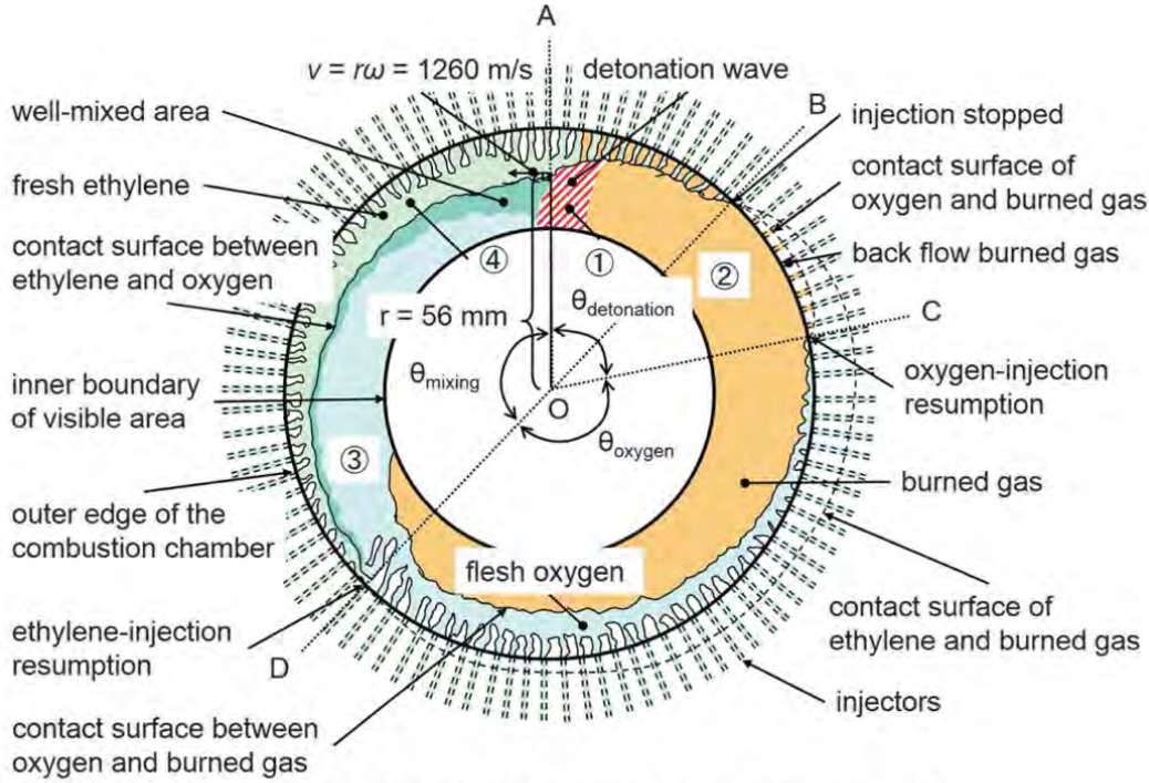
Fig. 5 Schematic of the phenomena in the disk-shaped RDC.
