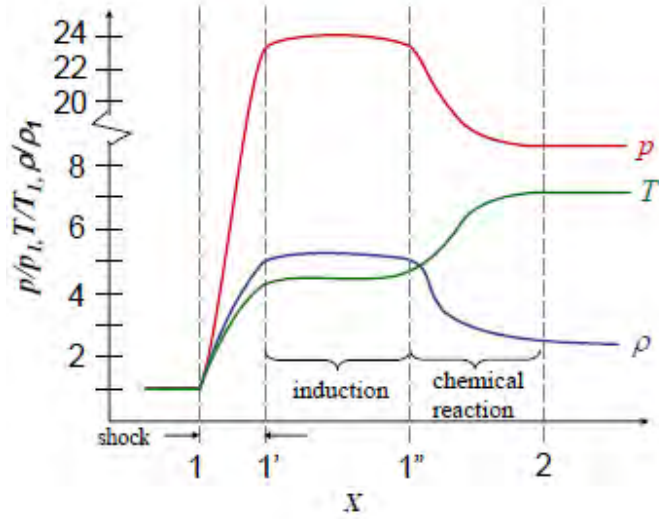
Figure 9. ZND Structure.[5]
