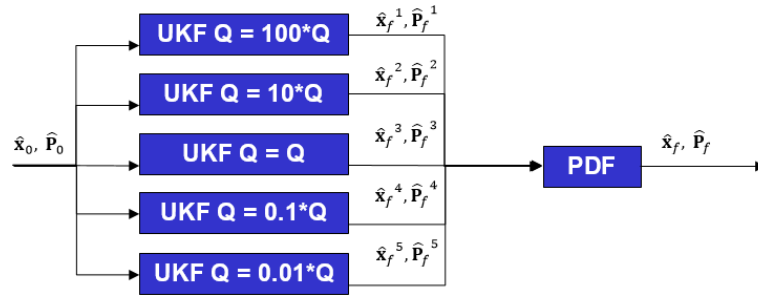
Figure 5. Visual diagram of the 1G IMM algorithm
