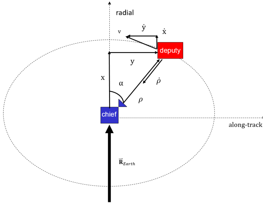
Figure 3. The LVLH reference frame
