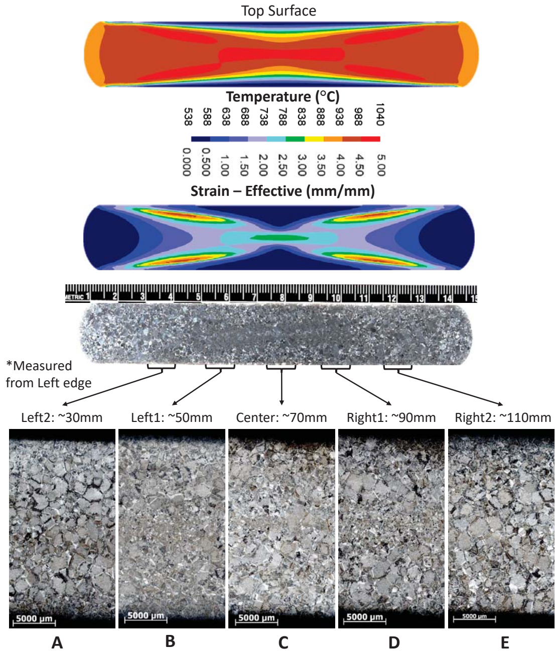
Figure 4.12. Sidepressing forging result at 955 °C initial furnace temperature, 25.4 \frac{\text{mm}}{\text{s}} ram speed, 65% reduction in height, and AFIT heat treatment. The macro scale image provides comparison between the predicted strain and temperature contour images. Each region of interest is labeled for closer grain size evaluation. This specimen appears to be developing coarse grains in the center and on the left and right edges with lobes of smaller grains in between. Scale bar: cm
