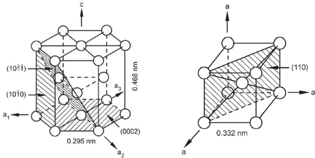
(a) Hexagonal Close-Packed (HCP)[1]
