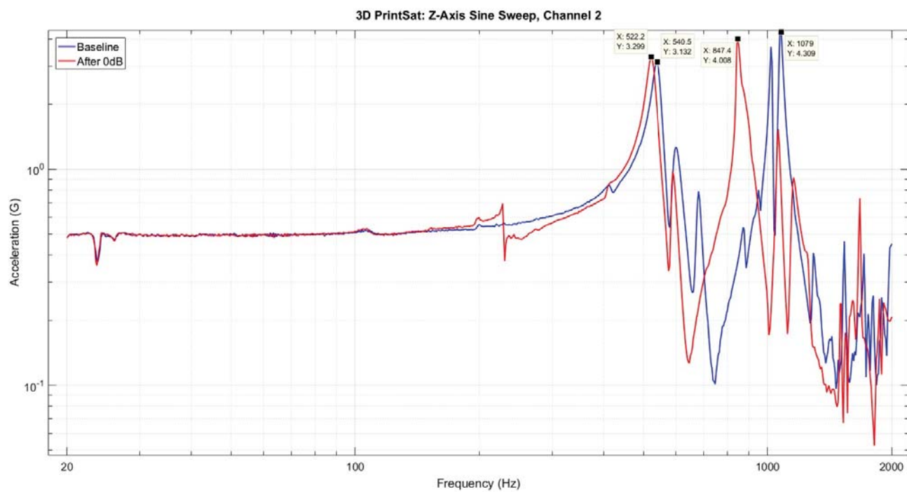
Figure 4.1: Z Axis Run 1 Accelerometer 1 Response
