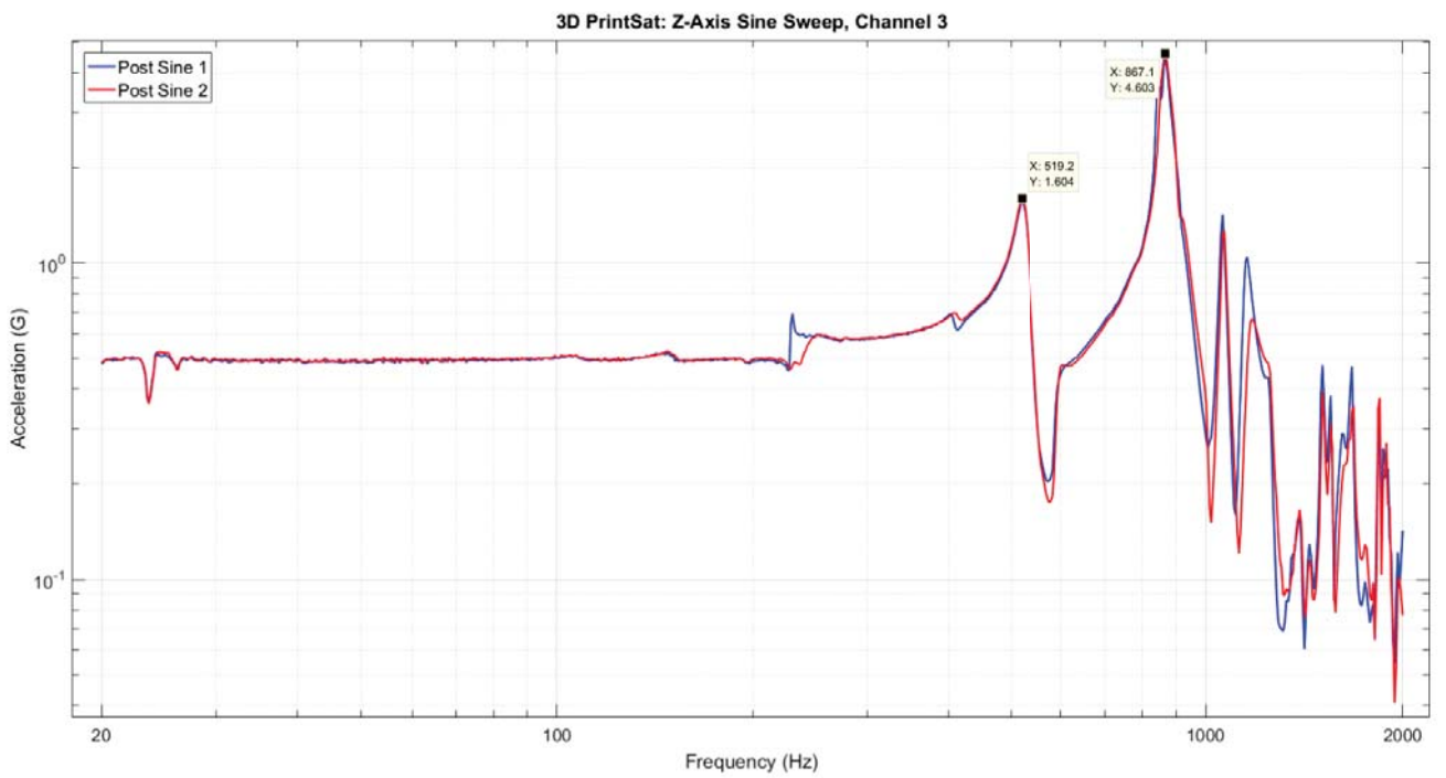
Figure 4.6: Z Axis Run 2 Accelerometer 2 Response
