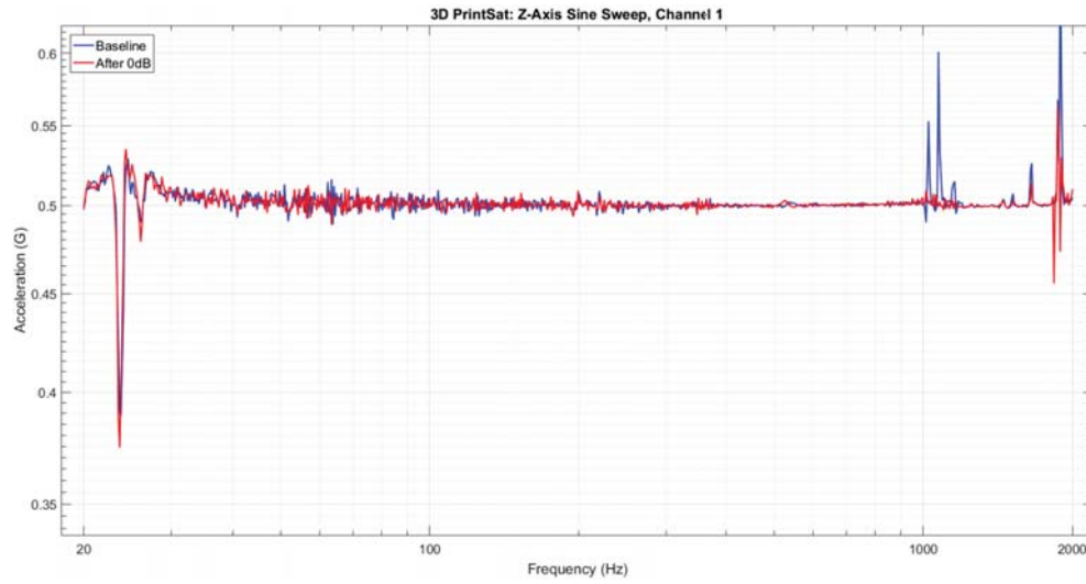
Figure D.1: Z Axis Run 1 Control Accelerometer Response
