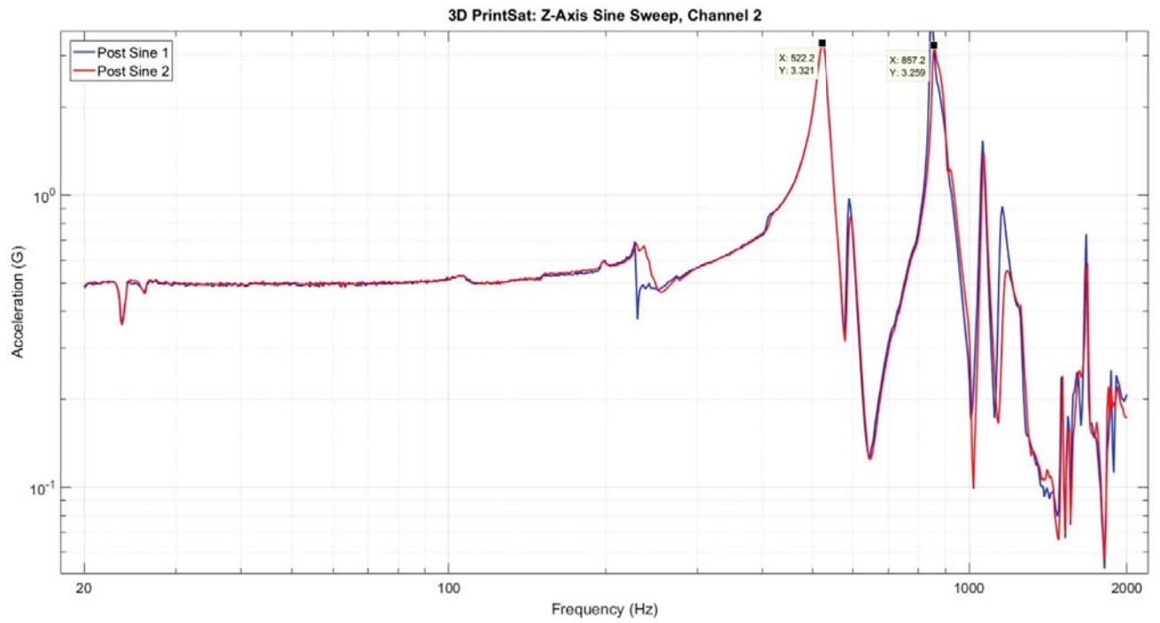
Figure 4.5: Z Axis Run 2 Accelerometer 1 Response
