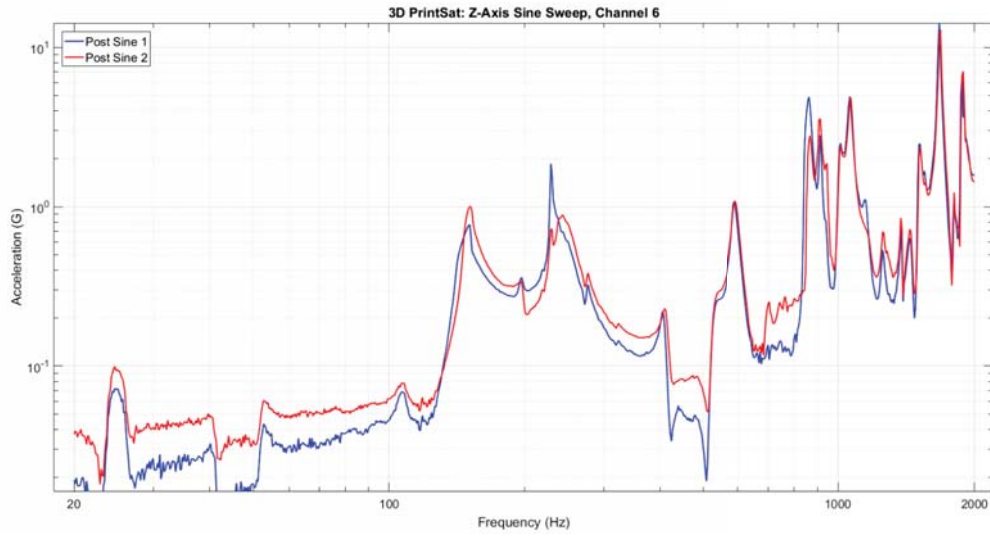
Figure D.9: Z Axis Run 2 Accelerometer 5 Response
