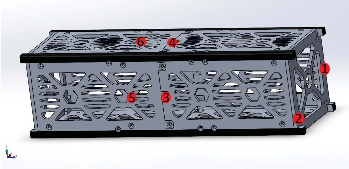
Figure 3.17: Accelerometer Locations
