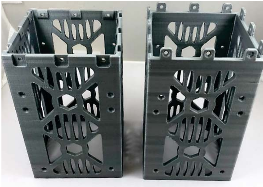
Figure 3.12: Male/Female Components
