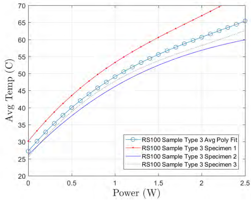
Figure B.33: The average of the three 3rd Order Polynomial curves plotted with the original fitted curves for RS100 Type 3 Specimens 1-3
