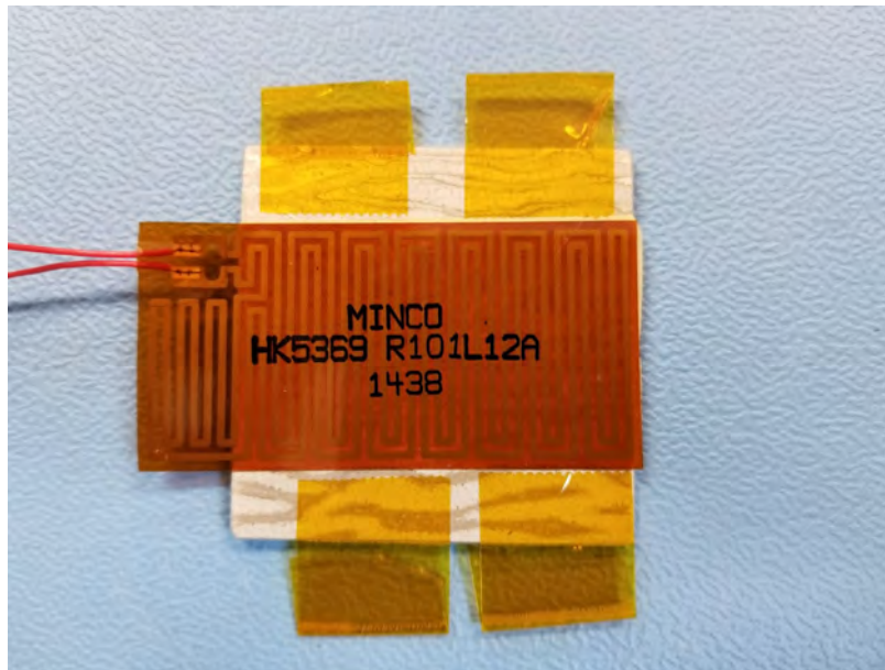
Figure 3.12: Etched foil heater with Kapton ® mounting tabs
