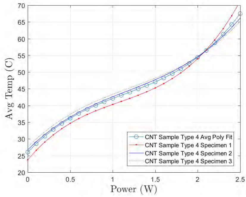
Figure B.34: The average of the three 3rd Order Polynomial curves plotted with the original fitted curves for CNT Type 4 Specimens 1-3
