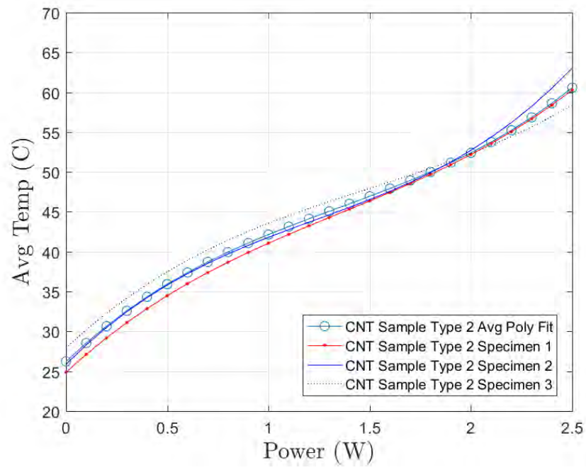
Figure B.32: The average of the three 3rd Order Polynomial curves plotted with the original fitted curves for CNT Type 2 Specimens 1-3
