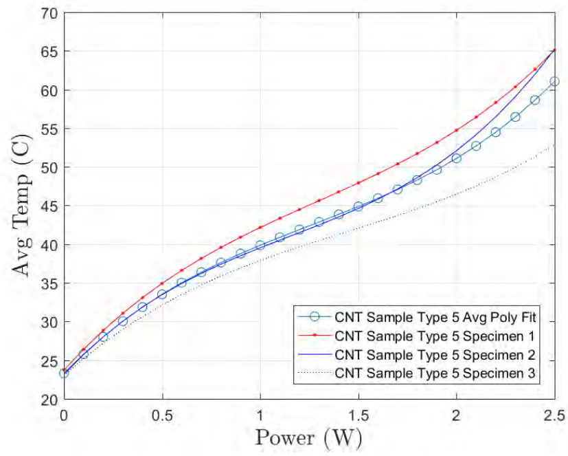
Figure B.35: The average of the three 3rd Order Polynomial curves plotted with the original fitted curves for CNT Type 5 Specimens 1-3
