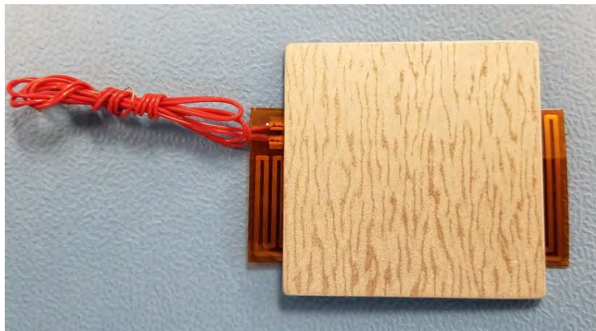
Figure 3.11: Minco TM heater specimen with bonded heat sink plate
