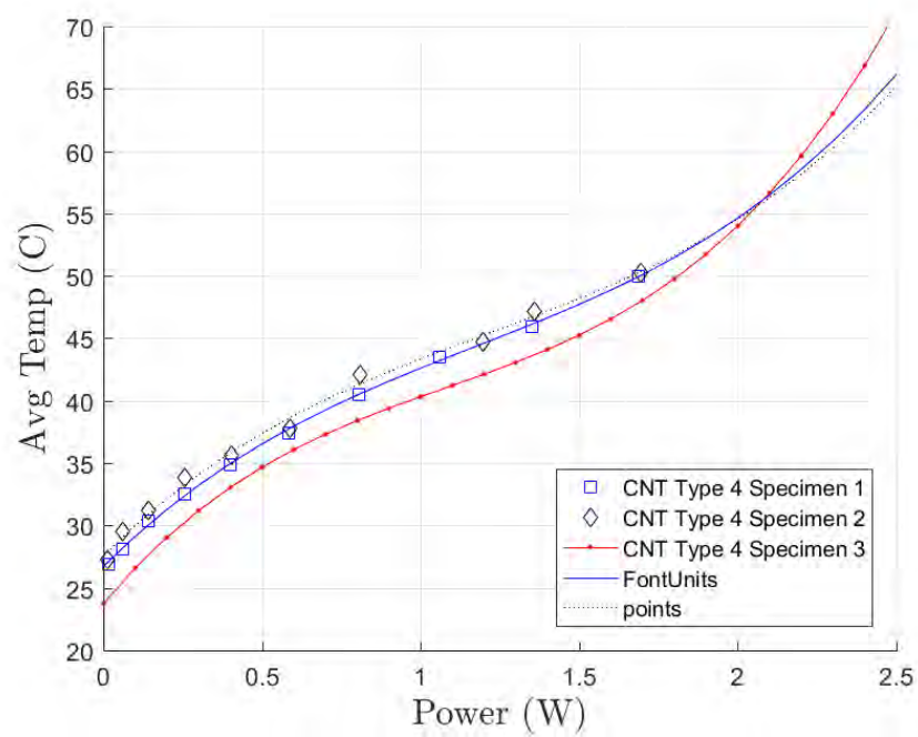
Figure B.28: This plot shows that a 3rd Order Polynomial curve fitted to the data accurately represents the known data points for Type 4 specimens
