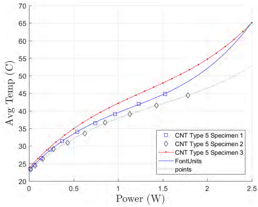
Figure B.29: This plot shows that a 3rd Order Polynomial curve fitted to the data accurately represents the known data points for Type 5 specimens
