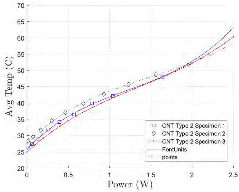
Figure B.26: This plot shows that a 3rd Order Polynomial curve fitted to the data accurately represents the known data points for Type 2 specimens
