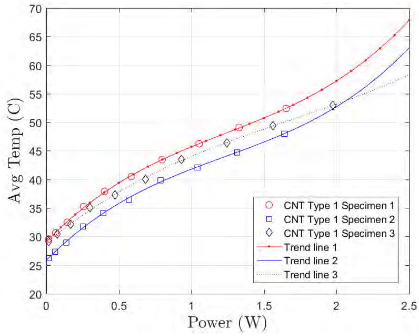
Figure B.25: This plot shows that a 3rd Order Polynomial curve fitted to the data accurately represents the known data points for Type 1 specimens
