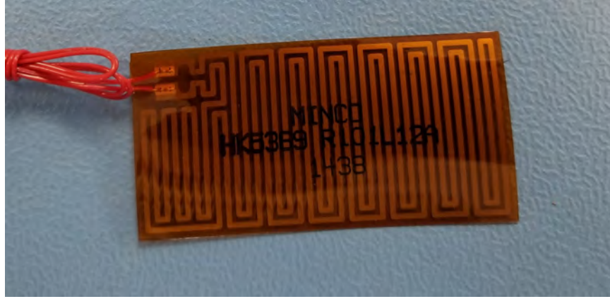
Figure 3.10: Minco TM HK5369 etched foil battery heater used on AFIT CubeSats
