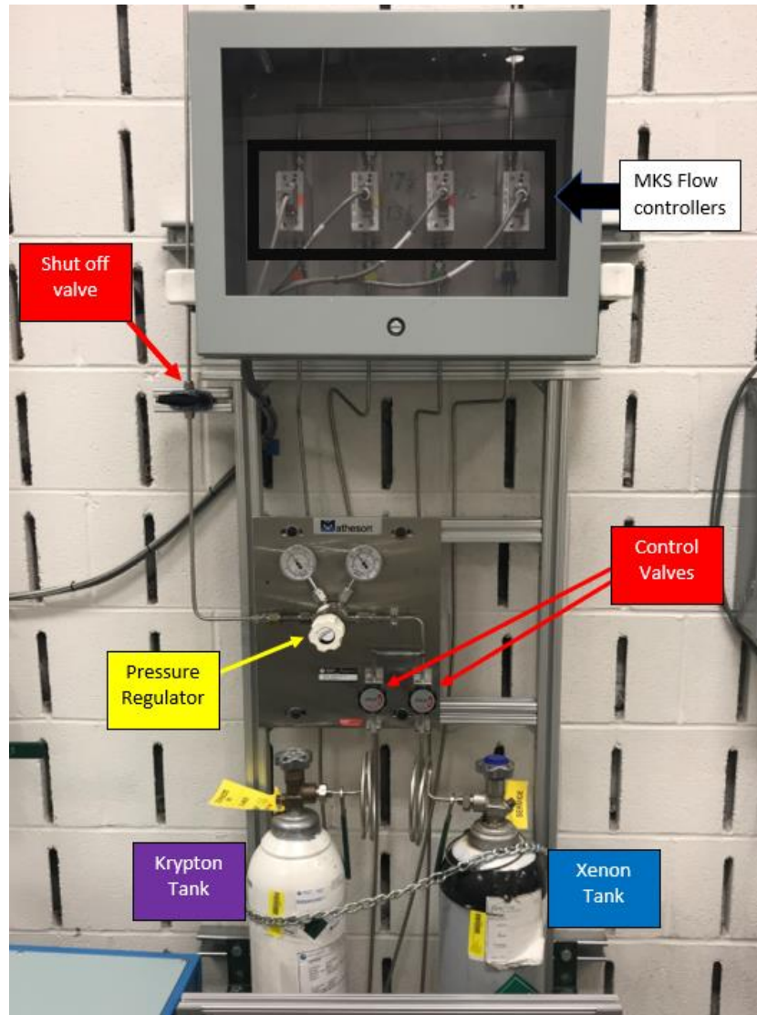
Figure 13: Propellant set-up
