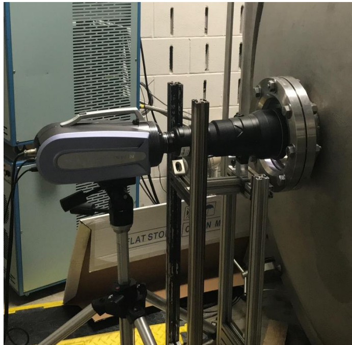
Figure 14: High speed camera set-up
