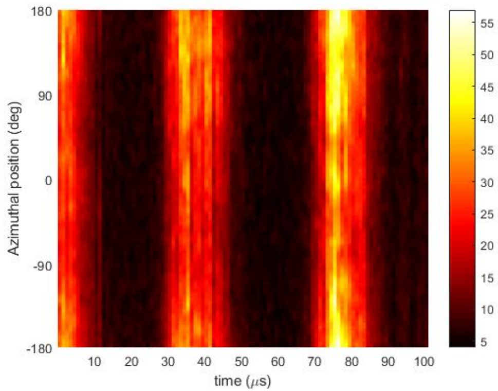
Breathing Mode Test 2, V_D = 75 V, I_D = 3.2 A
