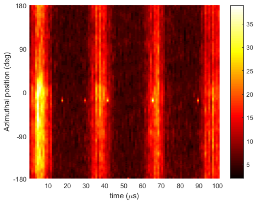
Breathing Mode Test 14, V_D = 250 V, I_D = 2.4 A
