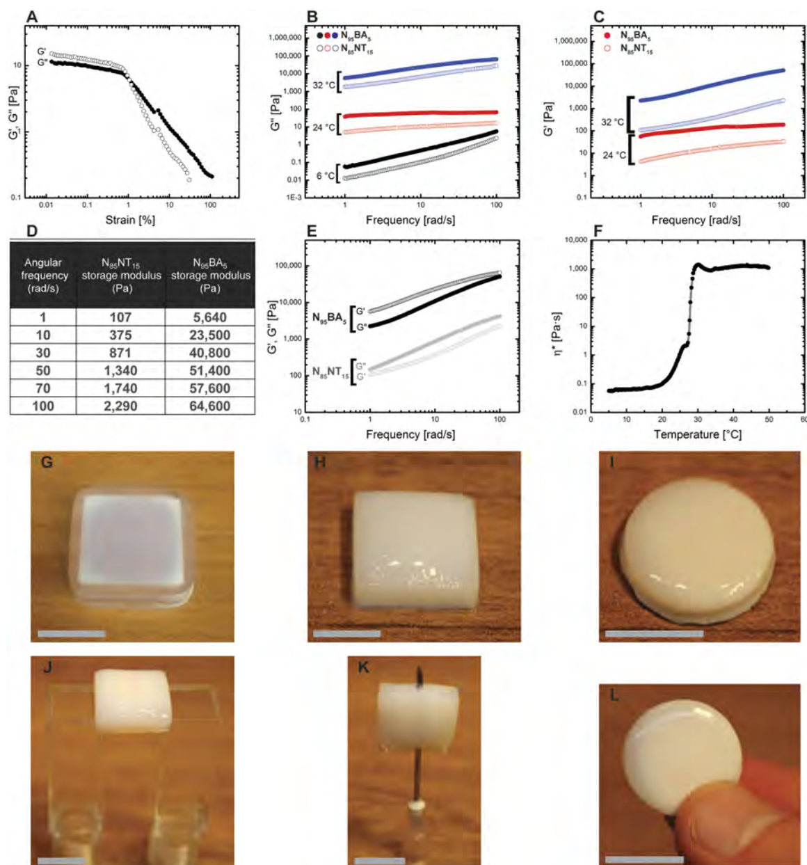
Fig. 2. Rheological characterization and hydrogel differentiation. (A) Storage and loss moduli ( G' and G'' , respectively) over strain for N 95 BA 5 . (B and C) G'' (B) and G' (C) modulus representations of viscoelastic behavior for co-BA and co-NT as a function of angular frequency at fixed strain. (D) Table of storage moduli for co-NT and co-BA compositions at different angular frequencies. (E) Storage and loss moduli ( G' and G'' , respectively) over frequency for co-NT and co-BA compositions. (F) Measurement of complex viscosity for N 95 BA 5 according to temperature. (G to I) Images of square and round gel molds formed by heating the hydrogel solutions to 32°C. Scale bars, 1 cm. (J to L) Images of solid N 95 BA 5 hydrogel demonstrating horizontal resilience (J), vertical resilience (K), and strength of form on contact (L). Scale bars, 1 cm.
