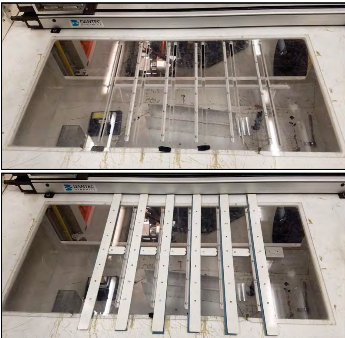
Figure 16. AFIT wind tunnel top access panel. Access panel without the inserts (top) and access panel with the inserts in place (bottom).
