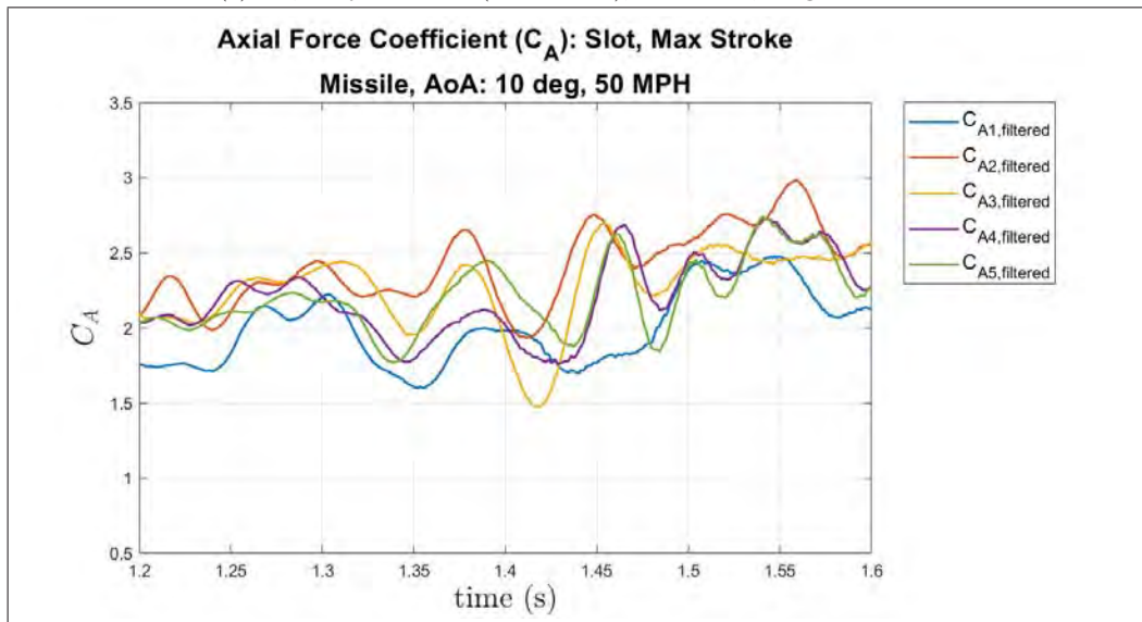
(b) C_A , Fully Extended (Max Stroke), 10.0° AoA, Small Window
