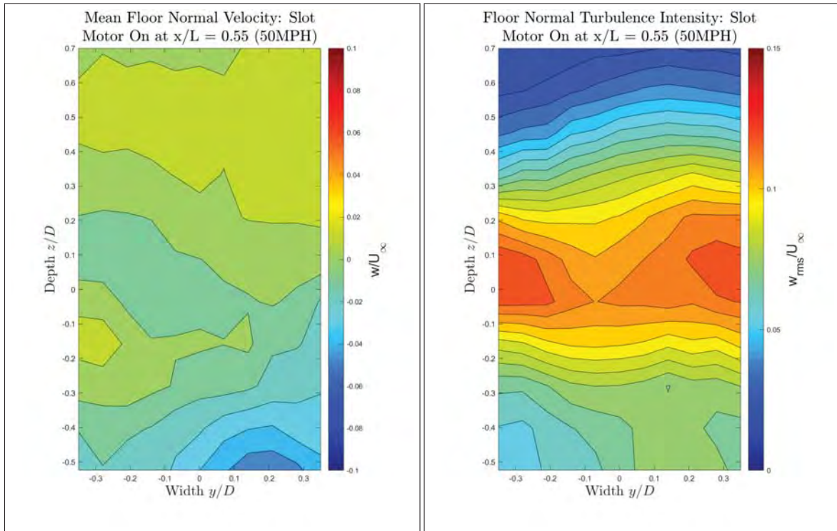
(a) Mean Floor Normal Velocity: Slot (50mph)
