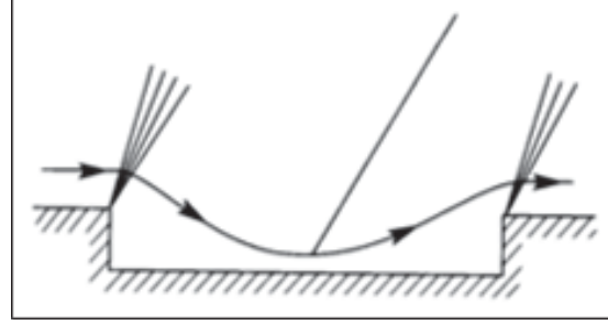
(d) Transitional closed cavity flow field at supersonic speeds 10 < L/D < 13
