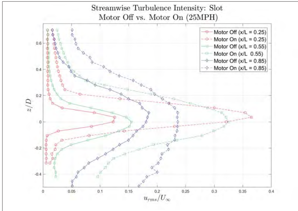
(b) Streamwise Turbulence Intensity: Slot (25mph)
