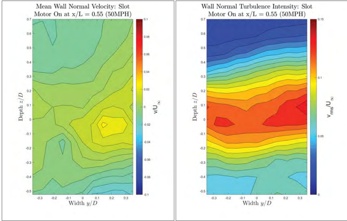
(a) Mean Wall Normal Velocity: Slot (50mph)
