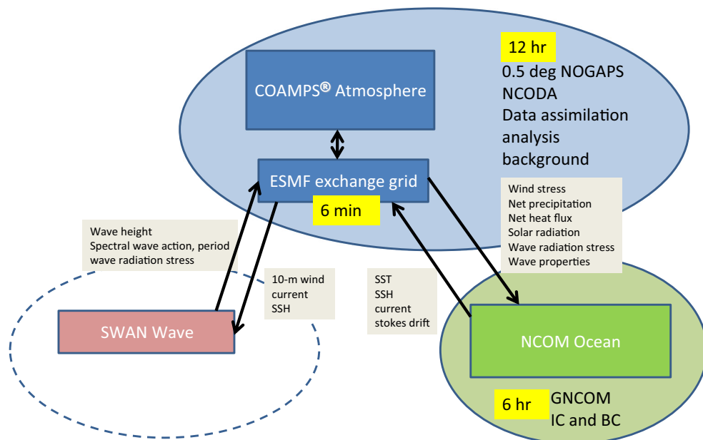
Fig. 1 Coupled Ocean-Atmosphere Mesoscale Prediction System setup and data exchange
