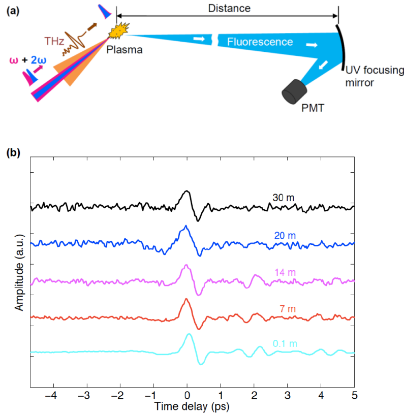
Fig. 1. (a) Schematic of the experimental setup used to remotely sense THz waves using two-color ( \omega and 2\omega ) THz radiation enhanced emission of fluorescence (THz REEF) at different distances; (b) THz waveforms sensed/detected at distances of 0.1 m, 7 m, 14 m, 20 m, and 30 m respectively. PMT, photomultiplier tube.
