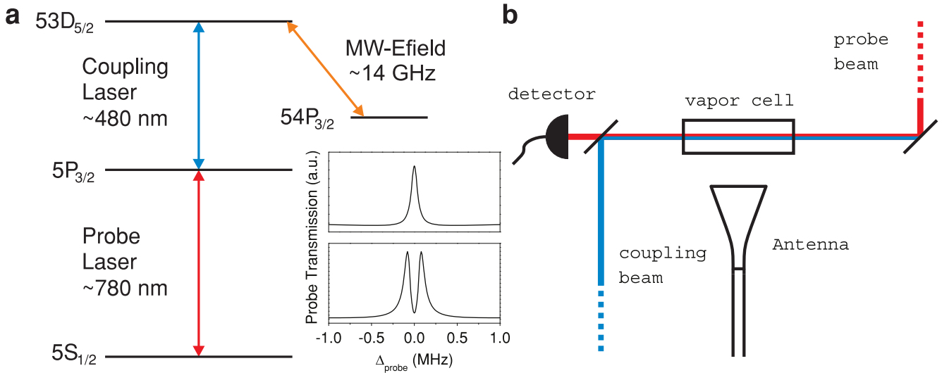
Figure 1. (a) An example atomic energy level structure for the measurement for the case of ^{87}\text{Rb} . The lasers are all generated using diode laser technology. A measurement takes place by recording the probe laser transmission in the presence of the coupling laser. If the RF-FI electric field was not applied then a narrow transmission peak for the probe laser is observed on resonance where the probe beam would normally be absorbed, upper graph in (a). This phenomena is referred to as electromagnetically induced transparency (EIT). When a resonant RF-FI electric field is applied to a third transition, a narrow absorption feature is induced within the transmission window, lower graph (a). The signal is extremely sensitive to the amplitude of the applied RF-FI electric field because the Rydberg atom transitions have extremely large transition dipole moments, the amplitude is converted into a frequency difference and the feature is the result of quantum interference between the different excitation pathways. Since EIT is a coherent multi-photon process, it is sub-Doppler so it can have relatively high spectral resolution in a vapor cell. Another advantage is that we have up-converted the RF-FI electric field signal to the probe laser frequency. (b) The experimental setup for testing. The probe and coupling fields counter-propagate through the cell.
