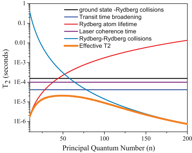
Figure 5. T_2 times for various processes as a function of n . Decreasing frequency is towards larger n . 100 MHz is around n = 135 . The Rydberg collision rates for Rydberg–Rydberg collisions are calculated for a pure C_6 long range interaction. The beam diameter is assumed to be 1 mm and the laser bandwidth is 100 kHz. The vapor cell has a length of 2.5 cm. The vapor cell is at room temperature. The Rydberg atom population is 0.0001. These parameters match ones we have used for prior experiments. The figure provides an idea of the factors affecting T_2 at different frequencies or n . The effective T_2 taking into account all the dephasing processes listed is shown for these conditions in orange.
