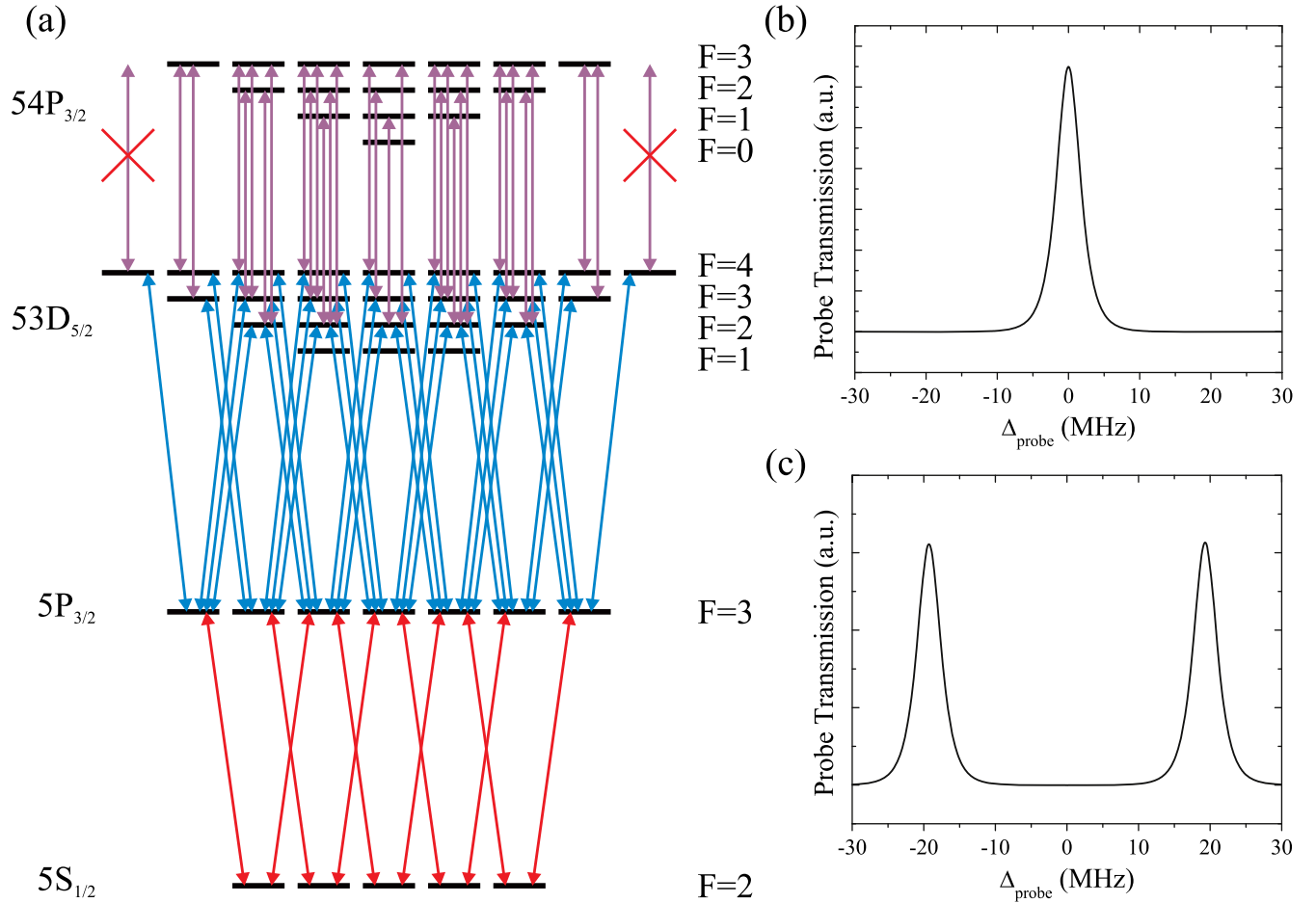
Figure 4. (a) An energy level diagram for the 52 states of the ^{87}\text{Rb} system labeled. The arrows indicating the transitions are for \sigma -polarized probe and coupling lasers and a \pi -polarized RF electric field. The 54P_{3/2} states are shown above the 53D_{5/2} states so that the diagram is easier to read. The laser polarizations correspond to an atomic quantization axis chosen along the probe and coupling laser beam propagation vectors. (b) Theoretical probe transmission lineshape for the effective three-level system obtained for the ‘stretched’ states in the system. (c) Theoretical probe transmission lineshape for the ‘non-stretched’ states in the system.
