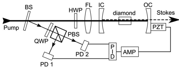
Fig. 12. Active stabilization of cavity length of a near concentric resonator using the Hänsch-Couillaud-type locking scheme. BS beam splitter, FL focusing lens IC input coupler, OC output coupler, PZT piezo actuator, QWP quarter-wave plate, HWP half-wave plate, PBS polarizing beam splitter, PD photodiode, PID controller, AMP high voltage amplifier.
