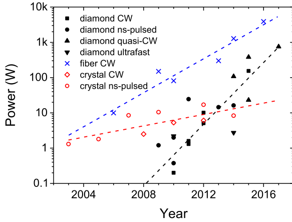
Fig. 4. Achieved average/CW output power of DRLs [15], [17]–[21], [44], [53], [65], [71], [72], [75], [77], [79]–[82] compared to non-diamond Raman crystals [72], [73], [83]–[89] and Raman fiber lasers [90]–[95]. On-time powers are used for quasi-CW (long-pulse) DRLs in the regime of steady-state thermal gradients ( >100 \mu\text{s} ).
