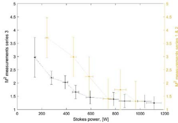
Fig. 2 Output Stokes beam quality as a function of output power for three different experimental cases (1,2,3) with similar conditions but some variability in pump beam quality.
