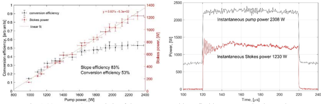
Fig. 1 (a) Power characteristic of the DRL pumped by a flashlamp-pumped Nd:YAG laser. (b) Power-calibrated oscilloscope trace of a pump pulse and corresponding Stokes output pulse at maximum power.
