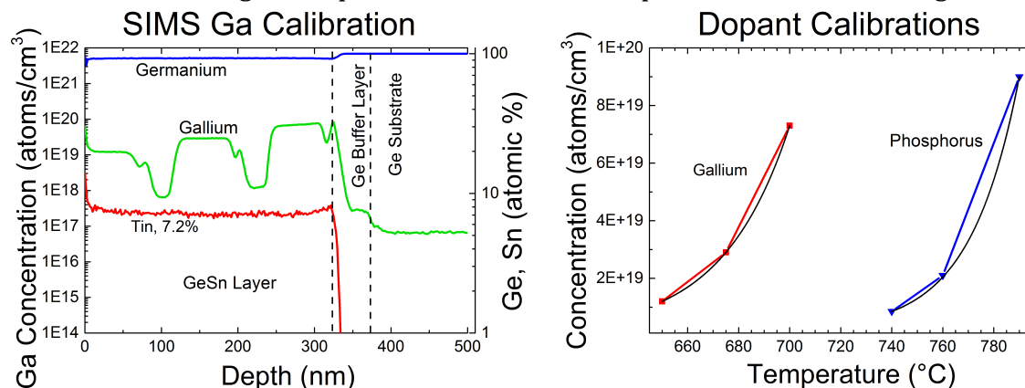
Figure 3. Left panel: secondary ion mass spectrometry (SIMS) plot of gallium concentration in atoms/cm 3 (left y axis), and tin concentration in percent (right y axis) versus material depth. For this stepped calibration sample, the dopant cell was opened for a growth of 75 nm, then closed for 25 nm while the Ge cell was ramped to a lower temperature. Right panel: phosphorus (right, blue) and gallium (left, red) concentrations in the grown layer versus effusion cell temperature. The exponential fitting for each cell flux is shown as overlaid black lines, for a GeSn growth rate of 1 nm/min. For different GeSn growth rates, the net doping concentrations can be easily scaled.
