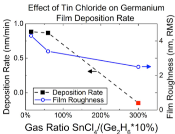
Figure 8. CVD Deposition with \text{SnCl}_4 vapor and digermene, showing the effect of \text{SnCl}_4 co-flow on the Ge deposition rate under ultra high vacuum (UHV) conditions. As the relative \text{SnCl}_4 flow increased, the films became smoother with no Sn incorporation, but the deposition rate decreased to below zero (i.e. etching). All growths were performed at a temperature of 285 °C and a pressure of \sim 1 \mu\text{bar} .
