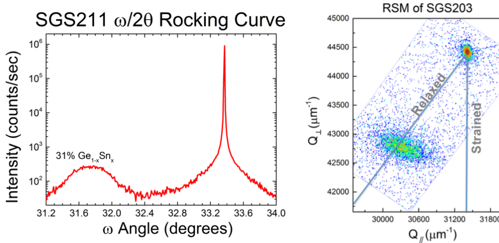
Figure 1. Left panel: x-ray rocking curve for GeSn sample (SGS211) with 31% Sn. Compared to the narrow Ge substrate peak near the diffraction angle of 33.4°, the wider GeSn peak near 31.75°, and the absence of interference (Pendellösung) fringes, was attributed to the presence of misfit dislocations that propagate from the Ge substrate interface into the GeSn layer, which has a larger lattice constant than Ge. Right panel: reciprocal space map (RSM) of sample SGS203 with 26 % Sn, showing intensity contours plotted with respect to the vertical reciprocal lattice vector Q_{\perp} and the in-plane ([110] direction) reciprocal lattice vector Q_{\parallel} . The broader GeSn peak on the left side of the RSM lies along the diagonal relaxation line, indicating nearly complete relaxation.
