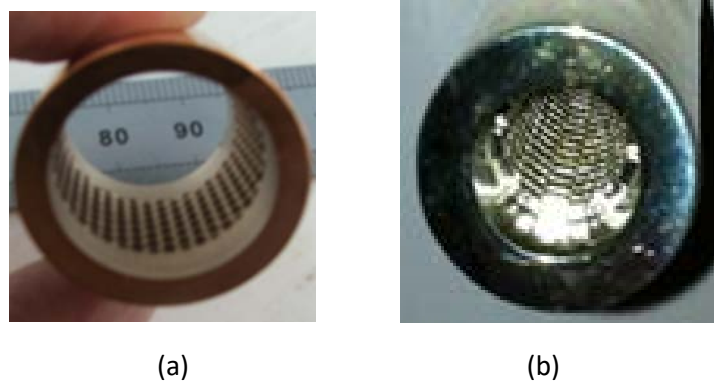
Fig. 5.1 Examples of metallic periodic surface lattice enhanced cavities (a) copper cavity constructed using electrodeposition on an aluminum mandrel (b) silver/chromium alloy cavity manufactured by a casting process using a 3D printed pattern to create the mold.
