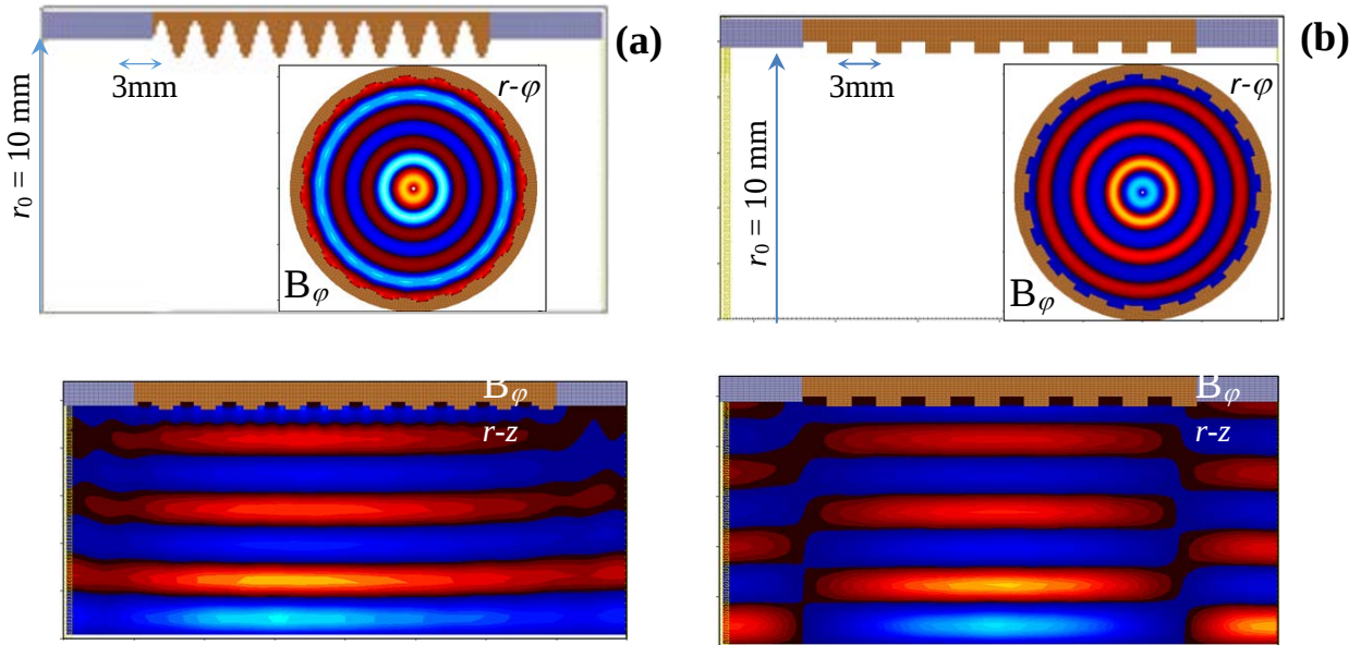
Figure 4.1 Numerical models of the (a) high and (b) low contrast 2D PSLs showing r - z cross-sections of the structures and contour plots of the eigenmodes' azimuthal magnetic field component excited, in r - \phi (insert to the first figure) and r - z (second figure)
