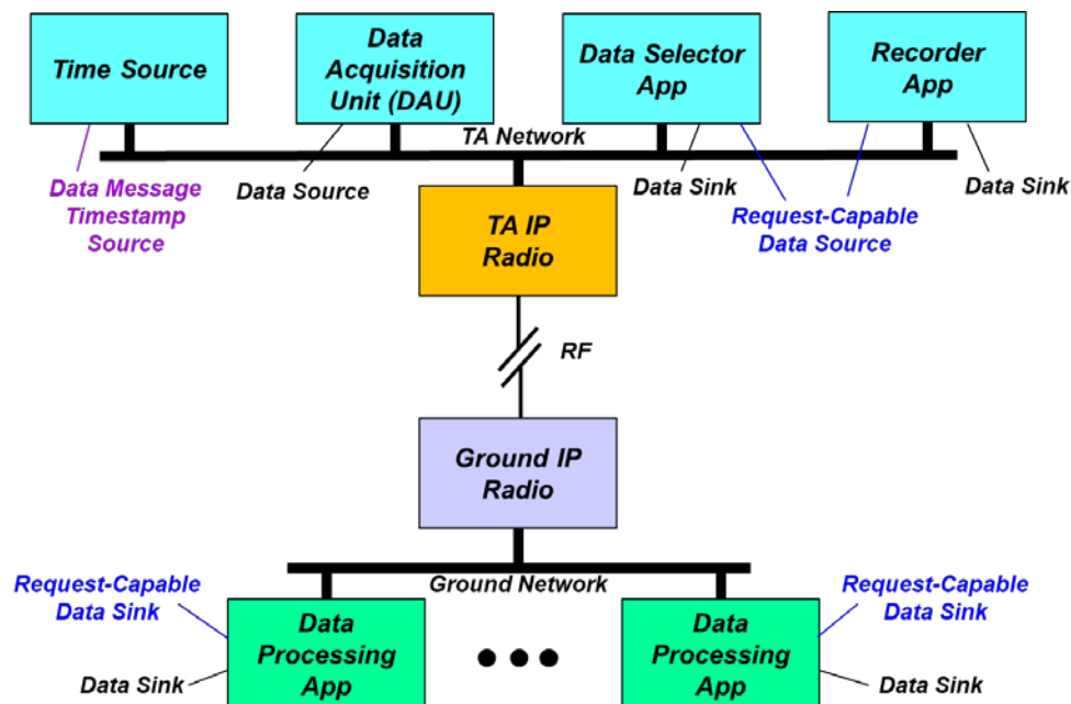
Figure 3. Simple Telemetry Network System
