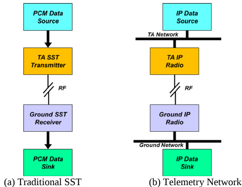
Figure 1. Telemetry Data Distribution Overview.
