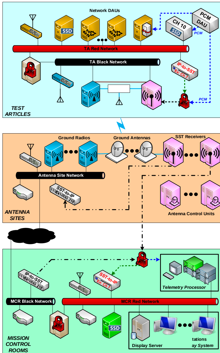
Figure 4. Flight Test System with both SST and TmNS Elements
