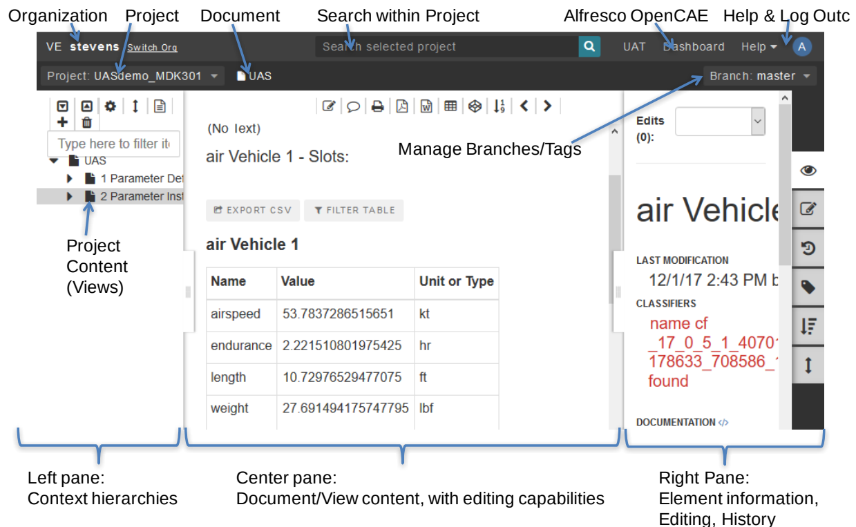
Figure 55. View Editor
