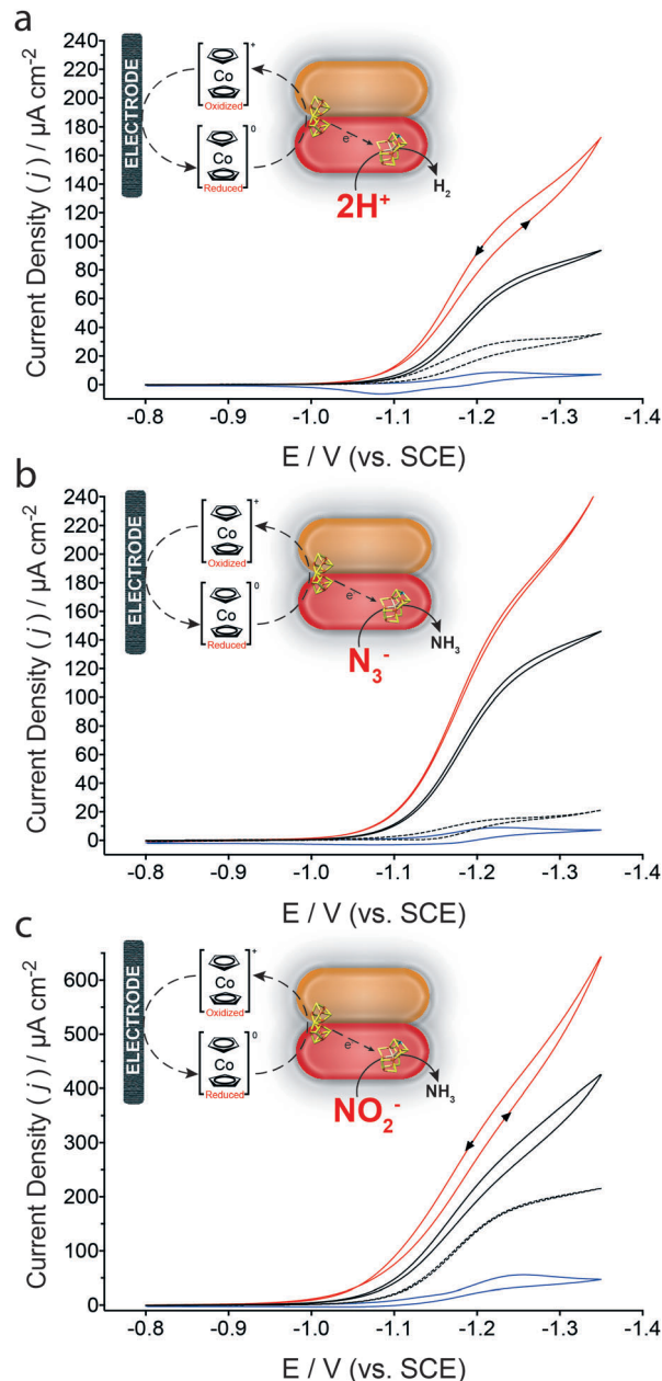
Fig. 2 Cyclic voltammograms of wild-type MoFe protein bioelectrode in HEPES buffer (pH 7.4, 250 mM) containing 200 \mu\text{M} \text{Cc}^+ at a scan rate of 2 \text{ mV s}^{-1} (solid black lines) in the (a) absence of any additional substrates, or in the presence of (b) 50 \text{ mM} \text{N}_3^- or (c) 50 \text{ mM} \text{NO}_2^- . MoFe protein bioelectrodes were also prepared with the \beta -98 Tyr→His MoFe protein (red solid lines). Equivalent control bioelectrodes were either prepared with BSA (blue line) or apo-MoFe protein (black dashed line) in the presence of the respective substrates. All voltammetric experiments were performed in an anaerobic tent (Ar) where the \text{O}_2 concentration was continuously <1 ppm, at room temperature ( \sim 21^\circ\text{C} ). Reactions depicted in (b) and (c) are unbalanced.
