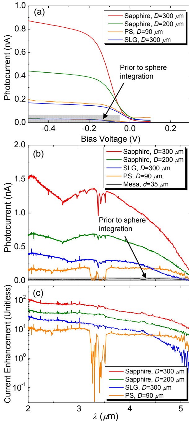
Fig. 27. (a) Photocurrent measured at different bias voltages from -0.5 to 0.1\ \text{V} for d=35\ \mu\text{m} . (b) FTIR photocurrent spectra at a negative bias of 0.3\ \text{V} with (colored curves) and without (black curve) the sphere. (c) Photocurrent enhancement factors, obtained by the division of FTIR photocurrent spectra at a negative bias of 0.3\ \text{V} by the corresponding spectrum obtained without sphere.
