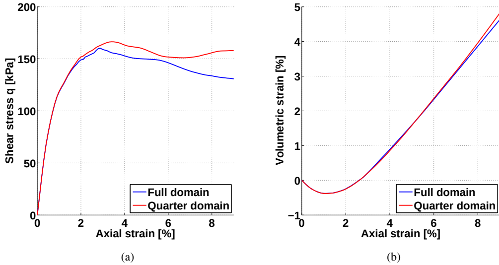
Figure 6.14: Global shear stress and volumetric strain behavior in globally drained triaxial compression test. Comparison of quarter-domain and full-domain simulations
