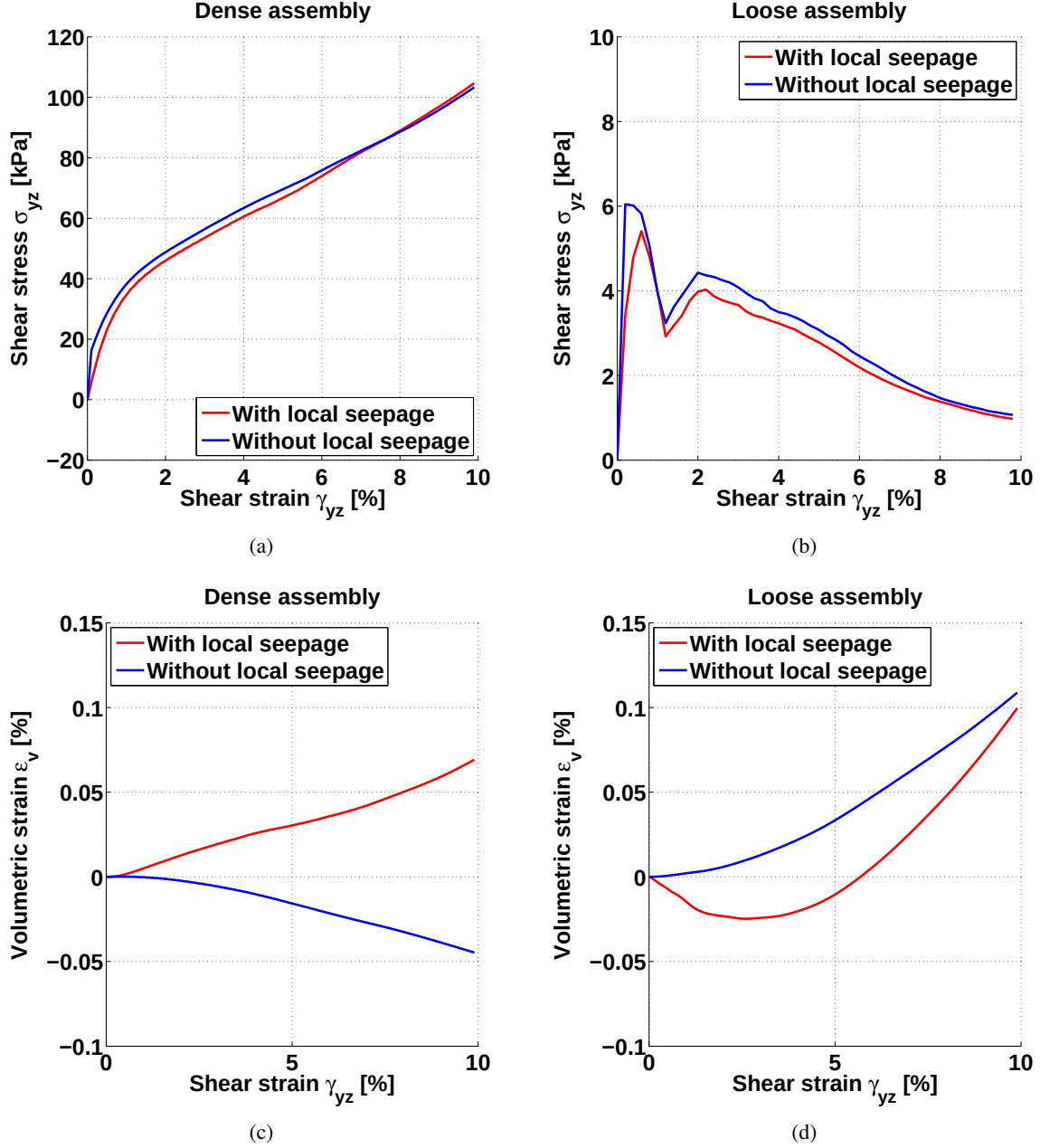
Figure 6.6: Comparison of global shear stress and volumetric strain behavior between globally undrained dense and loose assemblies with and without local diffusion
