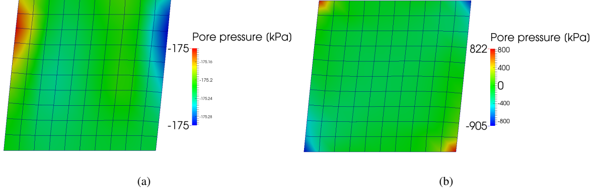
Figure 6.9: Comparison of pore pressure at 10% shear strain between (a) dense sample with local seepage and (b) dense sample without local seepage
