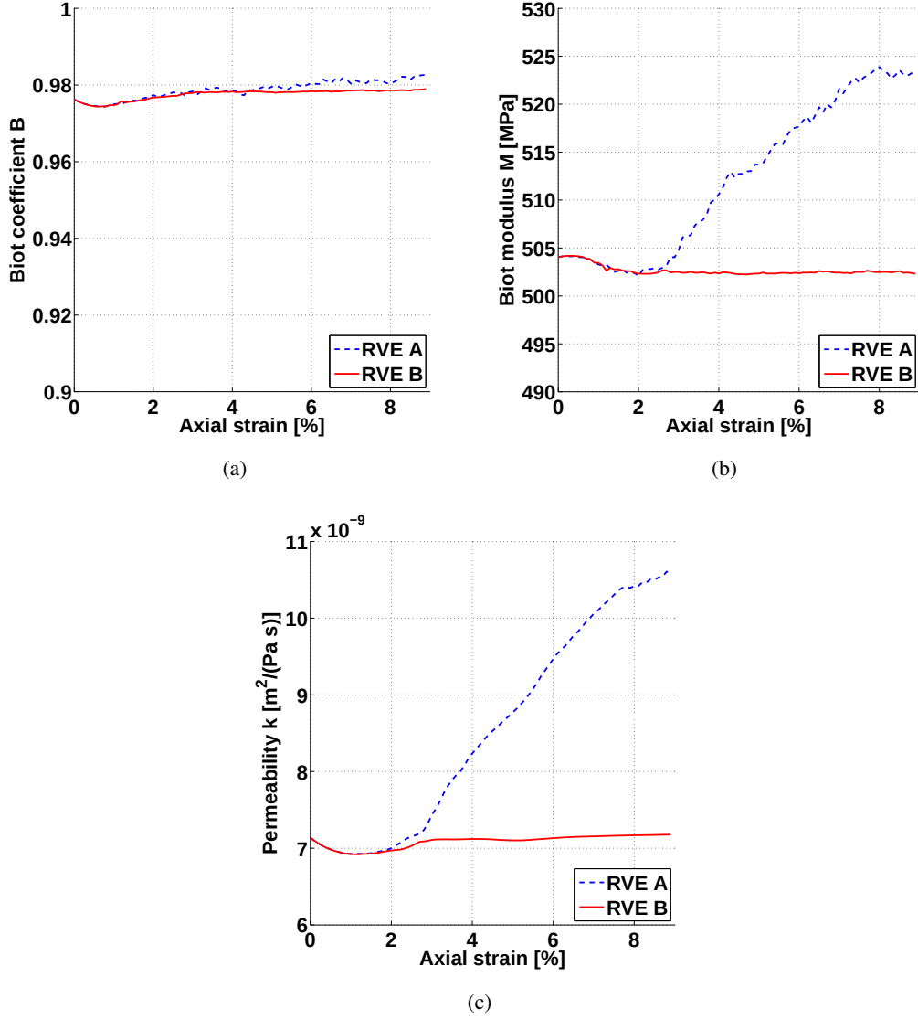
Figure 6.18: Evolution of (a) Biot's coefficient, (b) Biot's modulus and (c) effective permeability for RVE A (inside shear band, Fig. 6.15(c)) and RVE B (outside shear band, Fig. 6.15(c)).
