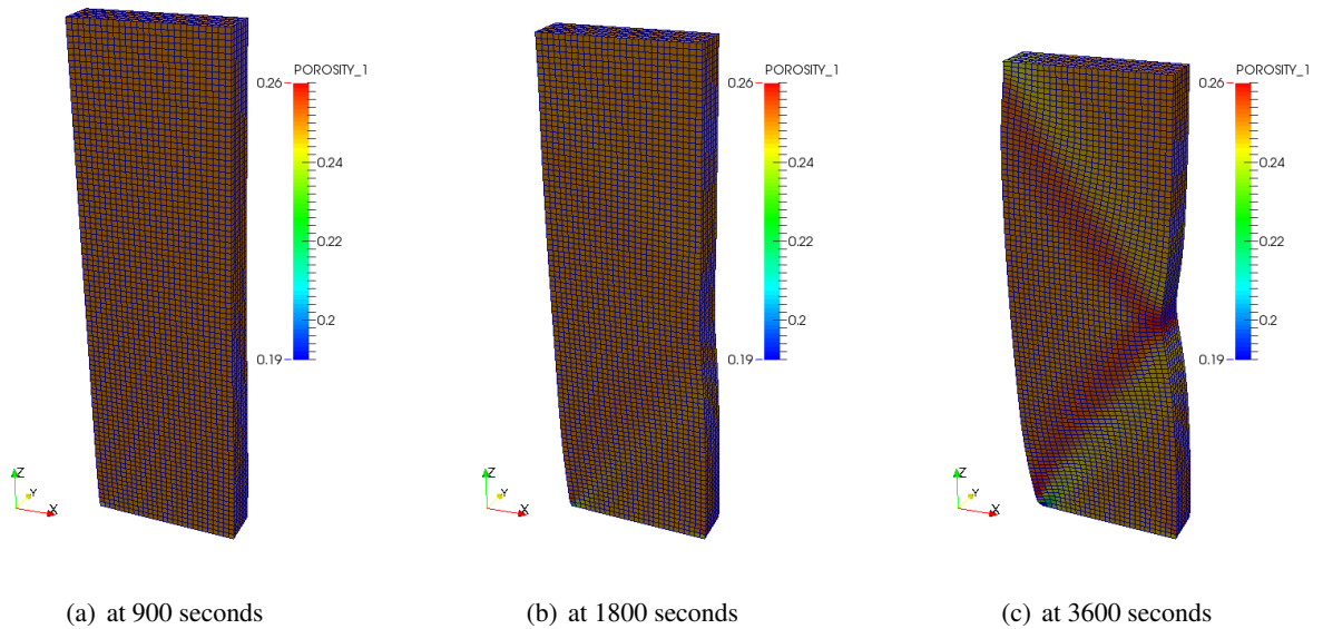
Figure 8.13: Porosity at various time during the biaxial loading test.
