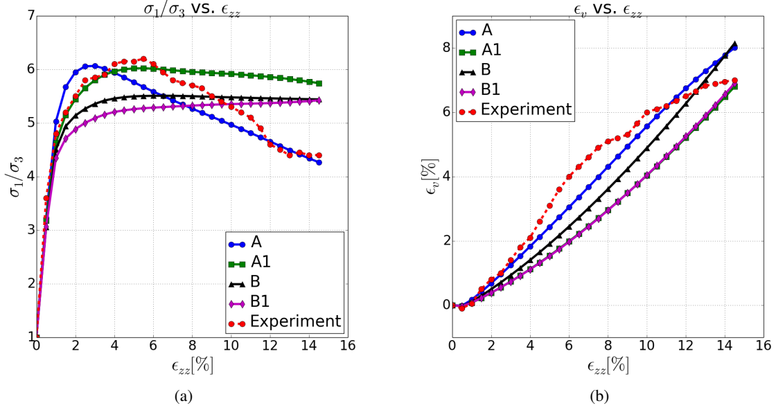
Figure 7.14: Stress ratio and volumetric strain responses of full sample simulation during the calibration procedure using Case A: only macroscopic responses; Case A1: equal weights of stress ratio, volumetric strain and local void ratio data, starts from results of Case A; Case B: macroscopic responses and local void ratio distribution; Case B1: equal weights of stress ratio, volumetric strain and local void ratio data, starts from results of Case B.
