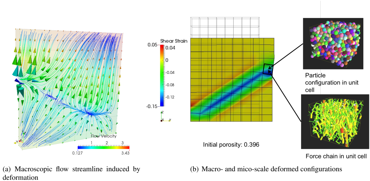
Figure 4.1: Preliminary results of an undrained triaxial compression test of a fully saturated granular specimen simulated via multiscale discrete-continuum coupling model developed by the PI.
