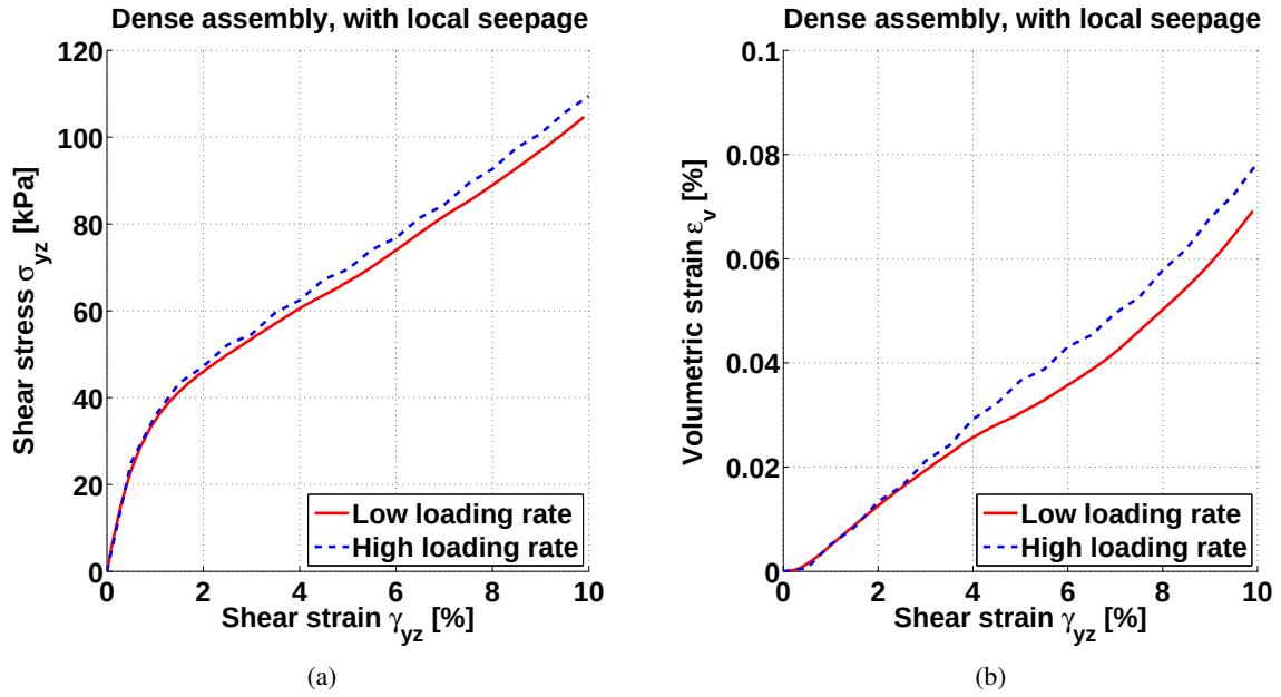
Figure 6.12: Comparison of global shear stress and global volumetric strain behavior between low loading rate (0.1% shear strain per second) and high loading rate (0.5% shear strain per second), finite strain formulation
