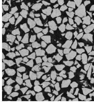
Figure 7.1: Reconstructed x-Ray image shows the clear contrast between grain and water and air. The experiments in this study are performed using x-ray setup of laboratory 3SR at Grenoble University.
