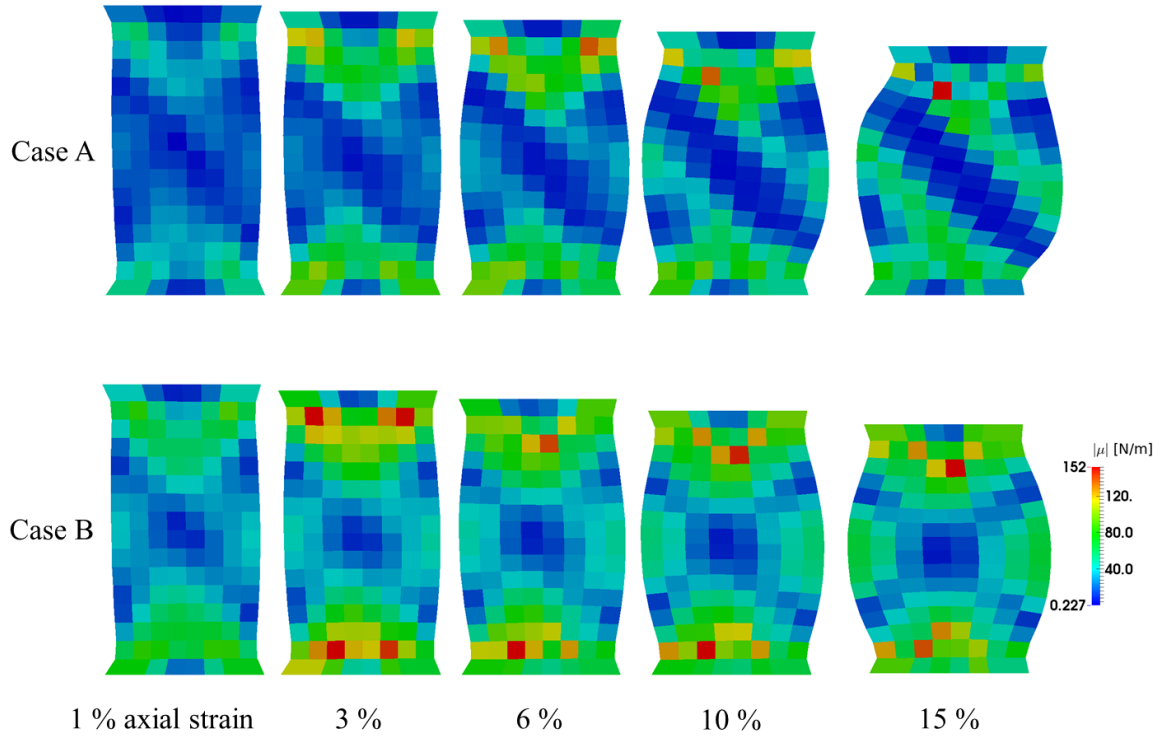
Figure 7.17: Evolution of shear localization in cross section YZ of calibration results of Case A and Case B, illustrated in the norm of couple stress.
