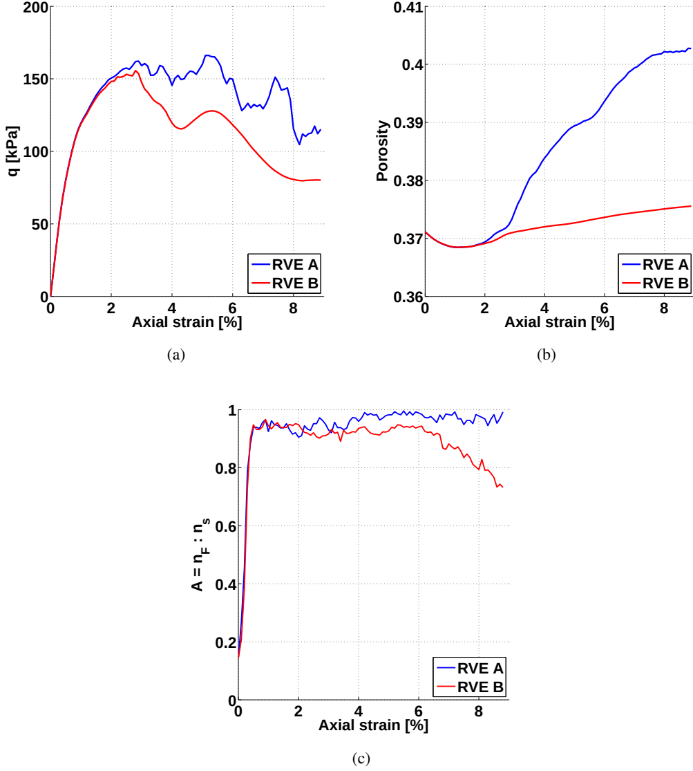
Figure 6.19: Evolution of (a) deviatoric stress q (b) porosity (c) A = \mathbf{n}_F : \mathbf{n}_s (relative orientation between anisotropic fabric and deviatoric stress directions) during triaxial compression test ( \dot{\epsilon}_z = 0.05\%/s ) for RVE A (inside shear band, Fig. 6.15(c)) and RVE B (outside shear band, Fig. 6.15(c)).
