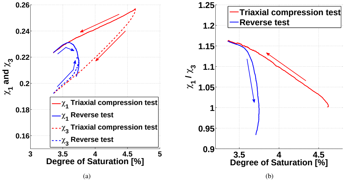
Figure 5.7: Major and minor principle values \chi_1 and \chi_3 of the Bishop's coefficient (a) and their ratio (b) vs. degree of saturation. At the late phase of the reverse test the major and minor principal directions switch between them, yet the subscripts 1 and 3 still refer to the same principal directions as before, allowing the ratio to be smaller than 1.
