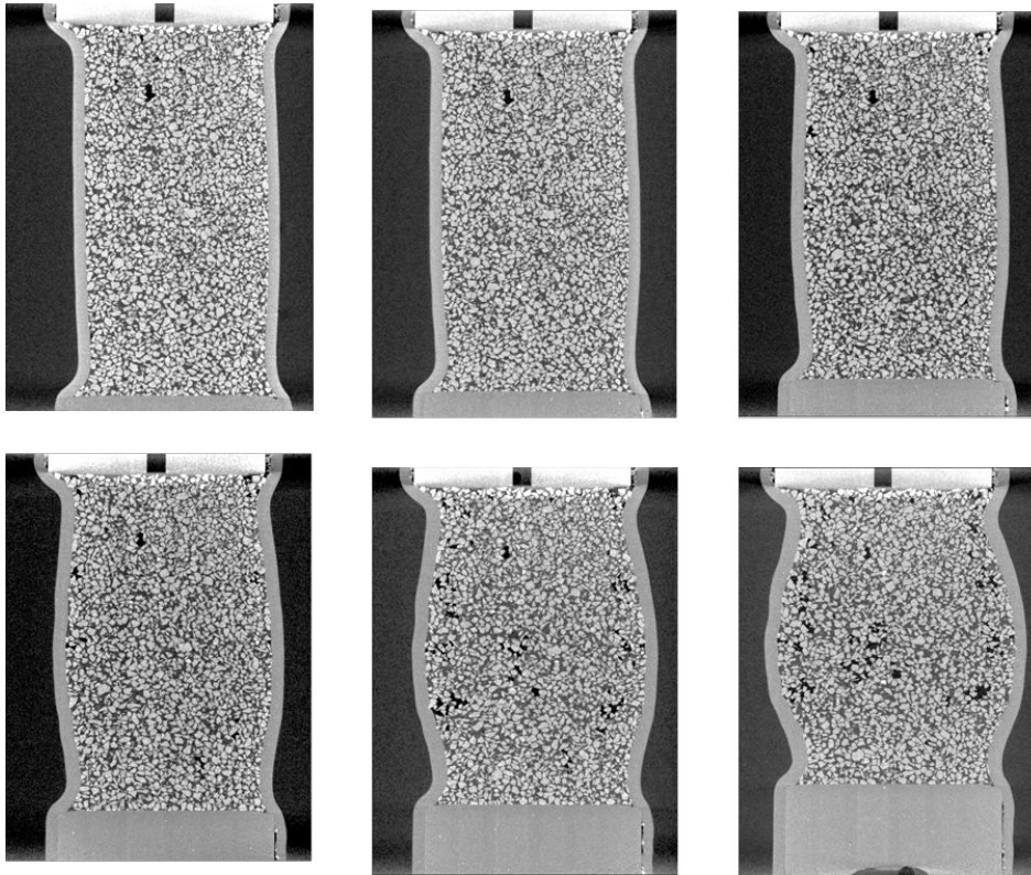
Figure 7.5: Micro-CT images of the cross section of the specimen at different axial strain level.
