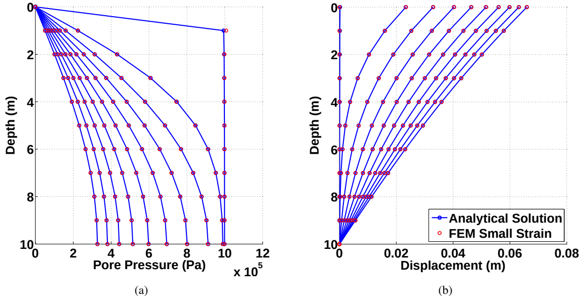
Figure 6.3: Response of saturated soil column under 1 MPa consolidation pressure from 0 s to 500 s (50 s between adjacent lines), verification of small strain formulation with analytical solutions (a) Pore pressure (b) Vertical displacement
