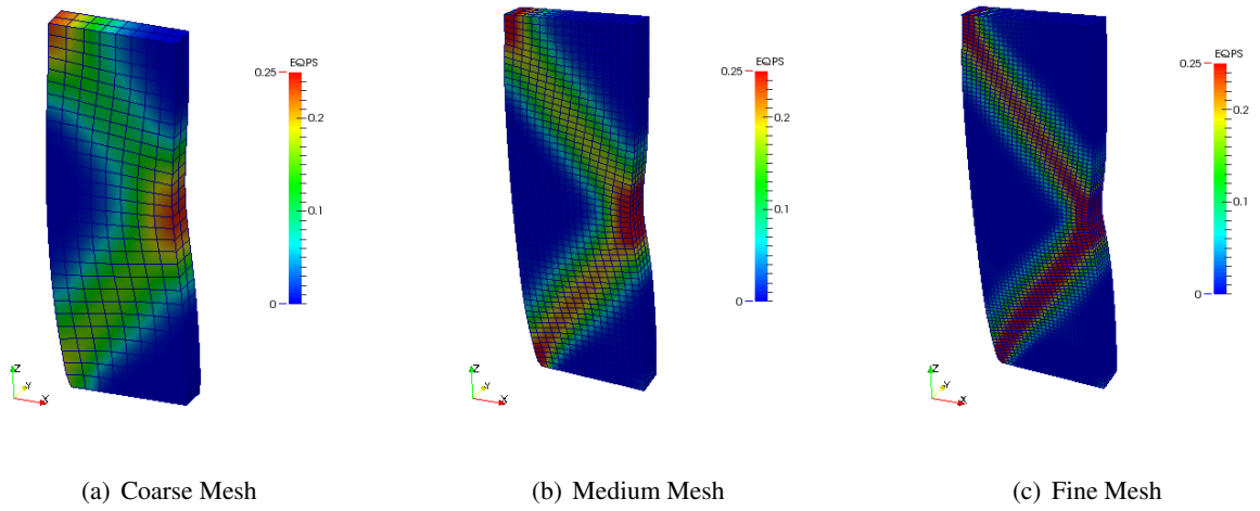
Figure 8.17: Equivalent plastic strain at t= 7200 seconds in three meshes.
