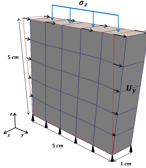
Figure 6.5: Geometry and boundary conditions for globally undrained shear test
