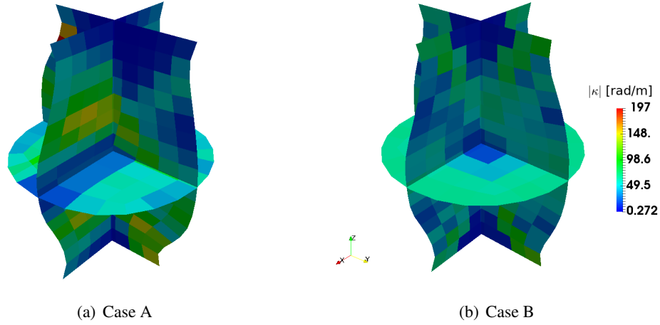
Figure 7.16: Norm of the curvature tensor |\kappa| = \sqrt{\kappa_{21}^2 + \kappa_{32}^2 + \kappa_{31}^2} for results of inverse problems A and B at residual stage
