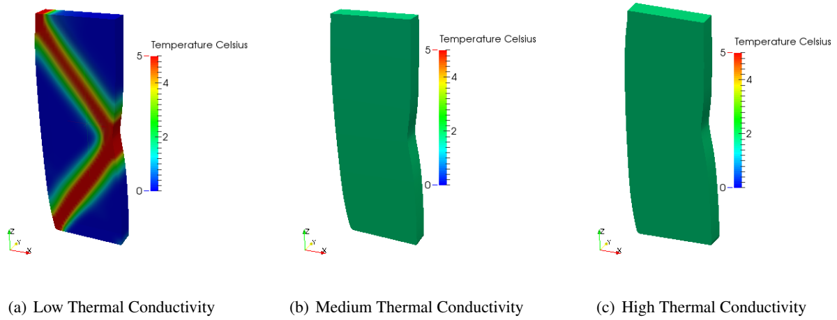
Figure 8.23: Temperature profile at time = 7200 seconds, with initial effective thermal conductivity equals to (a) 0.013 \text{ W/m/}^\circ\text{C} , (b) 1.33 \text{ W/m/}^\circ\text{C} and (c) 133 \text{ W/m/}^\circ\text{C} .
