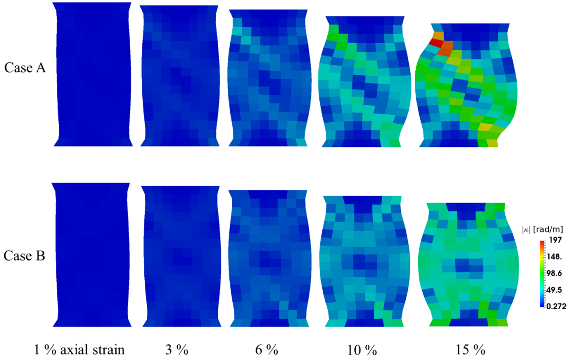
Figure 7.18: Evolution of shear localization in cross section YZ of calibration results of Case A and Case B, illustrated in the norm of curvature tensor.
