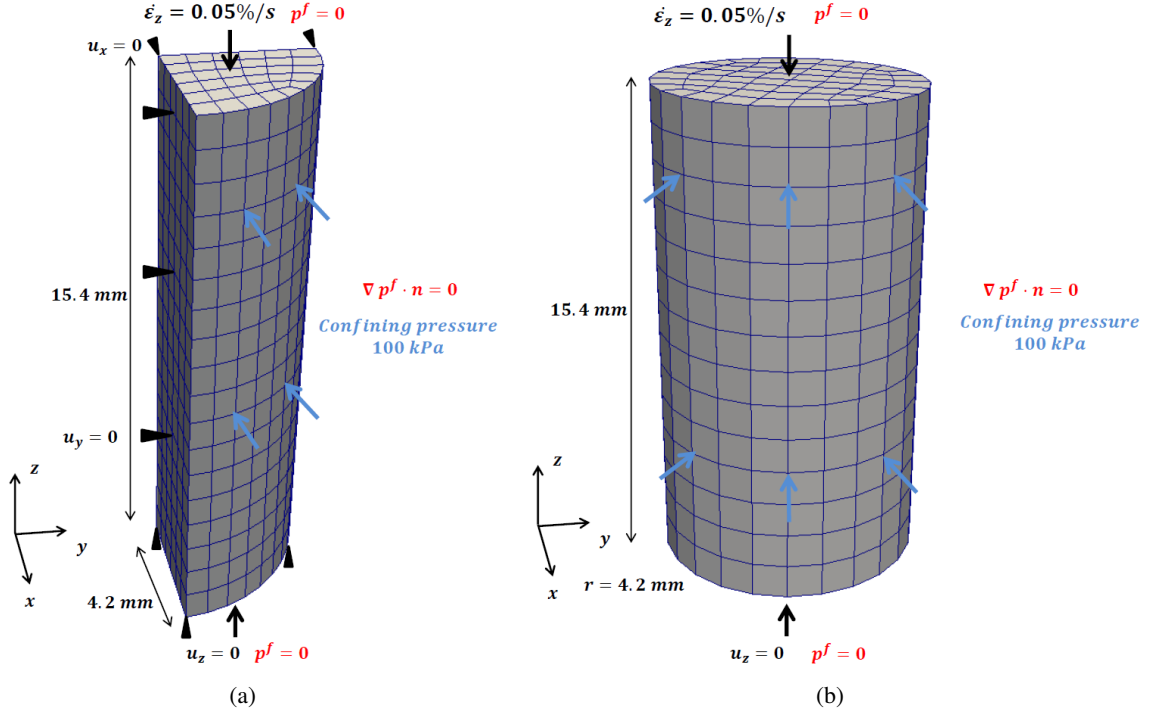
Figure 6.13: Geometry, mesh and boundary conditions for globally drained triaxial compression test. (a) Quarter-domain simulation. (b) Full-domain simulation
