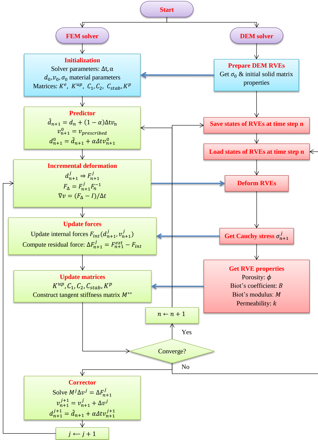
Figure 6.2: Flowchart of the multiscale semi-implicit scheme. Blue blocks represent initialization steps of the solution scheme ; Green blocks refer to FEM solver steps and red blocks refer to DEM solver steps; Blue arrows indicate the information flow between the two solvers.
