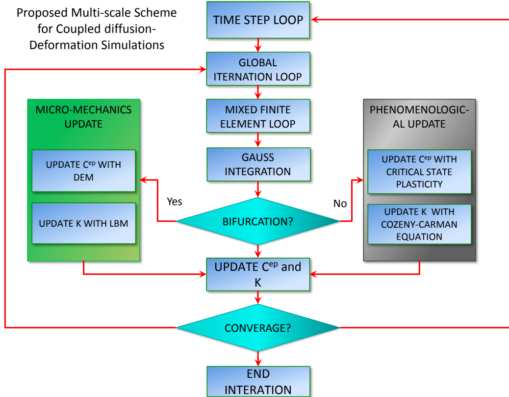
Figure 4.2: Multiscale LBM-DEM-FEM model that upscaling liquid-grain interactions at pore-scale to field scale continuum simulations. Length scale is preserved by modeling granular assemblies as three-dimensional non-local continua.
