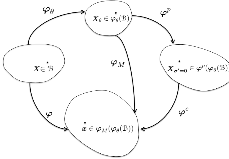
Figure 8.2: Multiplicative decomposition of the thermohydromechanics deformation.
