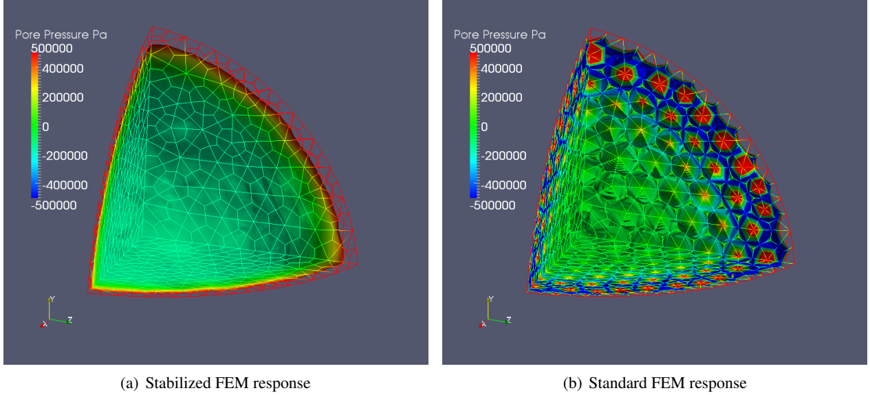
Figure 8.6: Pore Pressure Profile of undrained porous sphere in heat bath.
