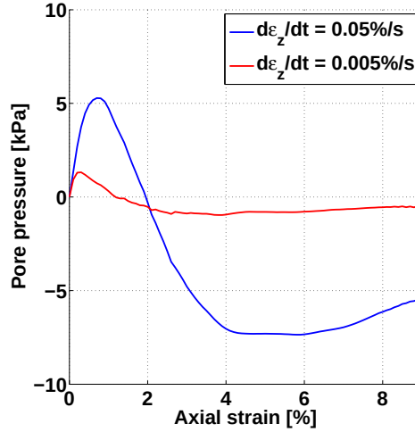
Figure 6.17: Evolution of pore pressure at the center of the cylindrical specimen during triaxial compression test subjected to two loading rate.
