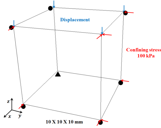
Figure 7.7: Domain and boundary condition for single unit cell calibration.
