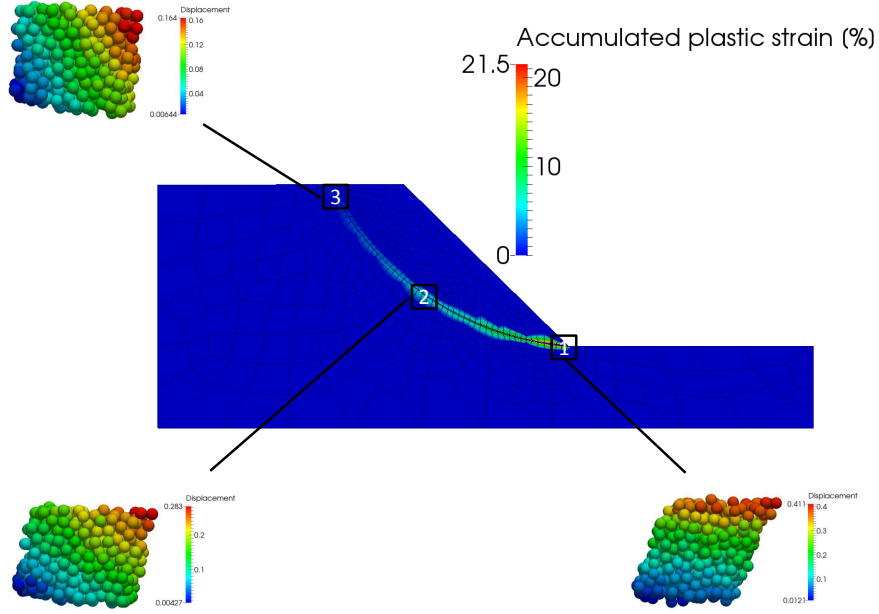
Figure 6.22: Accumulated plastic strain \bar{\epsilon}^P inside the slip surface on the verge of collapse (Load factor \alpha = 1.23 )
