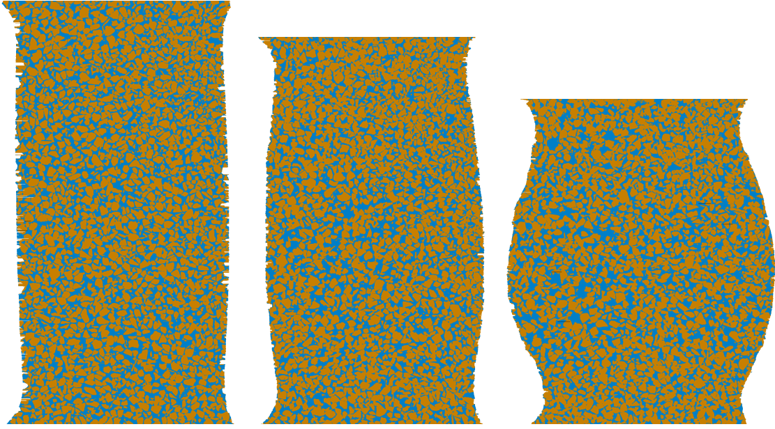
Figure 7.6: Cross sections of the "Binarized" two-phase images at axial strain = 0, 8 and 21 %.
