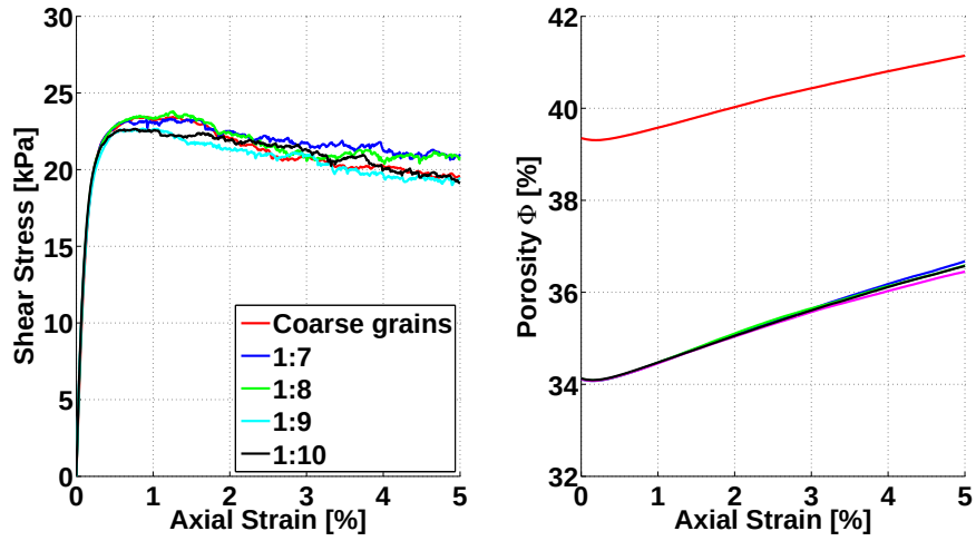
Figure 5.10: Shear stress (left) and porosity (right) versus axial strain curves with SU = 10\text{kPa} under constant confining stress 10\text{ kPa} . The samples are prepared with different ratios of the number of coarse grains and fine grains n_{\text{coarse}} : n_{\text{fine}}
