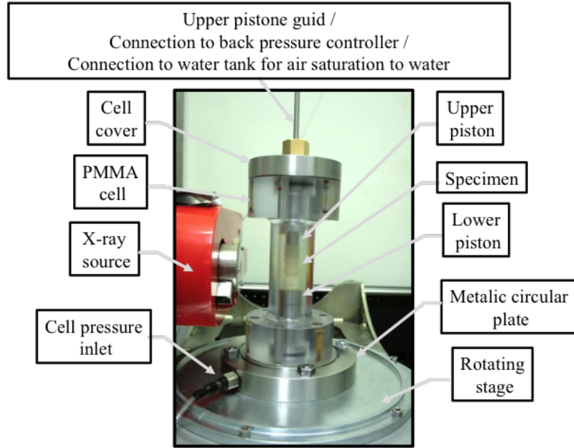
Figure 7.3: The PMMA cell in front of x-ray source with the specimen installed at its place inside the cell.
