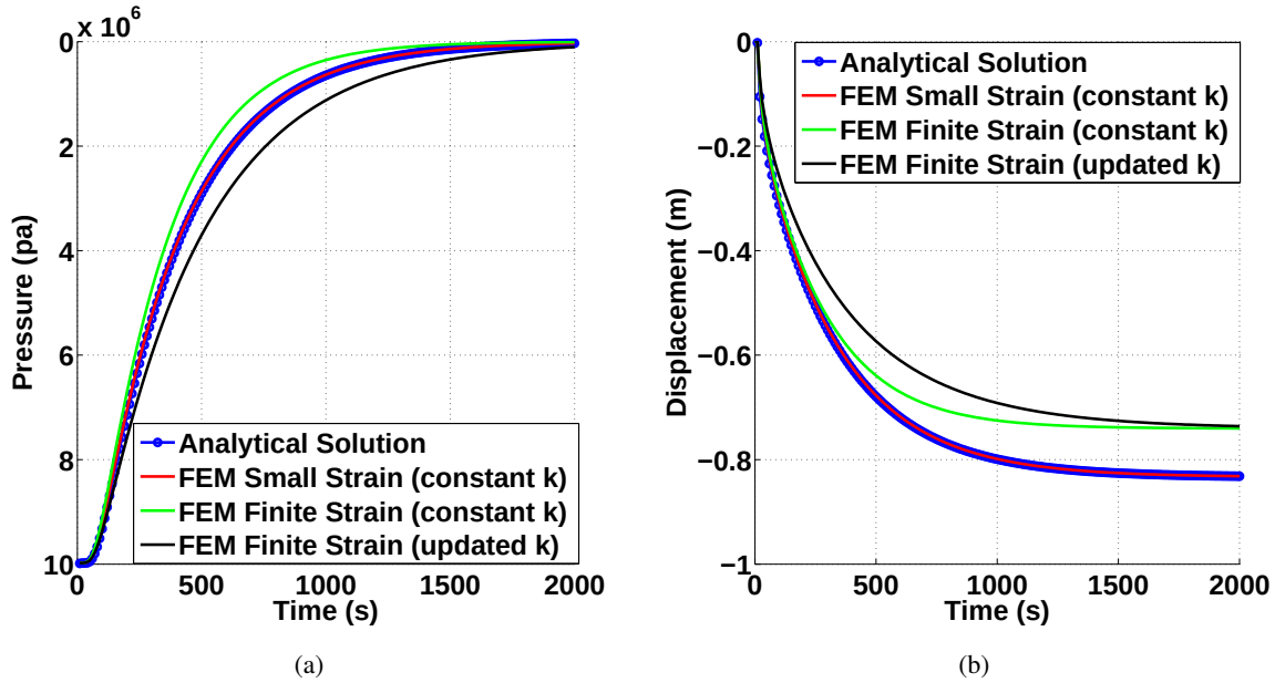
Figure 6.4: Response of saturated soil column under 10 MPa consolidation pressure. Comparison of analytical solution, numerical result from formulations of small strain, large strain with constant permeability k (in m/s) and large strain with k updated by the Kozeny-Carman equation. (a) Pore pressure evolution at bottom surface (b) Vertical displacement evolution at top surface
