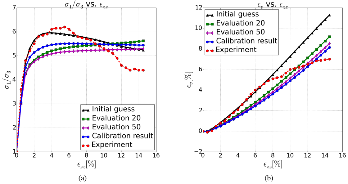
Figure 7.12: Stress ratio and volumetric strain responses of full sample simulation during the calibration procedure using macroscopic responses and local void ratio distribution (Case B).
