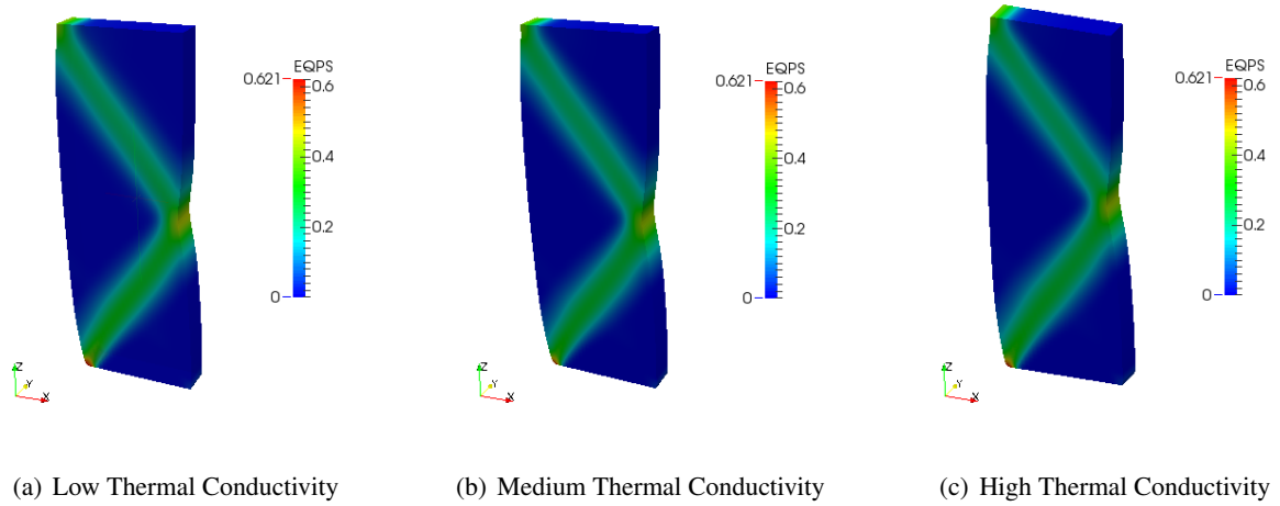
Figure 8.25: Equivalent plastic strain at time = 7200 seconds, with initial effective thermal conductivity equals to (a) 0.013\text{W/m/}^\circ\text{C} , (b) 1.33\text{W/m/}^\circ\text{C} and (c) 133\text{W/m/}^\circ\text{C} .
