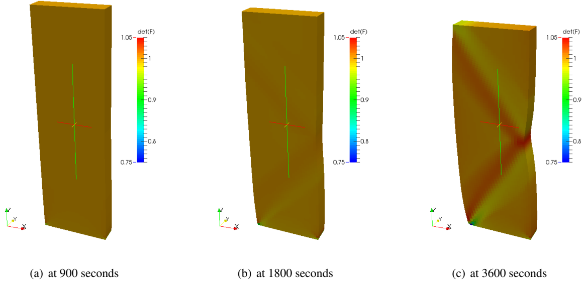
Figure 8.12: Determinant of the deformation gradient at various time during the biaxial loading test.
