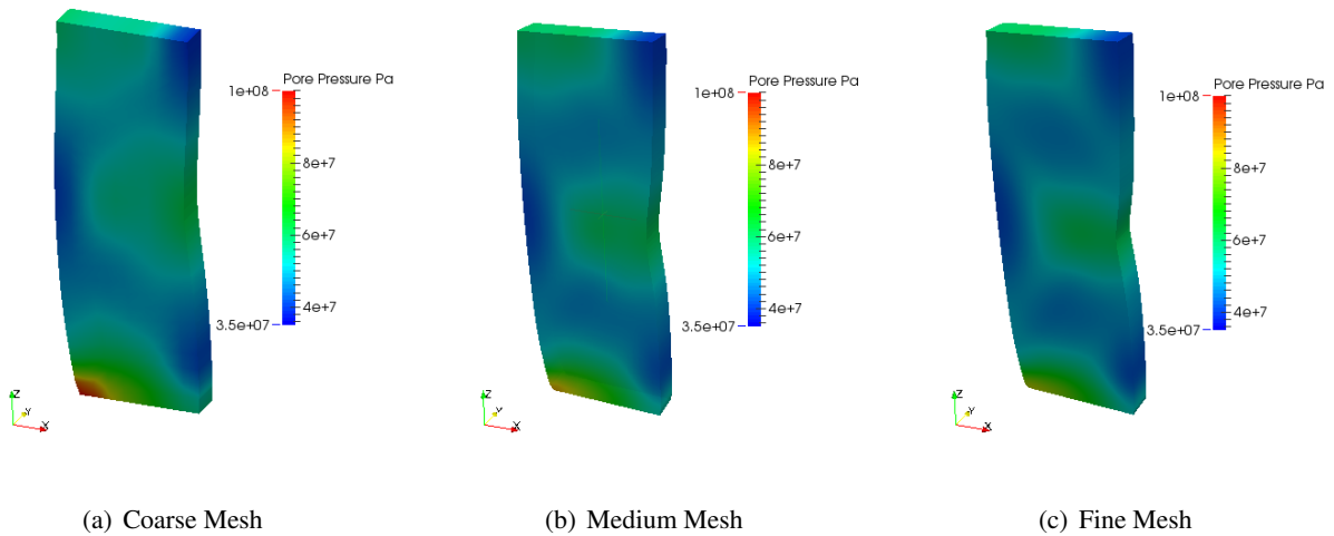
Figure 8.20: Pore Pressure at t= 7200 seconds in three meshes.
