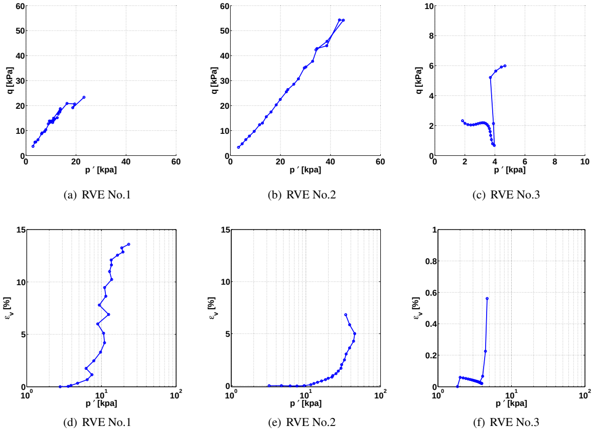
Figure 6.23: State paths of unit cells as labeled in Fig. 6.22 until slope collapses. Left: RVE No. 1; Middle: RVE No. 2; Right: RVE No. 3;
