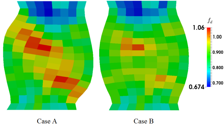
Figure 7.19: Distribution of f_d for results of inverse problems A and B at the residual stage. f_d = 1 indicates that the material is in critical state.
