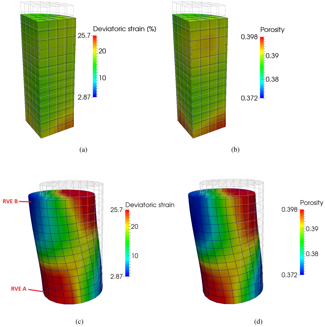
Figure 6.15: Distribution of deviatoric strain and porosity in globally drained triaxial compression test at 9% axial strain. Comparison of quarter-domain and full-domain simulations.
