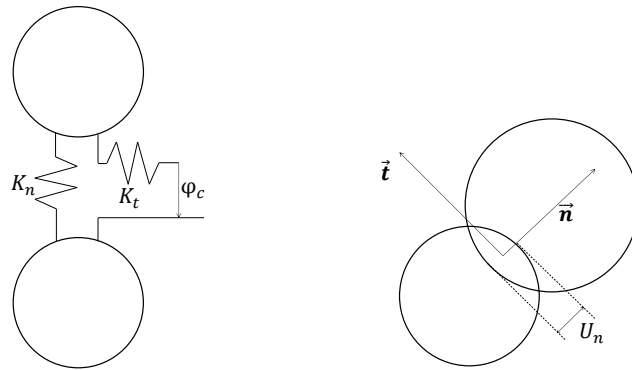
Figure 5.2: Contact friction model.
