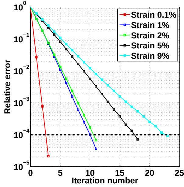
Figure 6.20: Convergence profiles of the triaxial compression test at different axial strain levels. The relative error is defined as \frac{\|\Delta \mathbf{F}^i\|}{\|\Delta \mathbf{F}^{(i=0)}\|} , where \Delta \mathbf{F}^i is the residual force at the iteration step i . The convergence is reached when the error falls below 10^{-4} .
