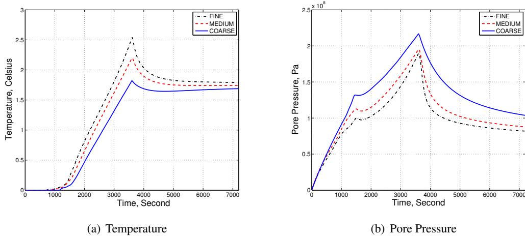
Figure 8.21: Time histories of temperature and pore pressure at the lower left corner of the three meshes.
