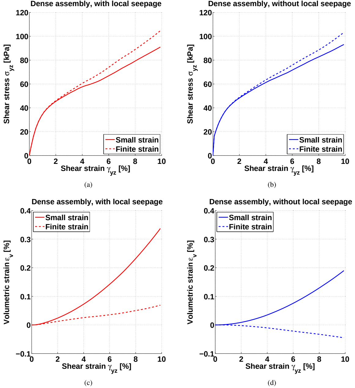
Figure 6.8: Comparison of global shear stress and global volumetric strain behavior between small strain and finite strain formulation. Left: globally undrained with local diffusion condition, Right: globally undrained but without local diffusion condition
