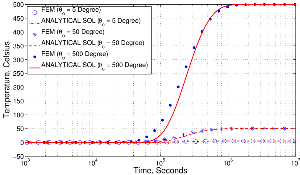
Figure 8.5: Comparison of the finite element solution and the analytical solution for three cases where \theta_o = 5, 50 and 500^{\circ}\text{C} .
