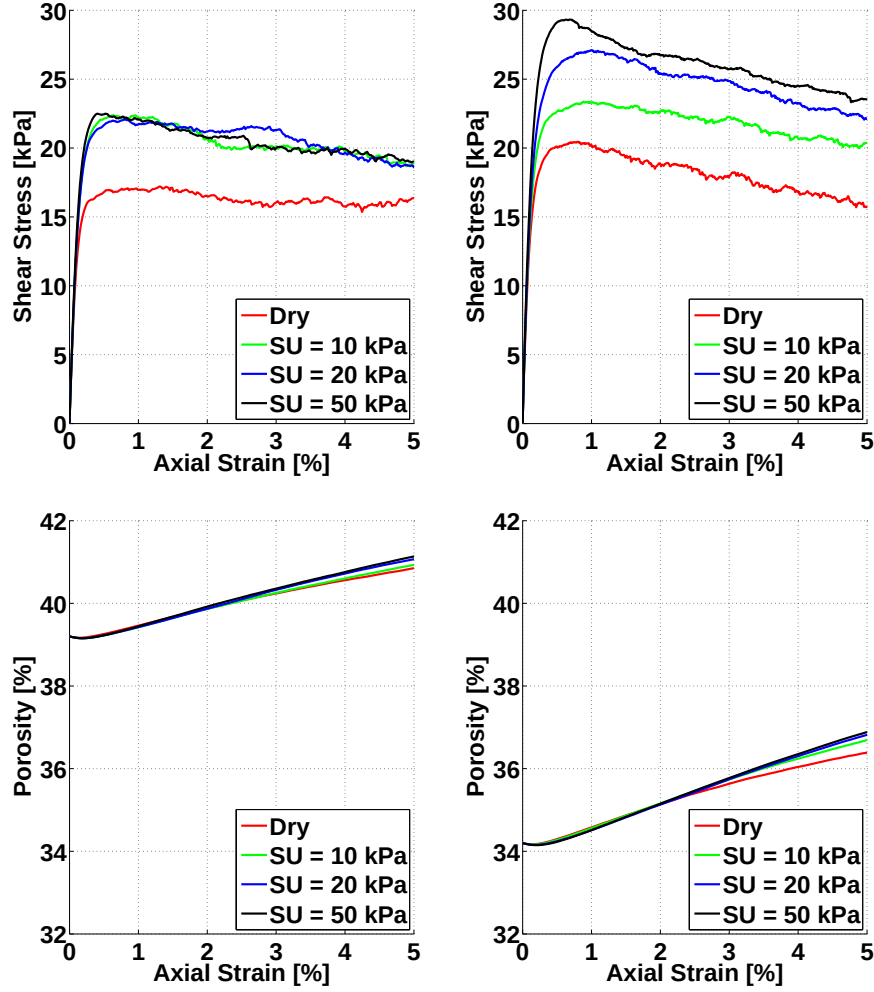
Figure 5.14: Shear stress and porosity versus axial strain curves with different suctions (SU) under constant confining stress 10 kPa. Left column: sample of coarse grains . Right column: mixture of coarse and fine grains
