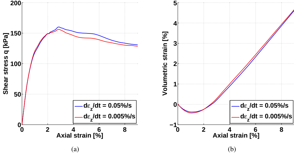
Figure 6.16: Global shear stress and volumetric strain behavior in globally drained triaxial compression test. Comparison of two loading rate.
