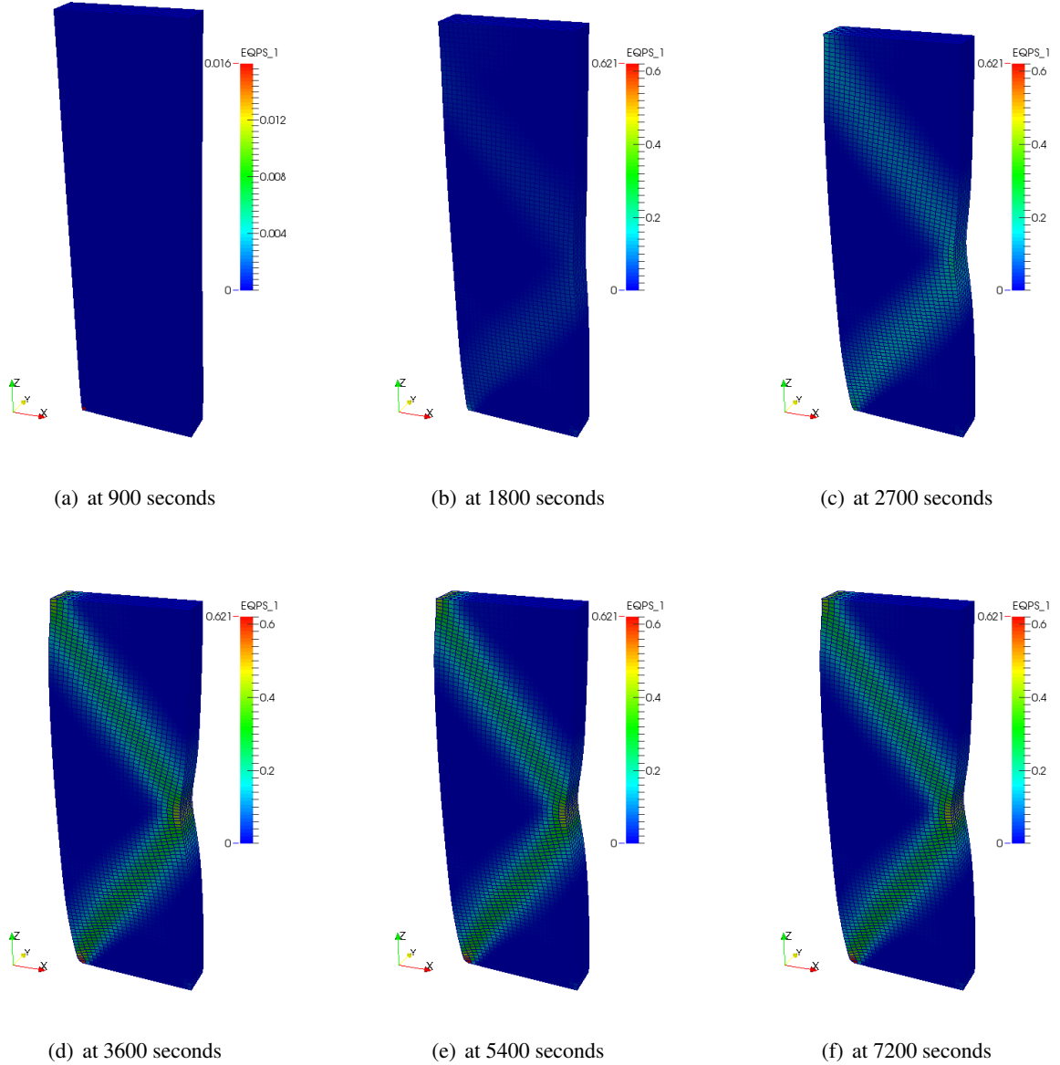
Figure 8.11: Equivalent plastic strain at various time during the biaxial loading test.
