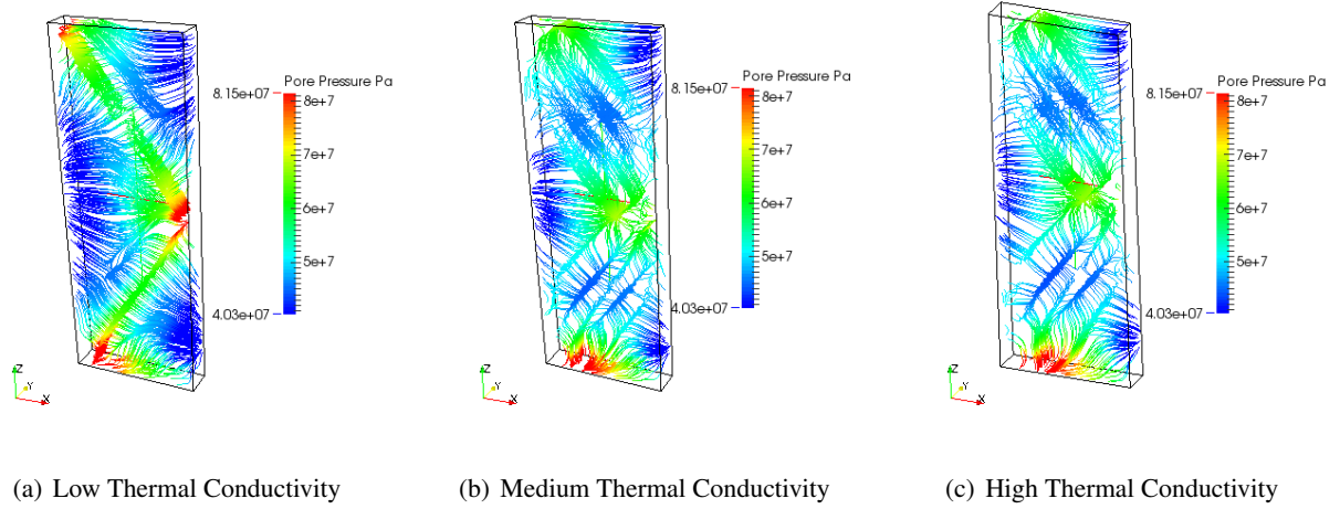
Figure 8.24: Flow streamlines at time = 7200 seconds, with initial effective thermal conductivity equals to (a) 0.013\text{W/m/}^\circ\text{C} , (b) 1.33\text{W/m/}^\circ\text{C} and (c) 133\text{W/m/}^\circ\text{C} .
