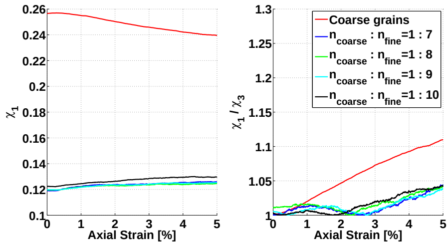
Figure 5.11: \chi_1 (left) and \chi_1 / \chi_3 (right) versus axial strain for samples of different amount ratios of coarse grains and fine grains n_{\text{coarse}} : n_{\text{fine}}
