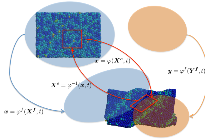
Figure 6.1: Trajectories of the solid and fluid constituents \varphi^s = \varphi and \varphi^f . The motion \varphi conserves all the mass of the solid constituent, while the fluid may enter or leave the body of the solid constituent. Figure reproduced from [Sun et al., 2013c]
