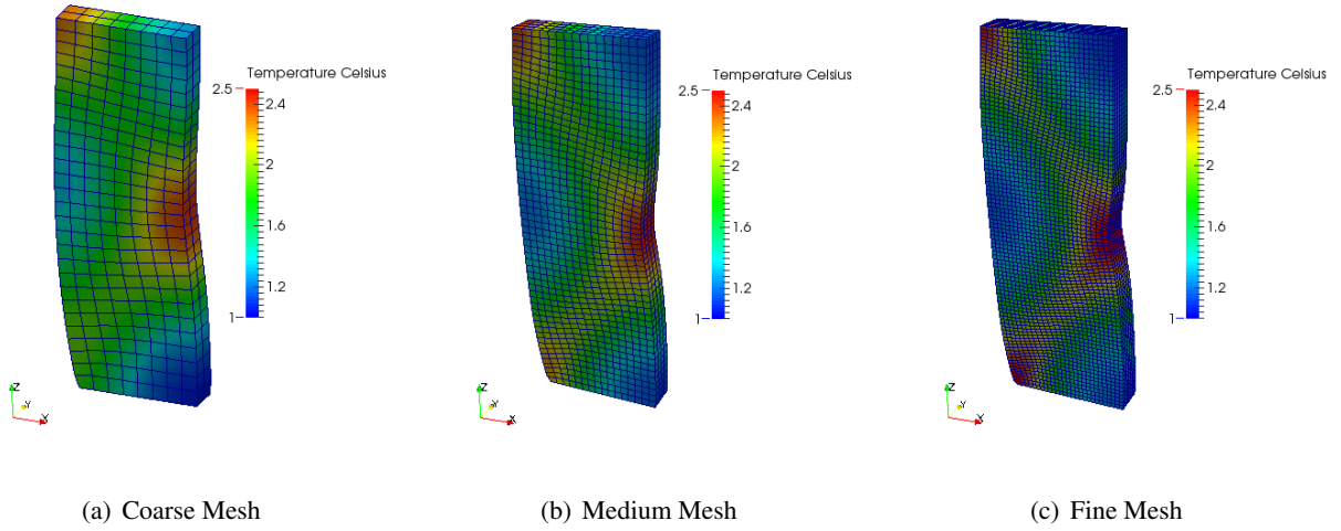
Figure 8.19: Temperature at t= 7200 seconds in three meshes.
