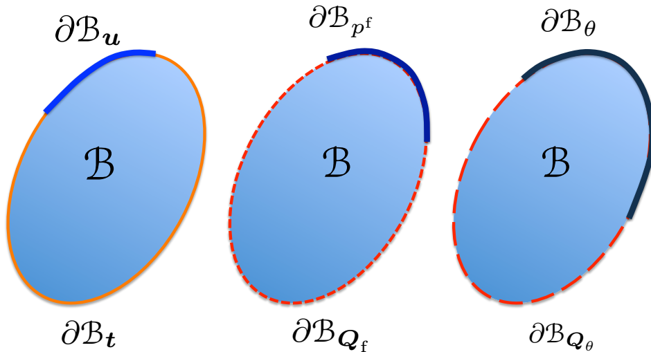
Figure 8.3: Domain and the corresponding boundaries of the thermo-hydro-mechanics problem. Figure reproduced from [Liu et al., 2009].
