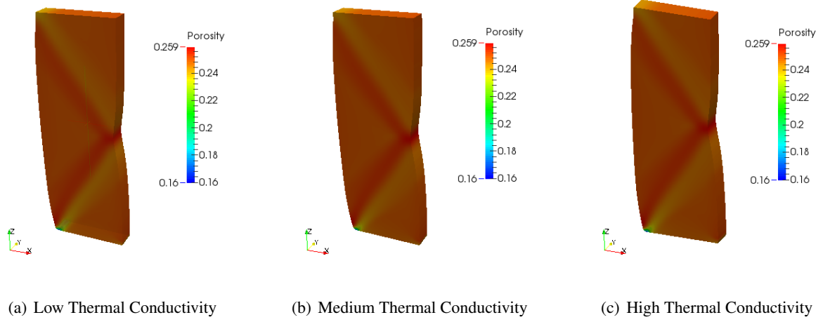
Figure 8.26: Porosity at time = 7200 seconds, with initial effective thermal conductivity equals to (a) 0.013\text{W/m}^\circ\text{C} , (b) 1.33\text{W/m}^\circ\text{C} and (c) 133\text{W/m}^\circ\text{C} .
