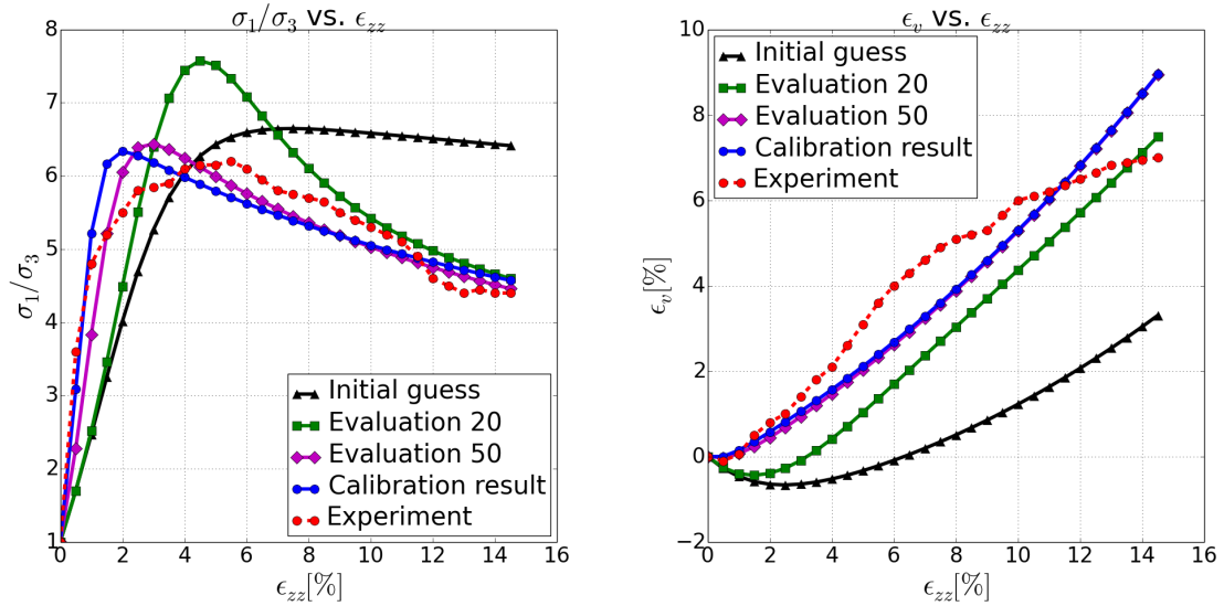
Figure 7.8: Macroscopic stress ratio (left) and volumetric strain (right) responses from selected value sets of material parameters in unit cell calibration
