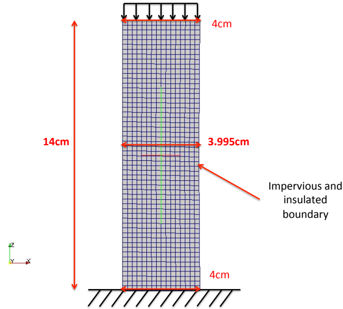
Figure 8.10: Description of the geometry, boundary and loading conditions of the bi-axial compression problem.
