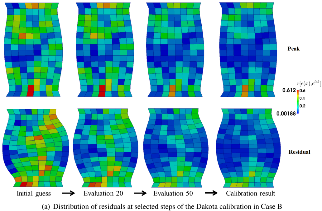
Figure 7.13: Relative error of local void ratio distribution between full sample simulation and micro-CT data (shown in cross-section in plane YZ) during Dakota calibration procedure using Case B: macroscopic responses and local void ratio distribution
