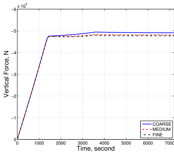
Figure 8.22: Time-history of vertical force on the top layer of the specimen.
