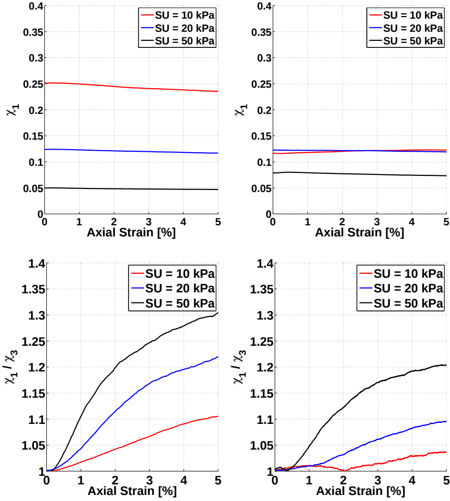
Figure 5.15: \chi_1 and \frac{\chi_1}{\chi_3} versus axial strain for sample of coarse grains (left column) and mixture of coarse and fine grains (right column)
