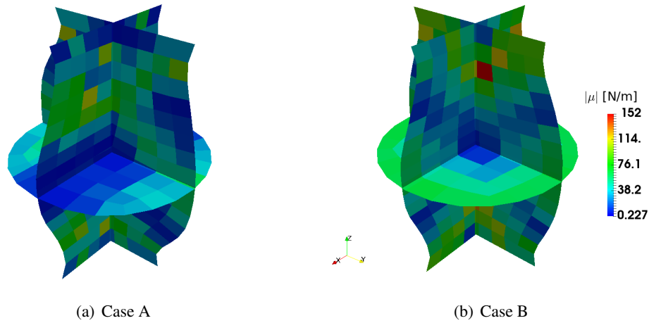
Figure 7.15: Norm of the couple stress tensor |\mu| = \sqrt{\mu_{21}^2 + \mu_{32}^2 + \mu_{31}^2} for results of inverse problems A and B at the residual stage.
