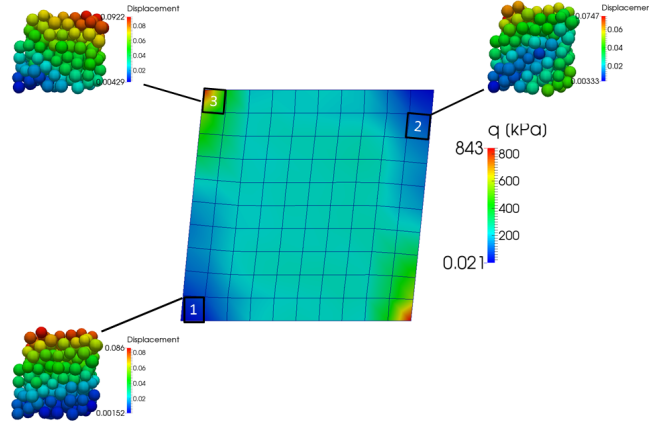
Figure 6.10: Spatial distribution of shear stress q at 10% shear strain for globally undrained dense sample allowing seepage within the specimen, attached with displacement magnitude of grains in unit cells (normalized by the initial cell size)
