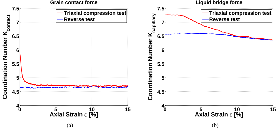
Figure 5.6: Evolution of the (a) coordination number of grain contact forces and (b) coordination number of liquid bridge forces along the triaxial compression test (red line, from left to right) and the reverse extension test (blue line, from right to left).
