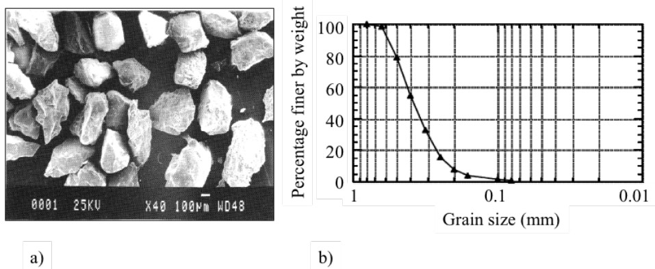
Figure 7.4: SEM image of Hostun sand from Flavigny et al. [1990] b) Grain size distribution of Hostun sand from Amat [2008]
