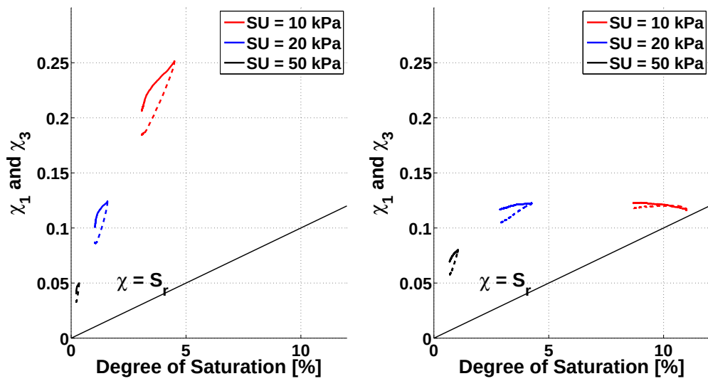
Figure 5.16: \chi_1 (solid lines) and \chi_3 (dashed lines) versus degree of saturation S_r for sample of coarse grains (left column) and mixture of coarse and fine grains (right column)
