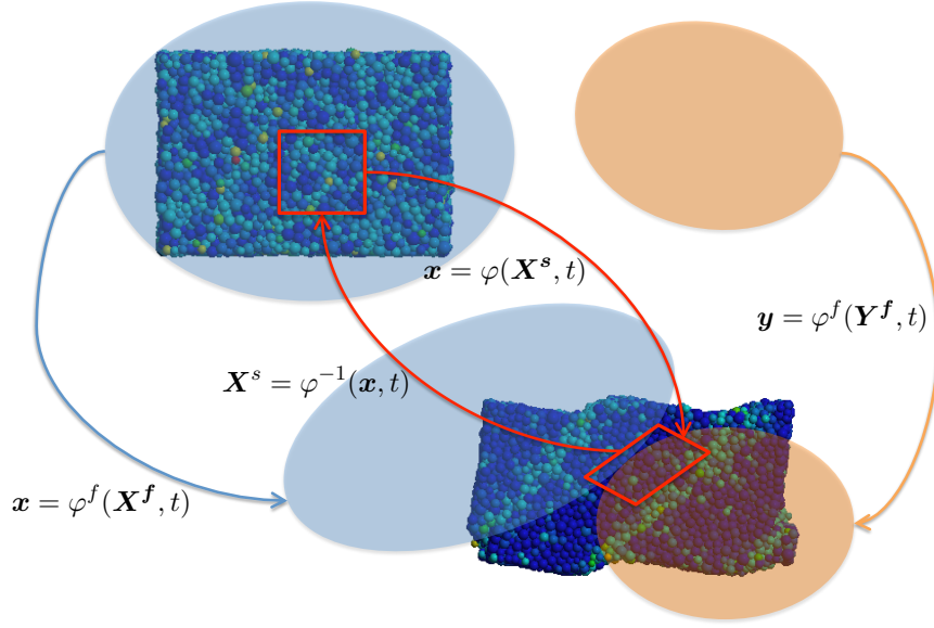
Figure 8.1: Trajectories of the solid and fluid constituents \varphi^s = \varphi and \varphi^f . The motion \varphi conserves all the mass of the solid constituent, while the fluid may enter or leave the body of the solid constituent. Figure reproduced from Sun et al. [2013c] .
