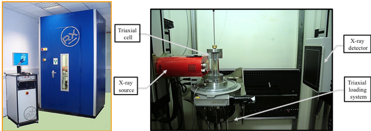
Figure 7.2: X-Ray CT scanner at Laboratory 3SR (left) and the whole arrangement of triaxial setup inside x-ray cabinet (right).
