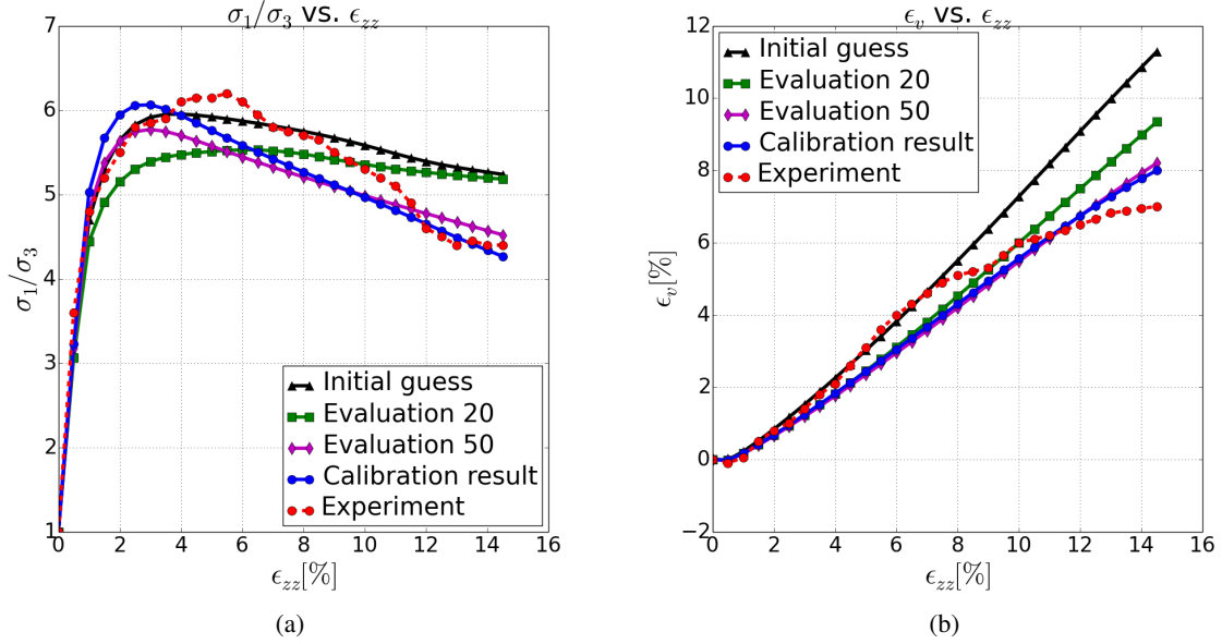
Figure 7.10: Stress ratio and volumetric strain responses of full sample simulation during the calibration procedure using only macroscopic responses (Case A).
