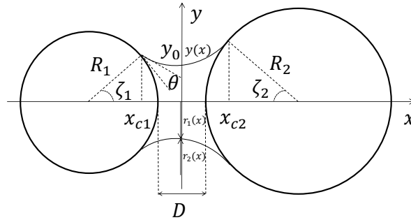
Figure 5.3: Liquid bridge model
