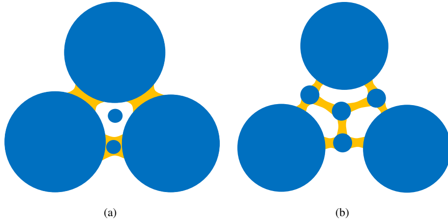
Figure 5.9: Inter-granular soil mix classification. Case (a): network dominated by coarse grain interactions with fine particles confined within void or between grains. Case (b): network dominated by fine grain interactions. The inter-granular distances are enlarged to show the network of liquid bridges.
