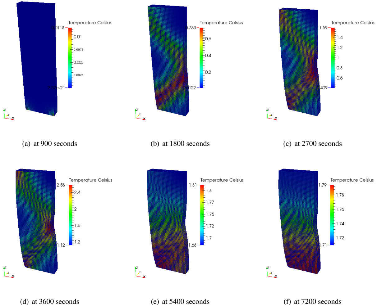
Figure 8.14: Temperature at various time during the biaxial loading test.
