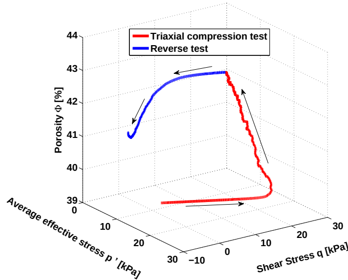
Figure 5.4: State path of the triaxial compression test and the reverse test. The arrows point at the loading direction.
