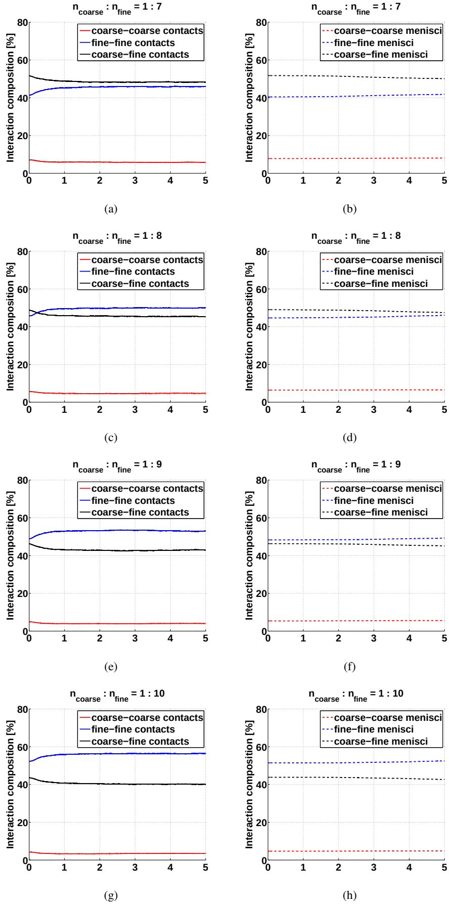
Figure 5.13: Evolution of interaction compositions versus axial strain for samples of different amount ratios of coarse grains and fine grains n_{\text{coarse}} : n_{\text{fine}}
