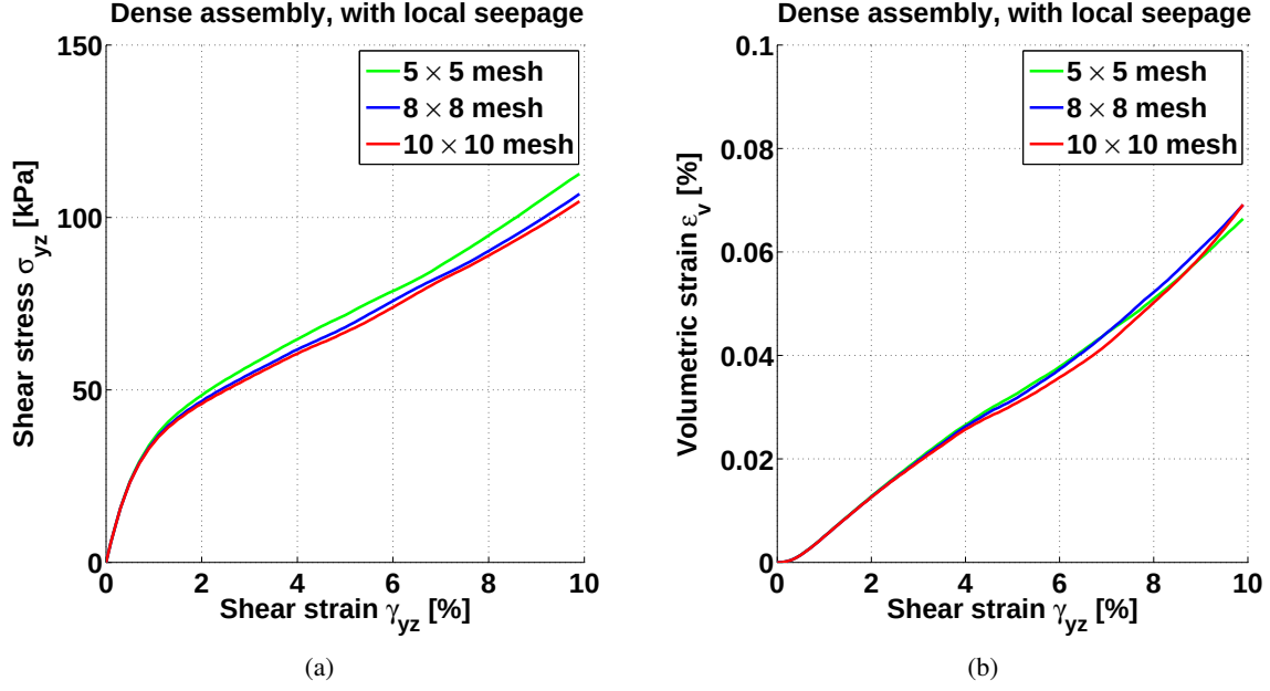
Figure 6.7: Comparison of global shear stress and global volumetric strain behavior between coarse mesh ( 1 \times 5 \times 5 ), medium mesh ( 1 \times 8 \times 8 ), fine mesh ( 1 \times 10 \times 10 ), finite strain formulation
