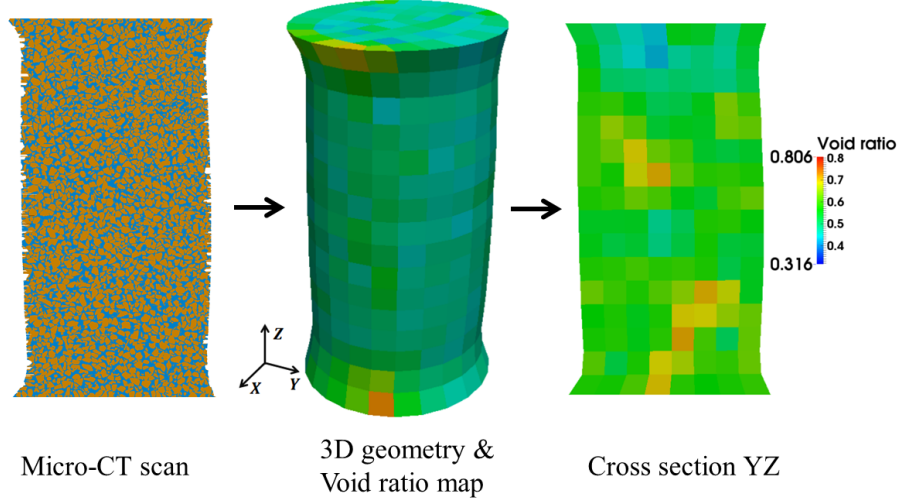
Figure 7.9: Construction of the numerical sample and void ratio distribution from micro-CT experimental data at the initial stage (0 % axial strain) of the triaxial compression test
