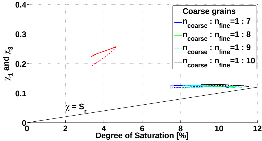
Figure 5.12: \chi_1 (solid lines) and \chi_3 (dashed lines) versus degree of saturation S_r for samples of different amount ratios of coarse grains and fine grains n_{coarse} : n_{fine}
