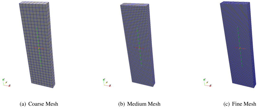
Figure 8.16: Mesher used in refinement study.
