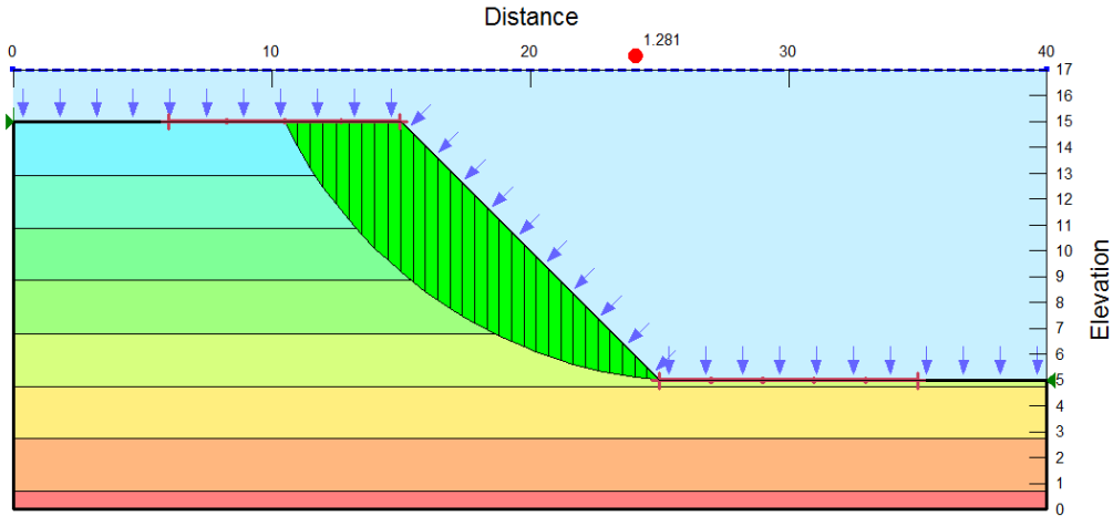
Figure 6.21: Slip surface and factor of safety of 1.281 estimated by SLOPE/W for a 1:1 submerged slope. The unit of the spatial dimensions is meter.
