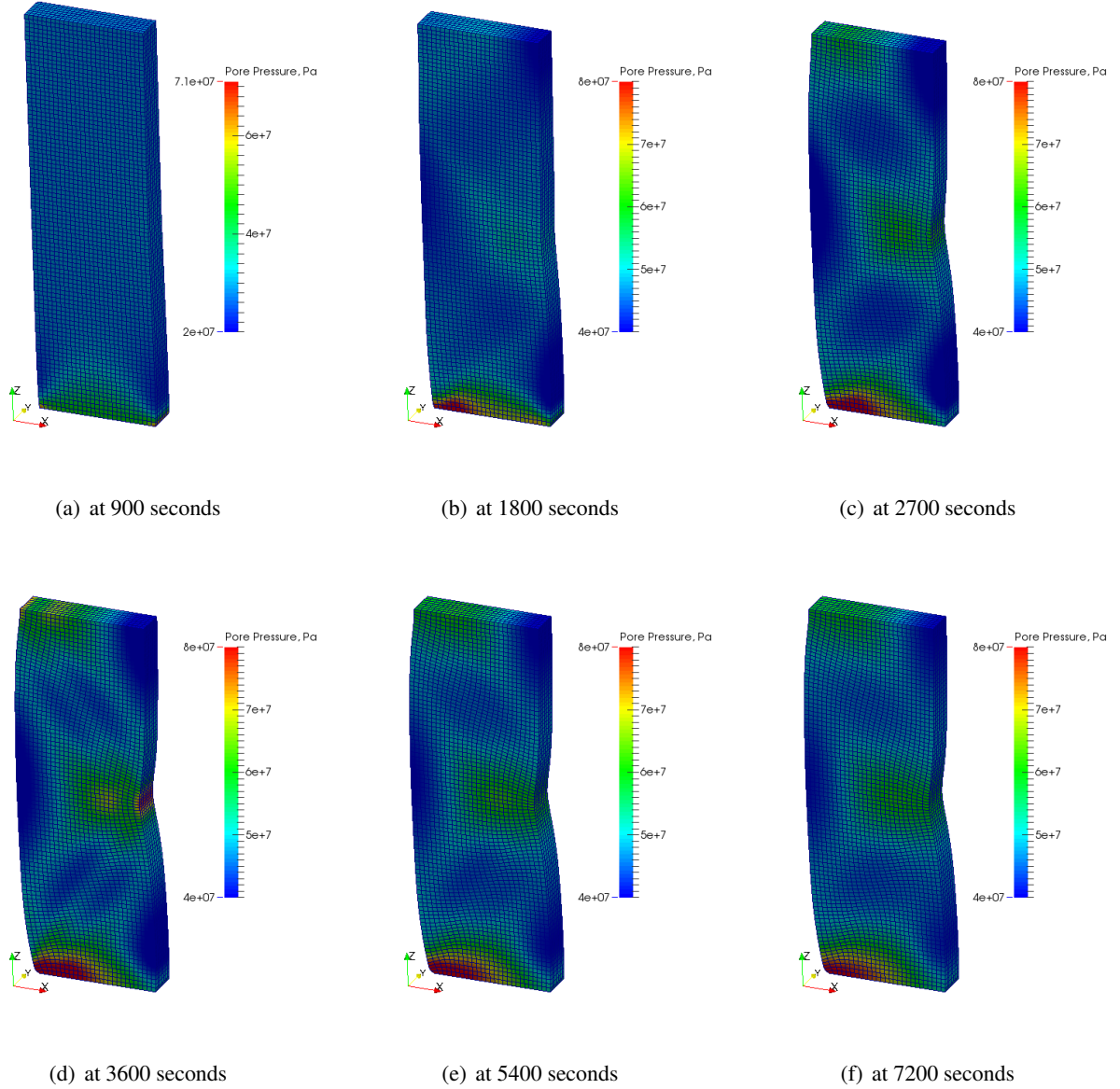
Figure 8.15: Pore Pressure at various time during the biaxial loading test.
