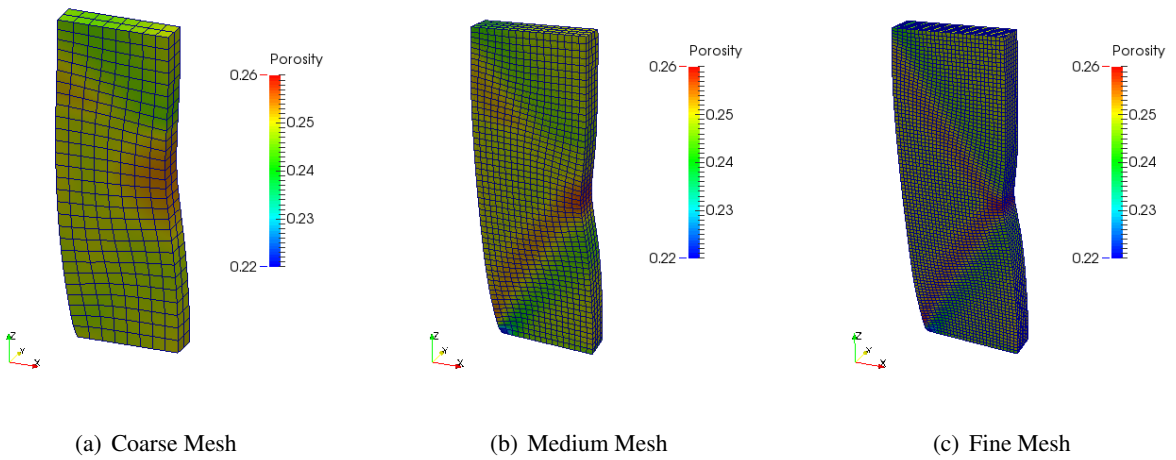
Figure 8.18: Porosity at t= 7200 seconds in three meshes.
