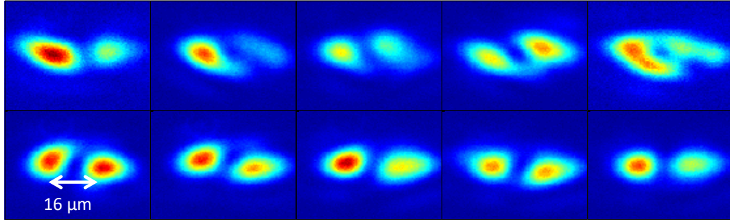
Figure 4.8. Series of guided modes at the exit of an 11 mm nitrogen plasma waveguide. The modes retain the two-lobe structure of the injected near- \text{TEM}_{01} mode with an energy throughput of \sim 30\% .
