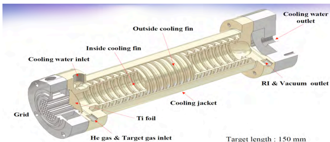
Figure 1: High pressure cell design for production of 11 CO 2 from N 2 :O 2 gas mixtures from a presentation by Hur. 1 The fins are devised to improve the surface area for convective heat transfer to the walls.
