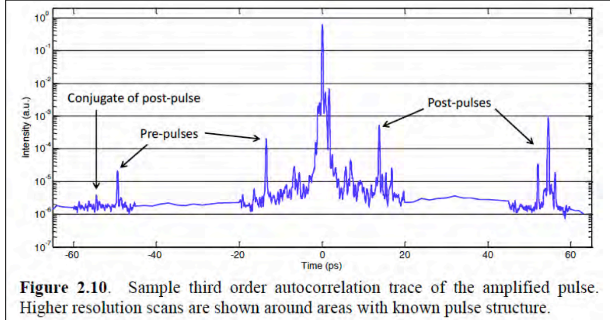
Figure 8: Pre- and post-pulse laser intensities. (Figure 2.10 in Appendix 1).
