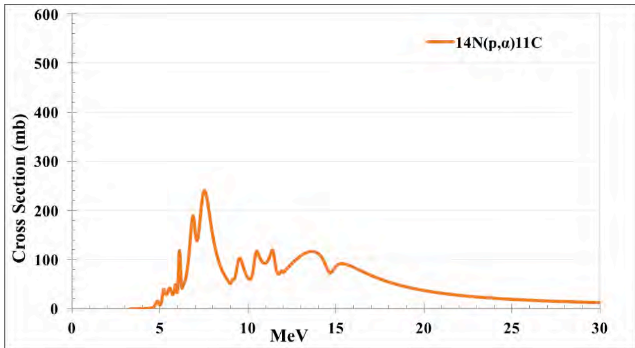
Figure 1: Cross section of ^{14}\text{N}(p,\alpha)^{11}\text{C} reaction as a function of proton energy
