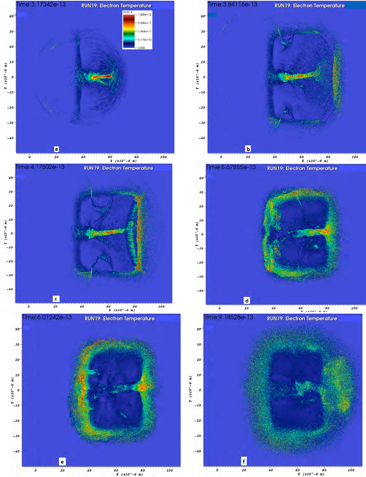
Figure 8: Figures a-d describe the dynamics and spatial distribution of hot electrons during the energy transfer from the laser to relativistic electrons. Figures e and f show the expansion of the multi-MeV electrons at the front of the target that controls the energy transfer from relativistic electrons to multi-MeV protons
