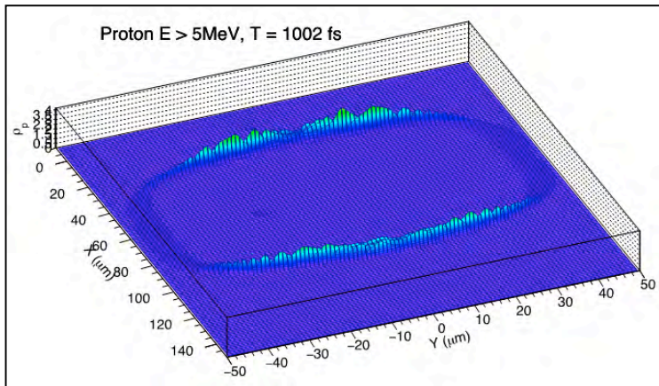
Figure 11: Proton density for E > 5 MeV and divergence angle smaller than 20^\circ
