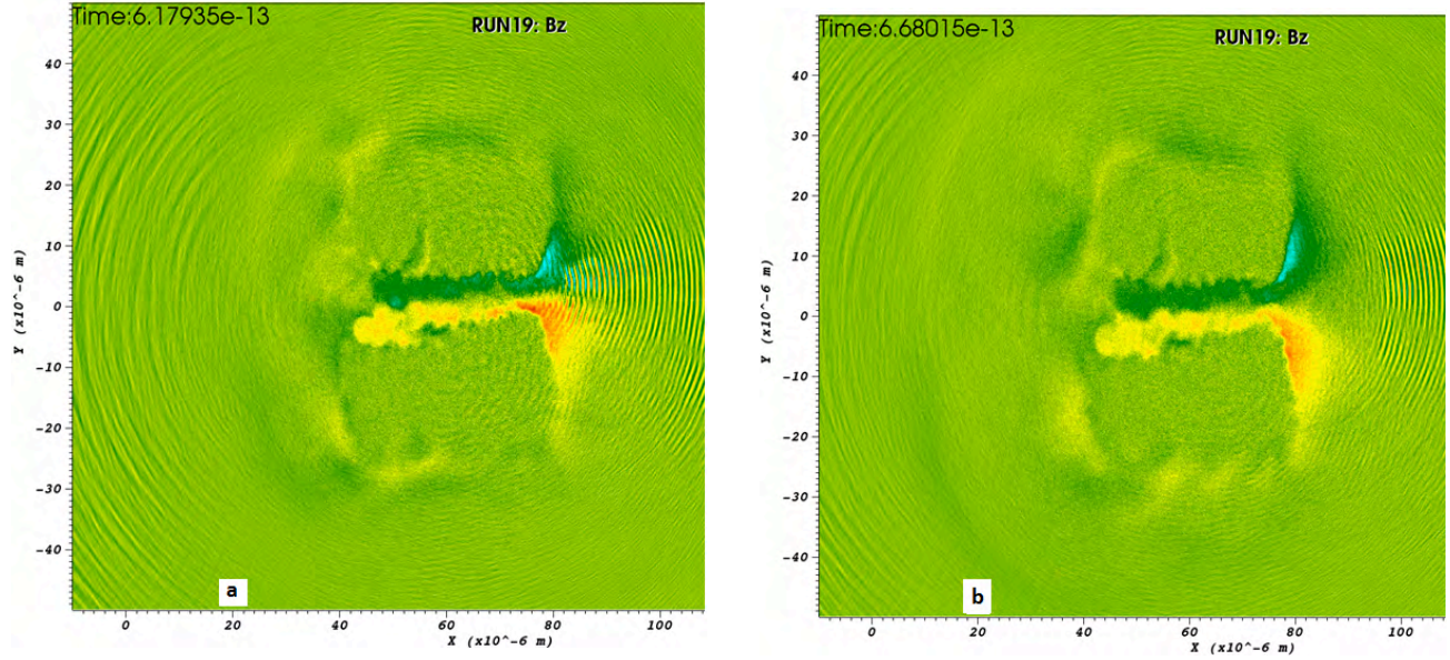
Figure 6: Quasi-static magnetic field in the z-direction following the depletion of the laser pulse energy. Notice that the fields persist to the end of the run.
