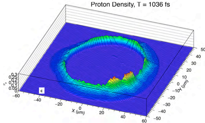
Figure 23: Proton acceleration signatures for the cylindrical plasma targets parameters of R15: (a) Volume averaged proton distribution function; (b) Proton phase space in the x-direction; (c) Two dimensional proton density for E > 3 MeV.
