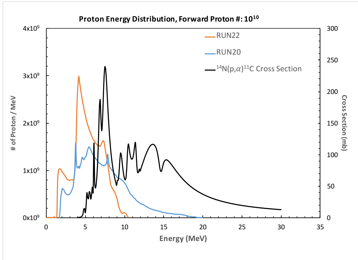
Figure 7: Ion energy distributions for a short pulse (RUN22: 50fs, 4 \times 10^{19} \text{W/cm}^2 and RUN20: 300fs, 2 \times 10^{19} \text{W/cm}^2 ) overlaid on the ^{11}\text{C} production cross-section. The rate of producing ^{11}\text{C} per proton is ten times larger for RUN20 than for RUN22.
