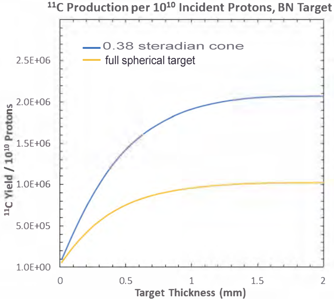
Figure 4: ^{11}\text{C} production rates normalized to the number of incident protons as a function of BN target thickness. The efficiency of the higher average energy of forward-directed protons in the quasi-neutral plasma jet is about twice as high in the smaller cone than in the full sphere.
