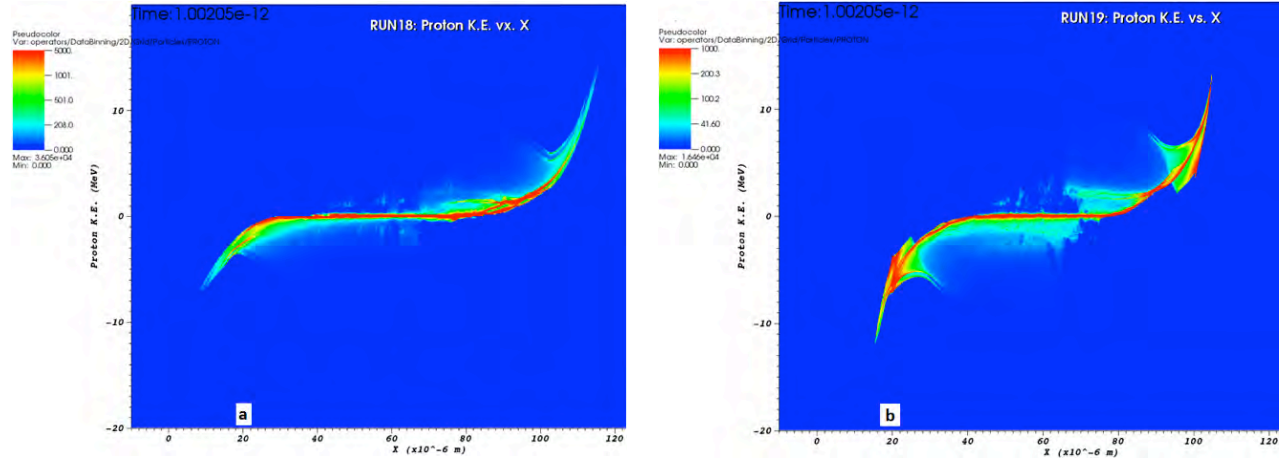
Figure 13: Phase space distributions for (a) R18 and (b) R19.
