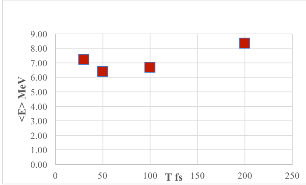
Figure 7: Average energy of forward collimated protons as a function of laser pulse length as a function of pulse length for at 3J per pulse.
