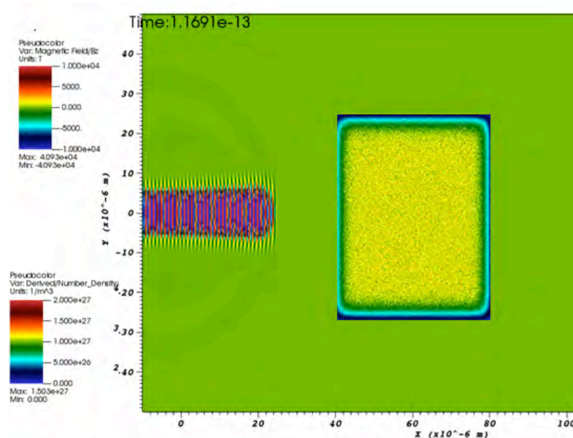
Figure 1: Simulation set-up. The laser pulse with Gaussian spatial and temporal profiles is introduced at the left boundary. The pulse propagates through free-space and enters the target at x=40 \mu m at t= .13 ps.
