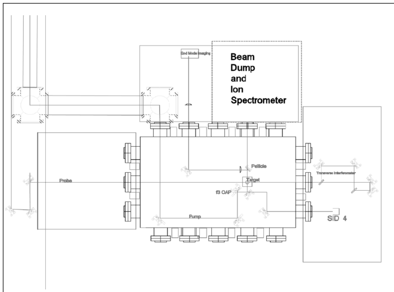
Figure 1: Top view of the proof-of-concept vacuum chamber. The expanded, high energy pulses enter the main chamber and are compressed by two gratings, then focused on the target by an off-axis parabolic mirror. Beam diagnostics, an interferometric probe for measurement of gas jet profiles, and a port for characterization of the proton fluxes and energies are also shown.
