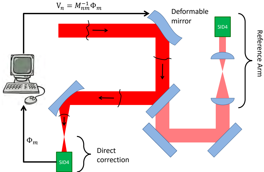
Figure 2.11. Schematic layout of an adaptive optics loop utilizing a reference arm for downstream aberration correction. First, a loop is closed with the SID4 behind the laser focus correcting the beam to a perfect diverging wave front. These mirror voltages are then used to obtain a reference wave front upstream of the final focusing optic. For daily operation, the loop is closed with the SID4 in this reference arm which corrects for aberrations in the full laser chain.
