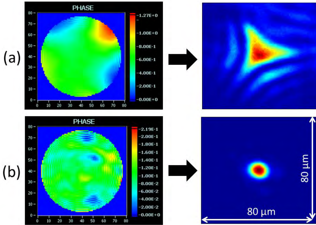
Figure 2.12. Measured laser wave front and focal spot before (a) and after (b) convergence of the adaptive optics loop. The phase measurements are in units of waves with \lambda = 800\text{nm} . The wave front curvature and tilts have been removed for clarity. The spatial scale is the same in both focal spot images though the color scales are individually normalized.
