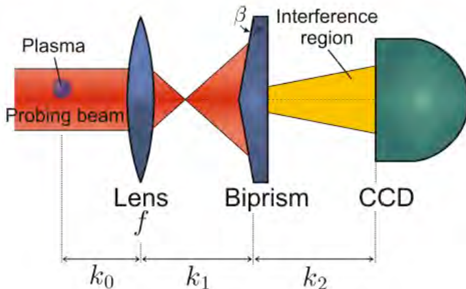
Figure 3. Schematic of the Nomarski interferometer with a Fresnel biprism as the wave front division optic. In our design k_0 = 90 \text{ mm} , k_1 = 170 \text{ mm} , k_2 = 280 \text{ mm} , f = 75 \text{ mm} , and \beta = 1^\circ . Image credit: Kalal et al. JKPS 56, 287 (2010).
