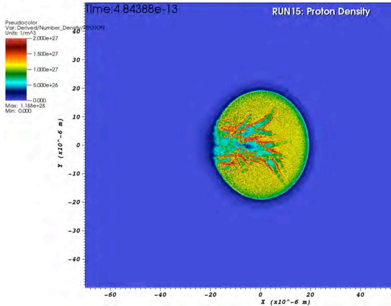
Figure 25: Filamentary plasma channel structure at t = .48 ps for R15 target parameters.
