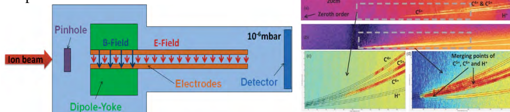
plasma of a carbon target (right) showing the parabolic trajectories and separation of ions with different q/m ratios. (From Cobble et al. 2 )
