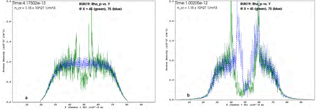
Figure 3: Line plots of the plasma density as a function of y at times t=.42 ps (a) and t=1 ps (b) at x=45 \mu\text{m} (green) and x=75 \mu\text{m} (blue). The figures indicate that plasma channel narrows with length and that the density of the channel walls reaches values of three times the critical density.
