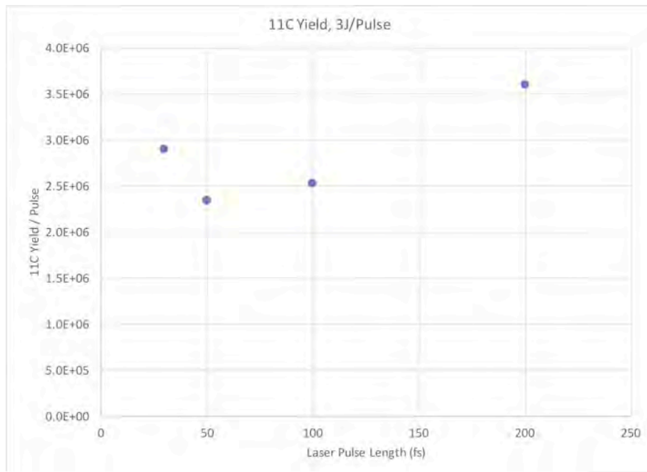
Figure 14: 11 C yield vs pulse length for 3J per pulse.
