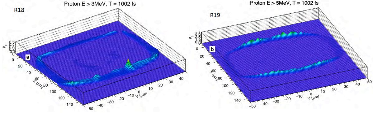
Figure 15: Two-dimensional proton density at t=1 ps for: (a) E>3 MeV protons in R18; (b) E>5 MeV protons in R19. Notice the hot spots in the R18 simulations corresponding to the location of hot electron temperature spots in Fig. 14a.
