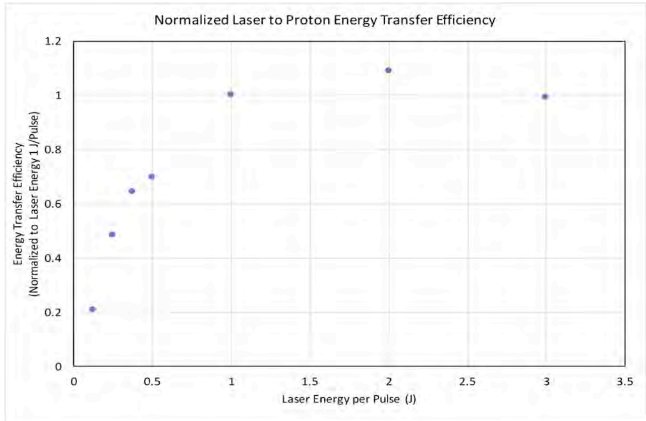
Figure 11: Relative laser-to-protons collimated forward efficiency as a function of energy per pulse, indicating optimal operation near 2J per pulse.
