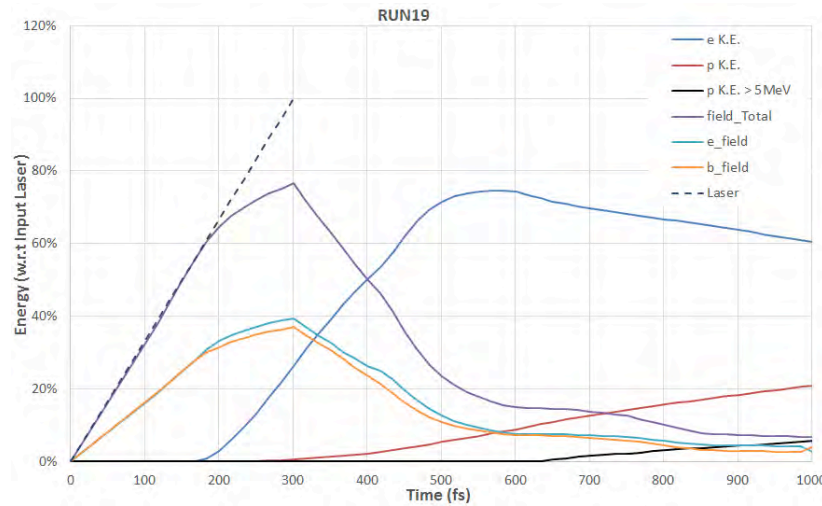
Figure 7: Temporal evolution of energy in key plasma and electromagnetic field components. Notice that energy transfer from the laser to relativistic electron heating is the dominant interaction till t = .6 ps, while energy transfer from relativistic electrons to protons in general and to protons with energy larger than 5 MeV at times t > .6 ps
