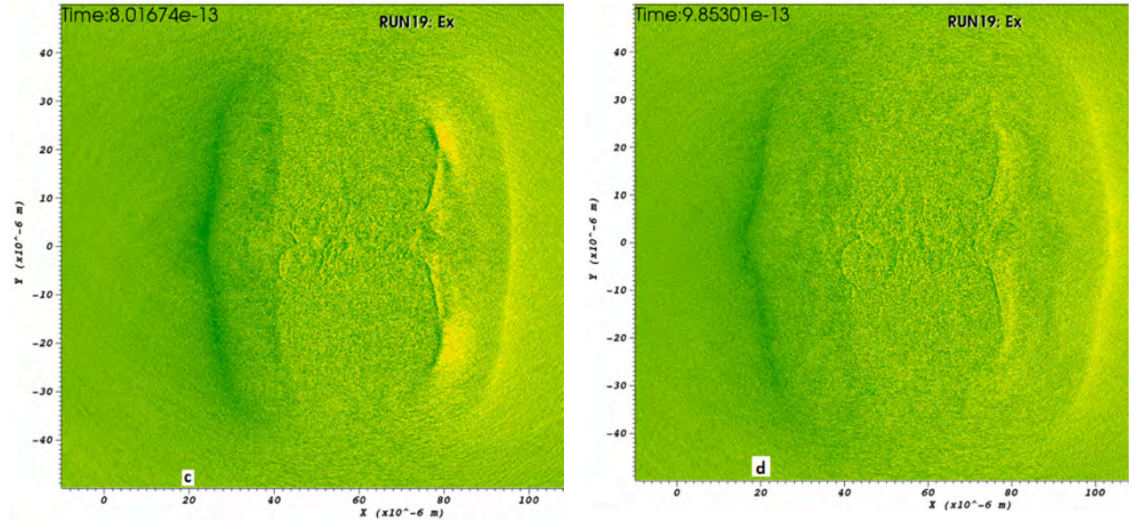
Figure 5: Temporal evolution of the quasi-static electric field ( E_x ) in two-dimensions. Notice that that they have planar structure and the dominant components are located near the front and the back of the target.
