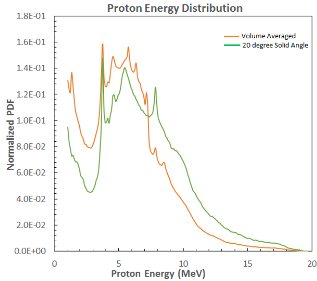
Figure 2a: Normalized ion energy distributions functions for collection in a .38 steradian solid angle oriented along the laser axis (green) and over the full sphere (orange).
