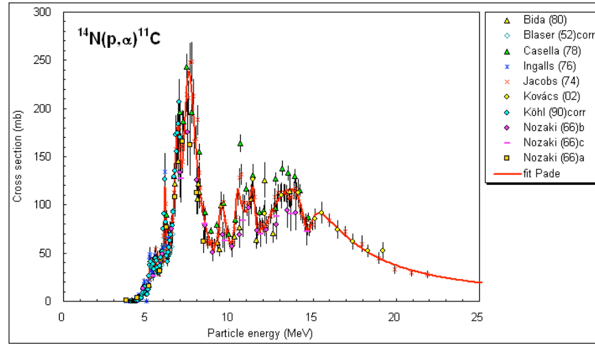
Figure 2: Recommended cross-section for production of ^{11}\text{C} from ^{14}\text{N} . 2
