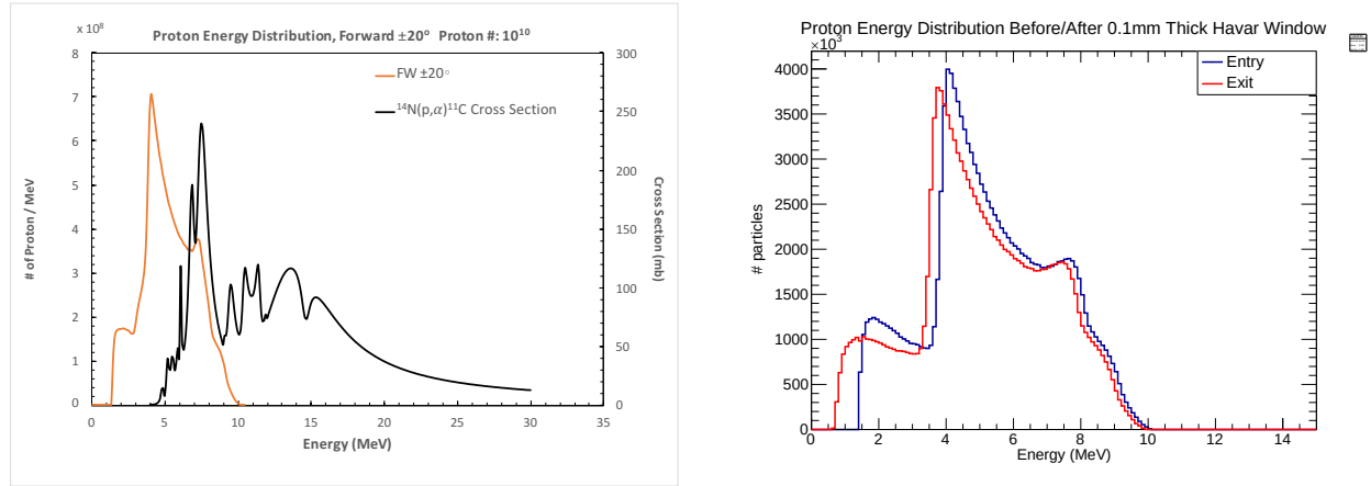
Figure 4: Proton energy distribution overlaid with the cross-section for ^{11}\text{C} production from ^{14}\text{N} (left) and its shifts on passing through 100 \mu\text{m} of Havar alloy (right).
