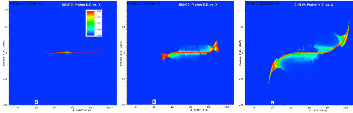
Figure 9: Proton phase space in the x -direction at: (a) t = .38 ps indicating acceleration only at the rear of the target; (b) t = .61 ps when proton acceleration at the rear and front side are approximately equal; (c) t = 1 ps showing that the acceleration at the front of the target dominates after t = .6 ps.
