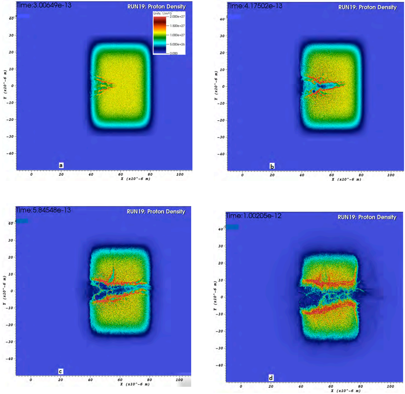
Figure 2: Temporal evolution of the plasma density in two-dimensions showing the formation of a plasma channel. Notice that the channel has a minimum size close to x=52 \mu\text{m} at t=.30 \text{ ps} corresponding to the focal point of the laser. The memory of the focusing can be seen in Fig. 2b at t=.42 \text{ ps} . The ponderomotive force of the laser results in a plasma channel that maintains its integrity throughout the simulation allowing the laser to propagate and deposit its energy to the electrons close to the target front.
