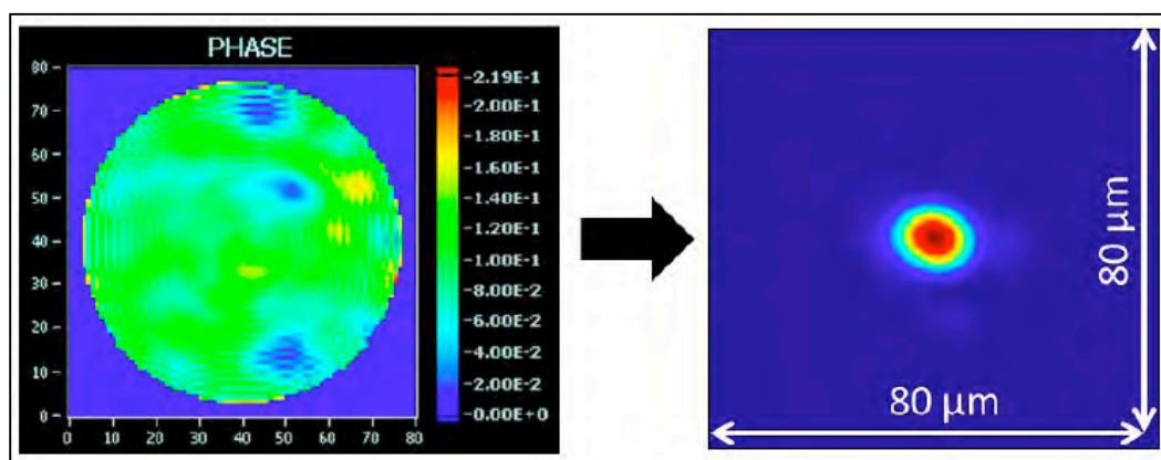
Figure 6: Measured phase front and focal spot for a ~40fs, 800nm pulse. (Appendix figure 2.12 for details).
