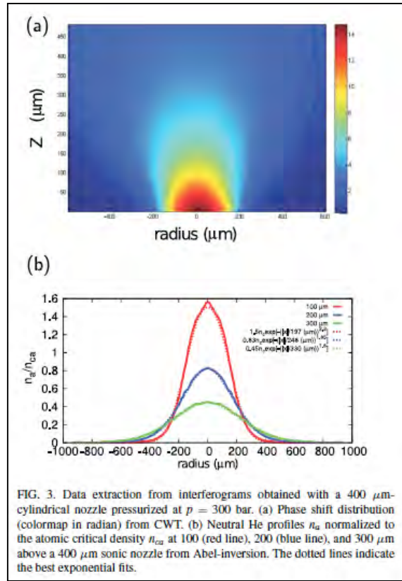
Figure 1: Figure 3 from reference (1) showing the spatial density profile of He gas with stagnation conditions of 20^{\circ}\text{C} and 30 MPa. The scale on the lower panel is in terms of n_{ca}=1.68 \times 10^{21} \text{ cm}^{-3} .
