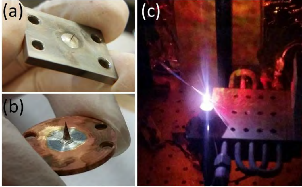
Figure 5.1. Custom fabricated straight (a) and tapered (b) nozzles with \sim 100\ \mu\text{m} throats. The gas jet is held in a custom cooling block (c) which can cool the jet to cryogenic temperatures.
