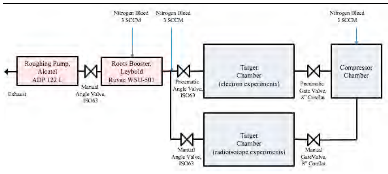
Figure 2: Layout of the vacuum system. The chirped laser pulse is compressed in a separate, valved chamber through which nitrogen is flowed at a few standard \text{cm}^3 per minute. Two target chambers are connected to a roots blower backed by a roughing pump. The continuous nitrogen bleed rigorously prevents backflow of oil vapor from the pumps and sweeps any adsorbed contaminants from the optics.
