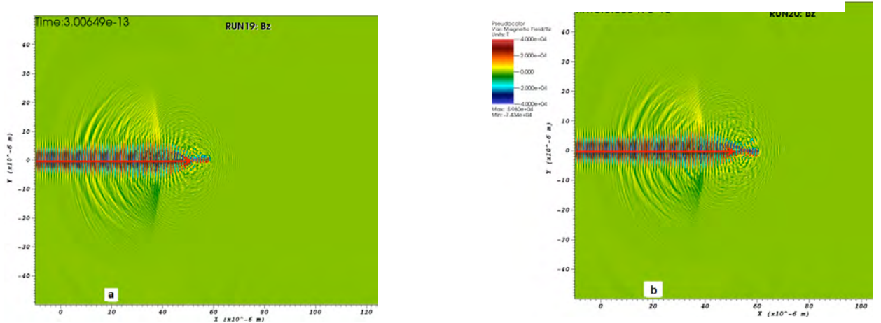
Figure 20: Spatial structure of laser pulse at time t = .3 ps for: (a) R19; (b) R20. It shows that the focal point (marked by the red arrow) for R19 occurs closer to the target entrance than for R20.
