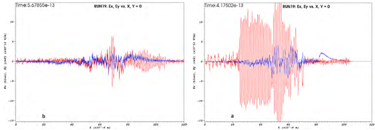
Figure 4: Line plots along of the laser field E_y (red line) and the electrostatic field E_x (blue line) at times t=.42 ps (a) and t=.57 ps (b). Spike-like E_x fields with alternating polarity and amplitude \text{MV}/\mu\text{m} are generated behind the laser front. These fields are responsible for electron heating and dissipation of the laser power. Starting at t=.42 ps an electrostatic field along the x -direction develops between 80-90 \mu\text{m} . In
