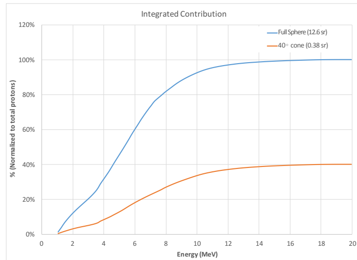
Figure 3: The contribution of ions with various energies to the production of ^{11}\text{C} showing that 40% of the useful yield is concentrated in 3% of the total solid angle.
