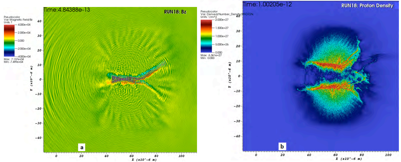
Figure 16: Consequences of filamentation resulting in poor matching of the laser to the plasma waveguide seen in: (a) laser guidance in filamentary channels; (b) formation of unmatched plasma channel as compared to Fig. 2 describing R19.
