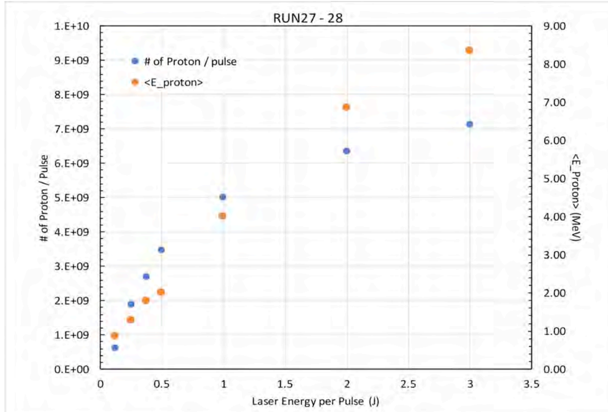
Figure 10: Average energy per proton and number of energetic proton collimated in the forward direction as a function of energy per pulse. The slope of the proton yield changes abruptly above \sim 1 J per pulse.
