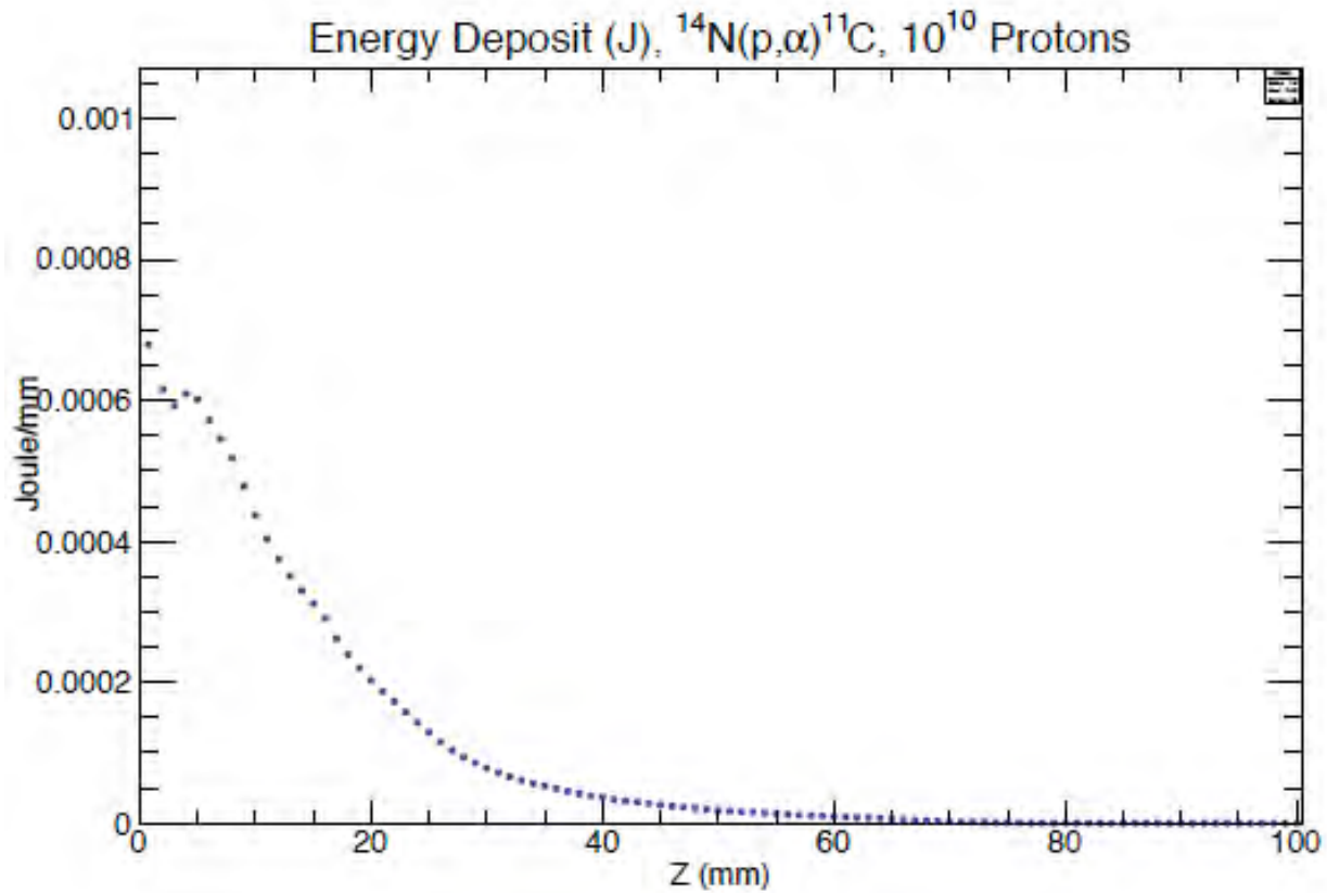
Figure 6: Energy deposition in 100 bar pressure \text{N}_2 gas from the quasi-neutral jet produced by the 50fs pulse described previously.
