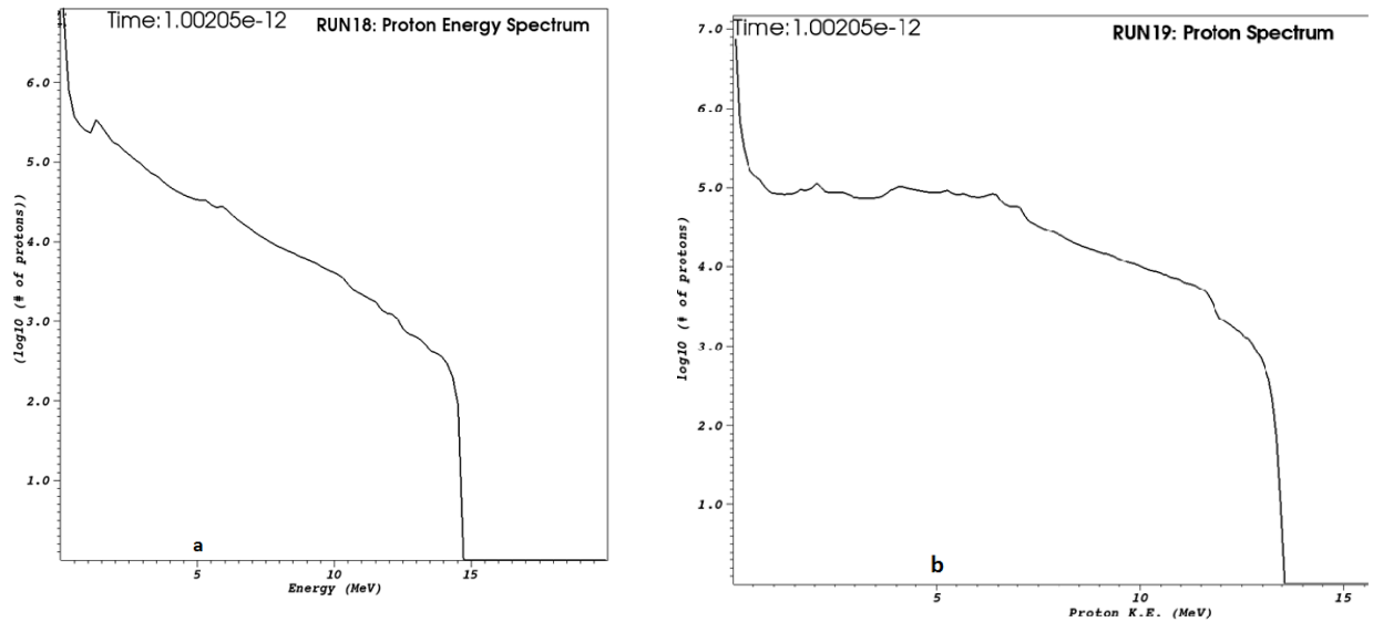
Figure 12: Proton energy distribution function averaged over the simulation volume for: (a) R18; (b) R19.
