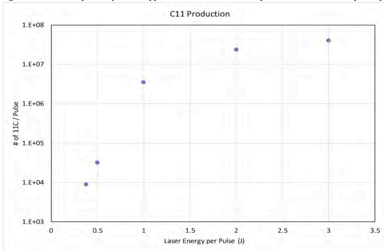
Figure 12: Scaling of C11 production yield with the energy per pulse. Notice similarity with the scaling of the average energy shown in Figure 4.
