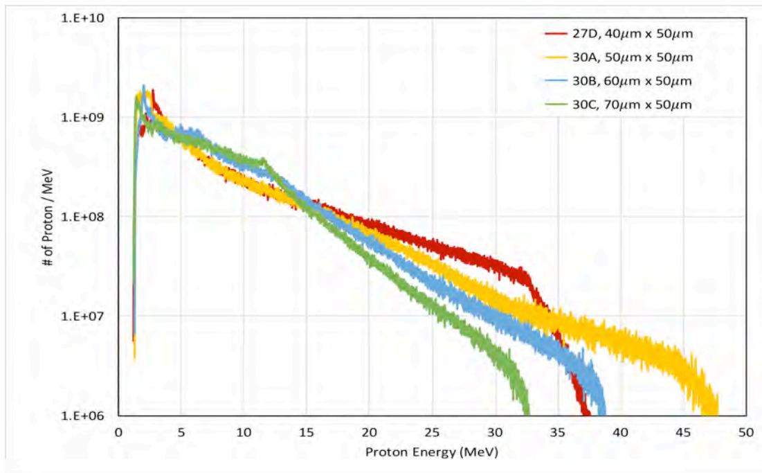
Figure 6: Forward collimated proton distribution functions for 3J energy per pulse, T = 200 fs but L = 40\text{-}70 \mu\text{m} .
