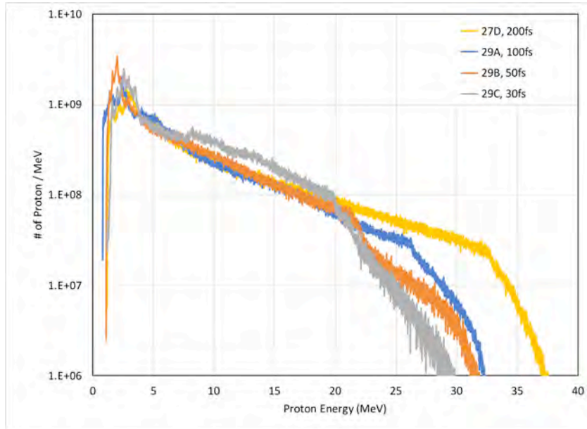
Figure 8: Forward collimated proton distribution function for 3J energy per pulse, L=40 mm, D=50 mm for pulse lengths 30, 50, 100 and 200 fs, corresponding to values of a=19.6, 15.2, 107 and 7.6 . Contrary to the conventional wisdom optimum distribution is obtained at 200 fs with a=7.6 .
