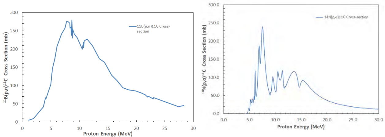
Figure 1: Cross sections ( 1\text{mb} = 10^{-31}\text{m}^2 ) for production of ^{11}\text{C} from ^{11}\text{B} (left) and ^{14}\text{N} (right).
