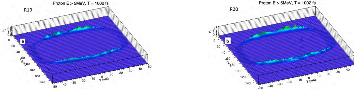
Figure 19: Two-dimensional proton density for E > 5 MeV at t = 1 ps for: (a) R19; (b) R20.
