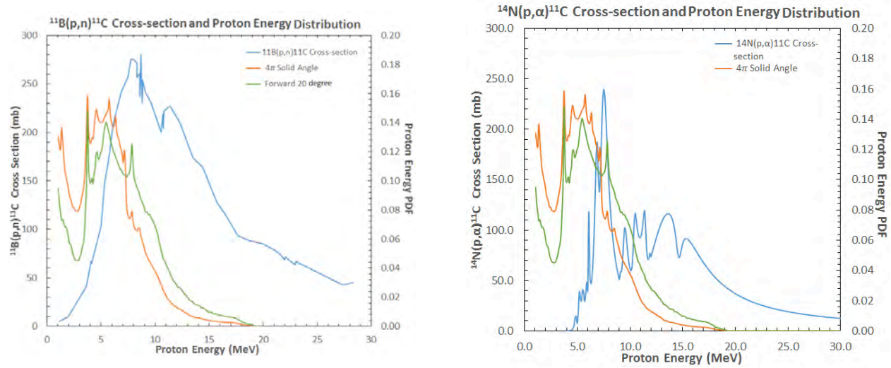
Figure 2b: The energy distribution of forward-directed protons (green) has better overlap with cross-sections for ^{11}\text{B} and ^{14}\text{N} and therefore greater efficiency for conversion to ^{11}\text{C} than the spatially average flux (orange).
