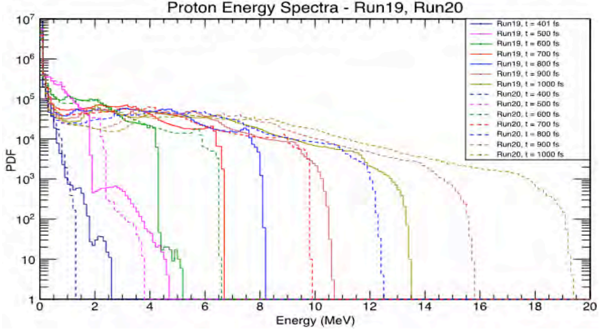
Figure 17: Temporal evolution of proton energy distribution function averaged over the simulation volume for R19 and R20 simulation runs indicating the greater efficiency of the subcritical R20 simulation parameters.
