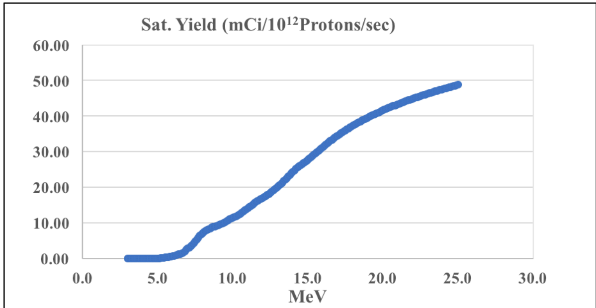
Figure 3: Saturation Yield of the ^{14}\text{N}(p,a)^{11}\text{C} reaction as a function of proton energy.
