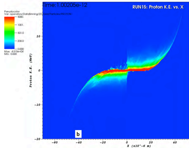
Figure 23: Proton acceleration signatures for the cylindrical plasma targets parameters of R15: (a) Volume averaged proton distribution function; (b) Proton phase space in the x-direction; (c) Two dimensional proton density for E > 3 MeV.
