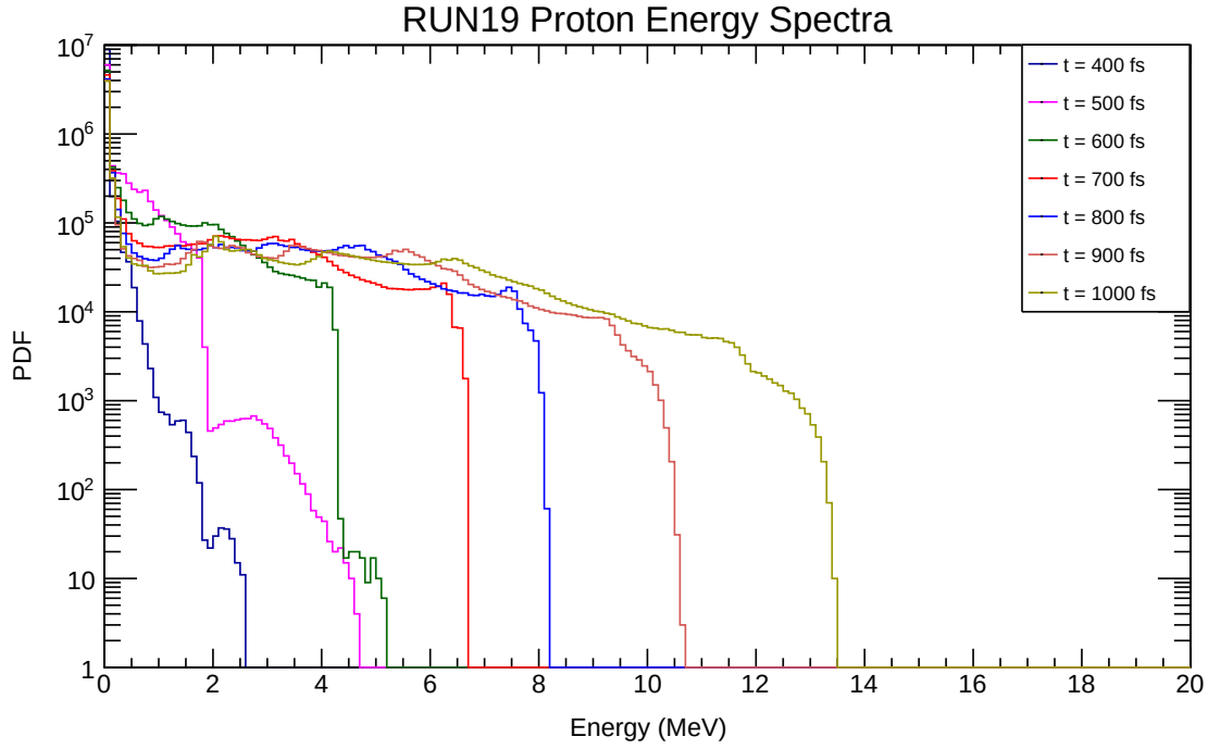
Figure 10: Temporal evolution of the proton energy distribution averaged over the simulation space.
