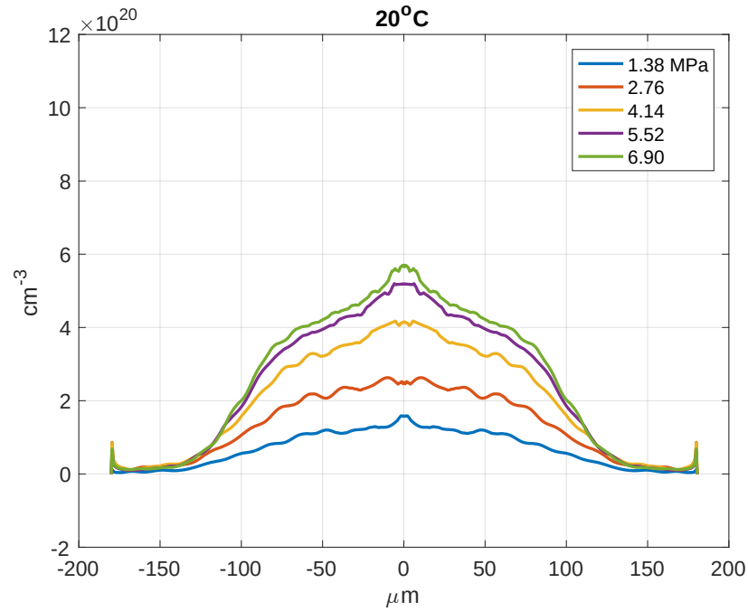
Figure 3: H_2 number density profiles 50\text{ }\mu\text{m} from the exit plane of a room temperature jet with stagnation pressures from 1.4 to 6.9 MPa (200 to 1000 psi) emerging from a 160\text{ }\mu\text{m} nozzle. The density of atoms in the laser driven plasma are twice these values.
