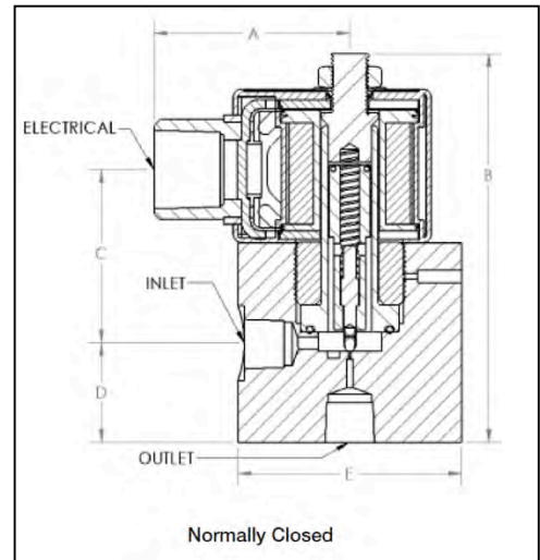
Figure 4: Cross-section of the 7 MPa EH30 valve planned for jet experiments.
