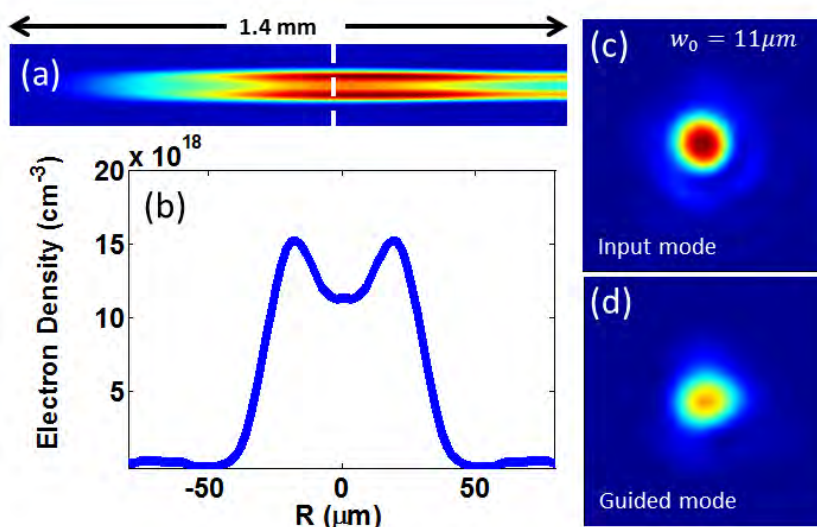
Figure 4.7. The Abel inverted density profile of the first 1.4 mm of an 11 mm nitrogen plasma waveguide (a) with a lineout shown in (b). A Gaussian input mode with an 11 \mu\text{m} spot size (c) is guided with approximately 60% energy throughput and the same spot size as the input mode (d).
