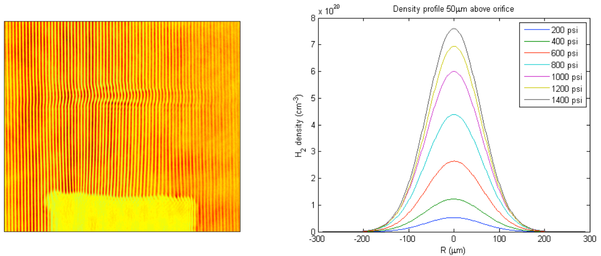
Figure 4: (left) 266 nm interferogram ( 400 \mu\text{m} edge lengths) of a transient plasma illustrating control of the fringe spacing for resolution of the plasma density profile. (right) Neutral density profile as a function of stagnation pressure at room temperature 50 microns in front of a 130 micron diameter nozzle extracted from a series of 400 nm interferograms. References
