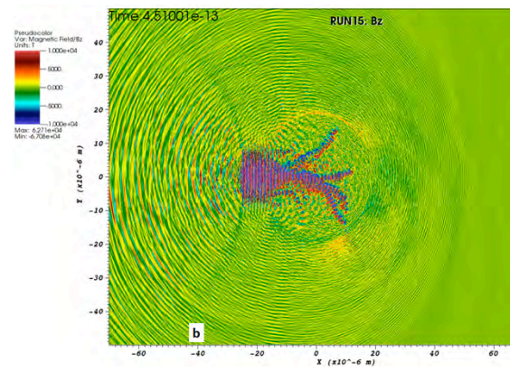
Figure 24: Laser pulse interaction with plasma target for R15 at (a) t = .23 ps; (b) t = .45 ps. Strong filamentation starts early and is completely developed by t = .45 ps.
