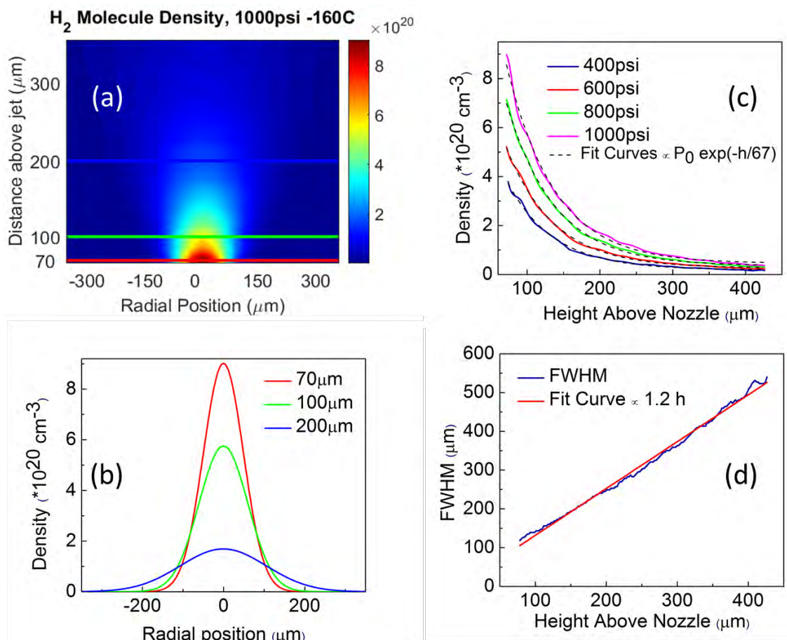
Figure 5.3. Sample 2D hydrogen molecule density profile (a) with 1000 psi backing pressure and -160° C reservoir temperature and lineouts 70, 100, and 200 μm above the nozzle (b). The peak density as a function of height decays exponentially (c) and the FWHM increases linearly with height above the jet (d).
