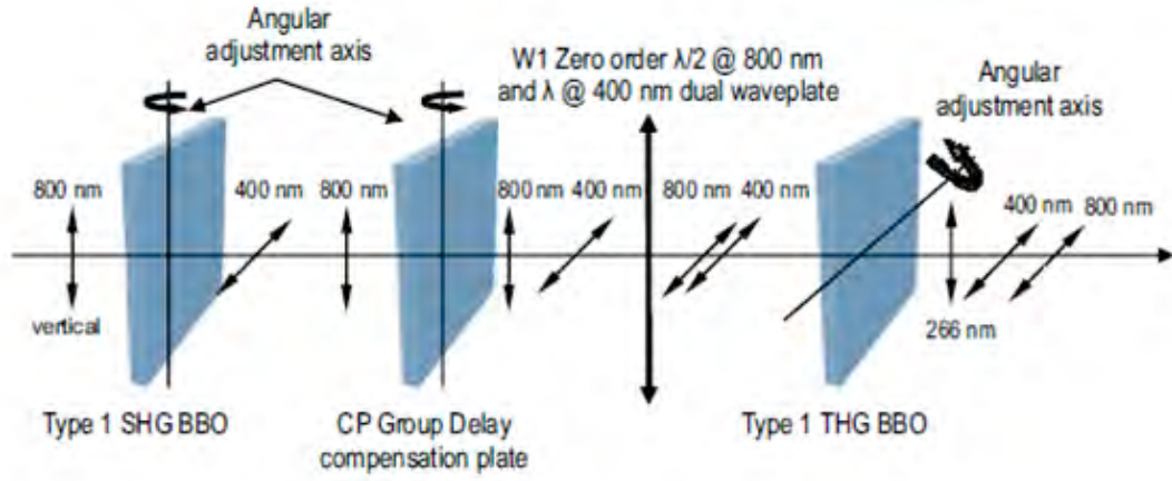
Figure 2. Schematic of the frequency tripling apparatus showing the polarization of the pulses as they travel through the assembly. Image credit: Eksma Optics www.eksmaoptics.com
