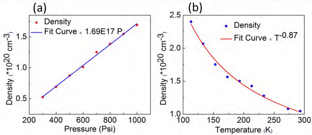
Figure 5.5. Peak jet density 200 \mu\text{m} above the 100 \mu\text{m} needle nozzle as a function of valve backing pressure at a fixed reservoir temperature -160° C (113 K) (a) and as a function of reservoir temperature at a fixed backing pressure 1000psi (b).
