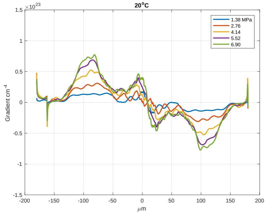
Figure 4: Room temperature density gradients for the profiles shown in the preceding figure. Systematic control of the gradients at the boundary is accomplished through adjustment of the stagnation pressure.
