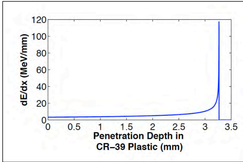
Figure 2: Energy loss in CR-39 for a 20 MeV proton with a Bragg Peak at 3.25 MeV.
