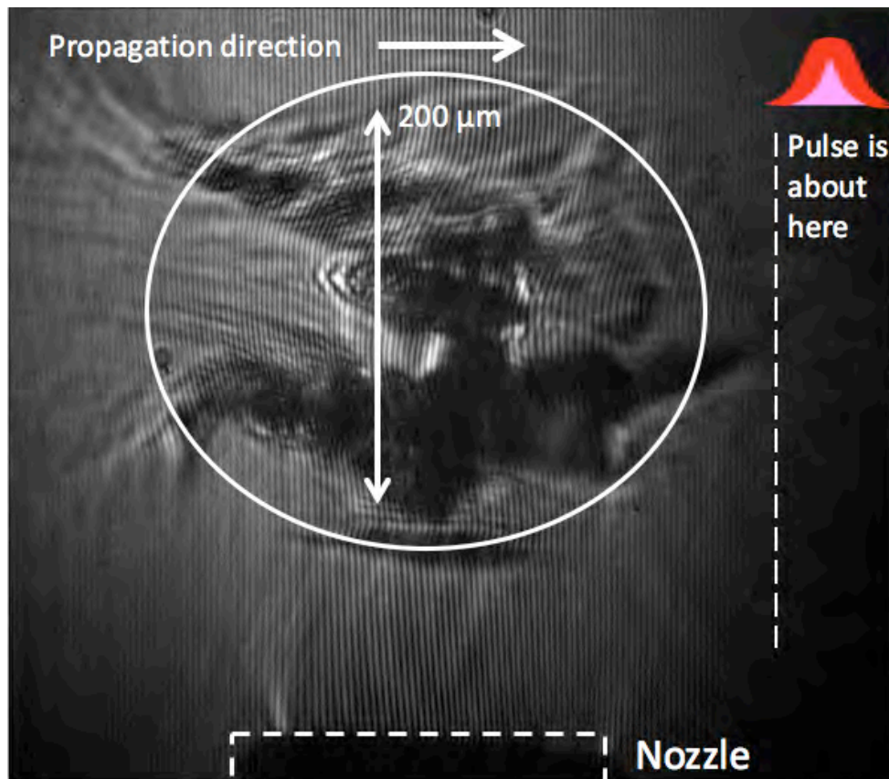
Figure 8: Interferometric image (266nm) of a transient hydrogen plasma ( -165^\circ\text{C} , 7MPa stagnation conditions) using a 500mJ, 400fs, 800nm laser pulse.
