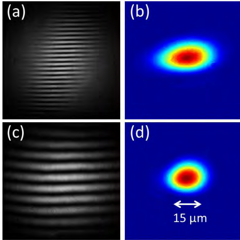
Figure 2.14. Inverted field autocorrelation traces before (a) and after (c) correction of a 0.5 \mu\text{rad/nm} angular chirp on a 39 fs pulse. The focal spot before (b) the correction is elliptical and becomes much more symmetric after improvement of the grating parallelism (d).
