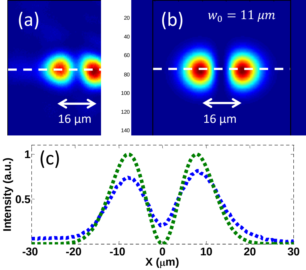
Figure 4.6. The focus of the half-pellicle beam (a) resembles a pure \text{TEM}_{01} Hermite-Gaussian mode (b). Lineouts along the maxima are compared in (c).
