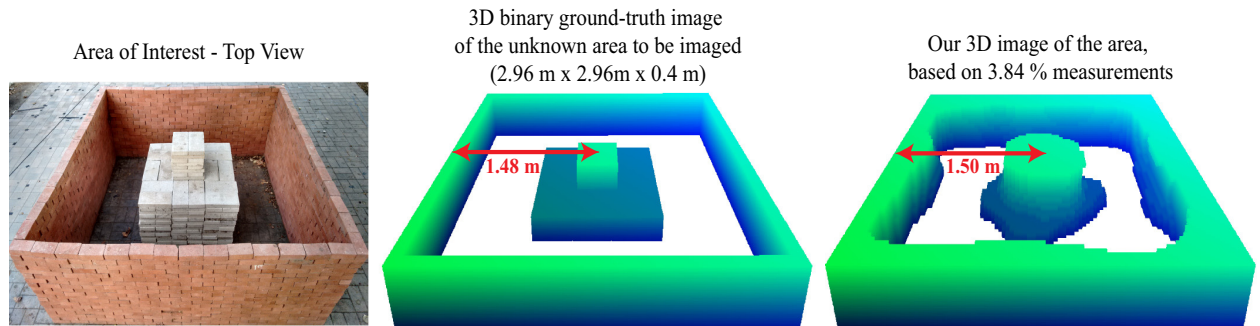
Figure 3: 3D robotic imaging through walls with on-board WiFi signals.
