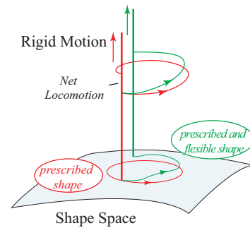
Figure 2: Geometric picture underlying undulatory locomotion.
