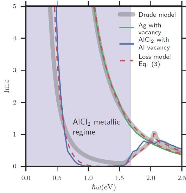
Fig. 10 Defect induced optical losses and energy-dependent relaxation time model. The calculated optical losses ( \text{Im } \epsilon ) for silver (green) and \text{AlCl}_2 (blue) with a vacancy defect.
