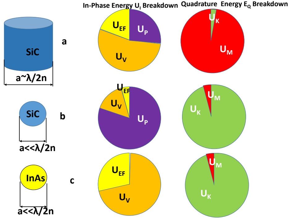
Fig.3 The breakdown of energies in three different resonant structures in mid-IR region (a) dielectric resonator (b) localized surface phonon polariton (c) localized surface plasmon polariton
