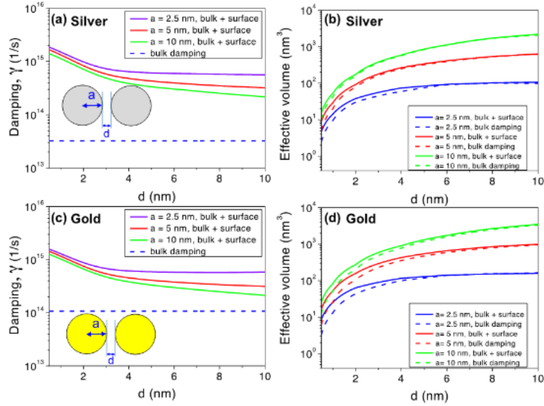
Fig. 6. (a) Total damping (solid lines) in the silver dimer as a function of gap width for three different radii compared with bulk damping (dashed line). (b) Effective mode volume as a function of gap width with (solid lines) and without (dashed lines) surface collisions. Corresponding results for the gold dimer in (c) and (d).
