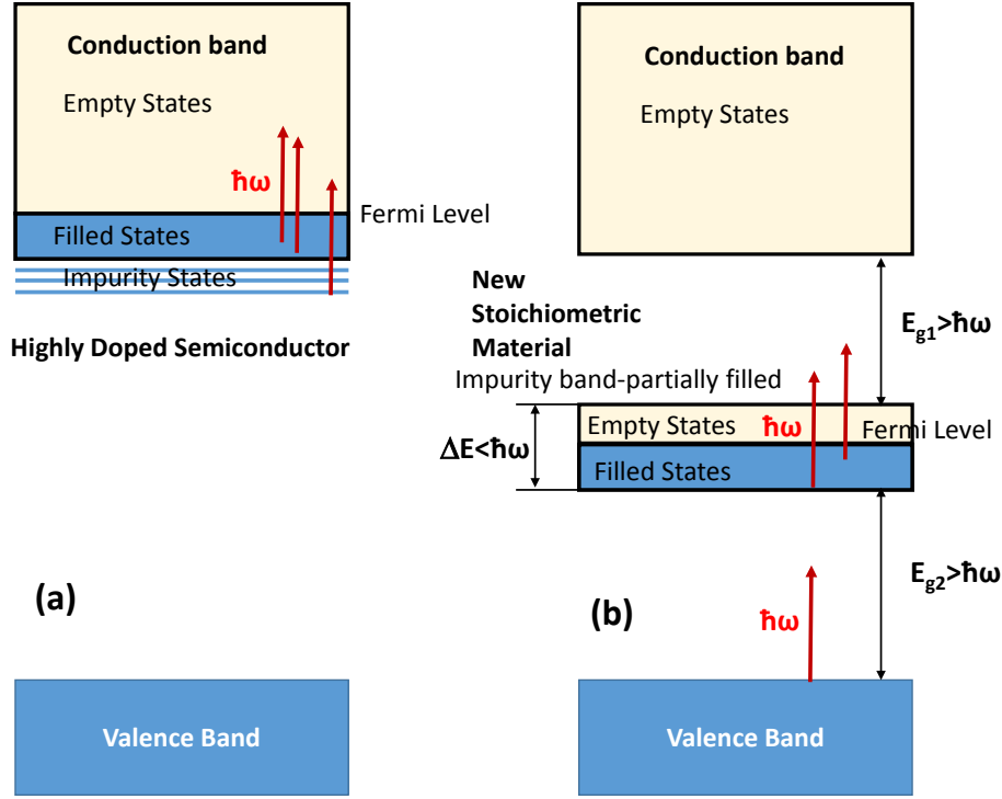
Fig.8 (a) Highly doped semiconductor with strong absorption. (b) Novel stoichiometric material that exhibits no absorption in a range of frequencies that are too high for the intraband absorption and too low for the interband absorption.
