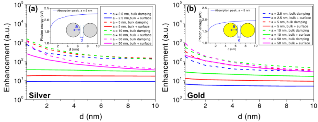
Fig. 7. Maximum enhancement as a function of gap width in (a) silver and (b) gold dimers of four different radii with (solid lines) and without (dashed lines) LD.
