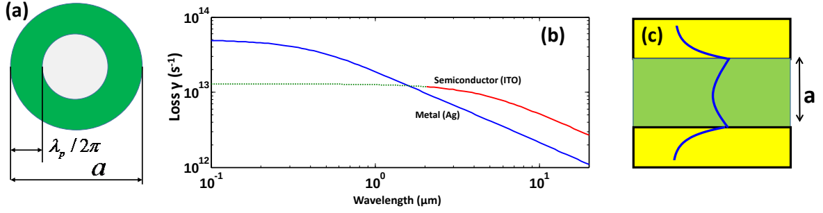
Fig. 1. (a) Cylindrical nanoparticle (b) Effective loss of the nanoparticle SPP for metal (Ag) and “new Plasmonic material” (ITO) (c) Gap plasmon
