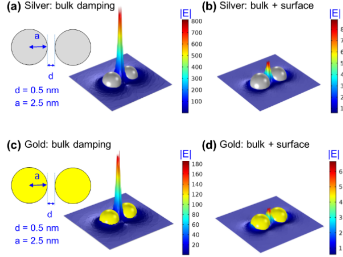
Fig. 5. SPP Field distribution in the silver dimer ( a=2.5 nm and d=0.5 nm) taking into account (a) only bulk damping and (b) both bulk and surface damping, and corresponding results for the gold dimer of equal dimensions in (c) and (d).
