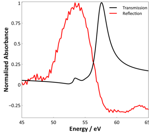
Figure 3: Normalized static spectrum of \text{Fe}_2\text{O}_3 as measured by Reflection-Absorption (red) and transmission (black) experiments.
