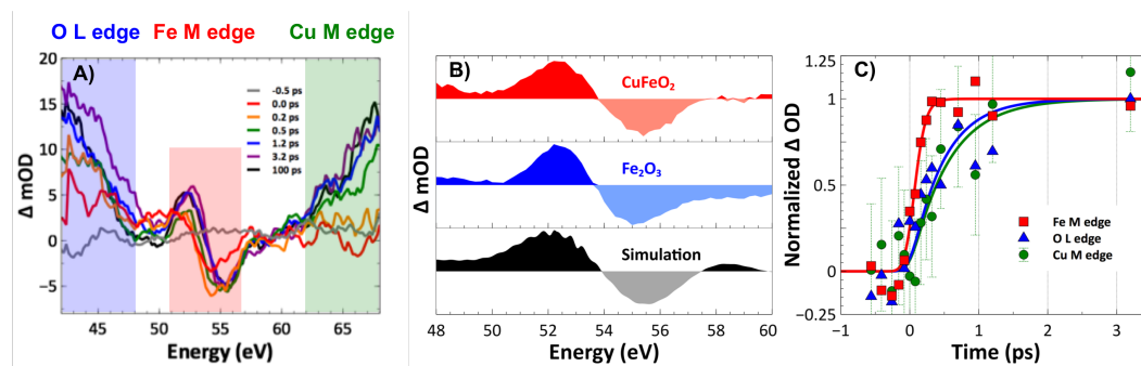
Figure 8: (A) Transient XUV-RA spectra of \text{CuFeO}_2 for a series of time delays. (B) Comparison of the XUV transient spectrum at the Fe M_{2,3} -edge obtained 1 ps following photoexcitation for \text{CuFeO}_2 and \text{Fe}_2\text{O}_3 along with the result of a ligand field multiplet simulation depicting the expected transient spectrum. (C) Kinetic traces showing the transient response at the Fe M_{2,3} -edge, the Cu M_{2,3} -edge, and the O L_1 -edge. Traces have been normalized and plotted as positive \Delta\text{OD} for clarity. Representative standard errors based on replicate measurements are shown for the Cu M_{2,3} -edge.
