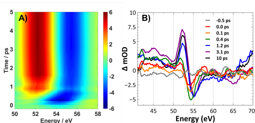
Figure 6: (A) The experimental contour plot for \text{Fe}_2\text{O}_3 up to 5 ps post-excitation. (B) \text{Fe}_2\text{O}_3 after photoexcitation at 400 nm depicting the spectral evolution up to 10 ps post-excitation.
