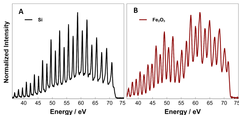
Figure 2: XUV harmonic spectrum generated in Ne gas as measured after reflectance from a Si mirror (A) and from a Fe 2 O 3 sample (B).
