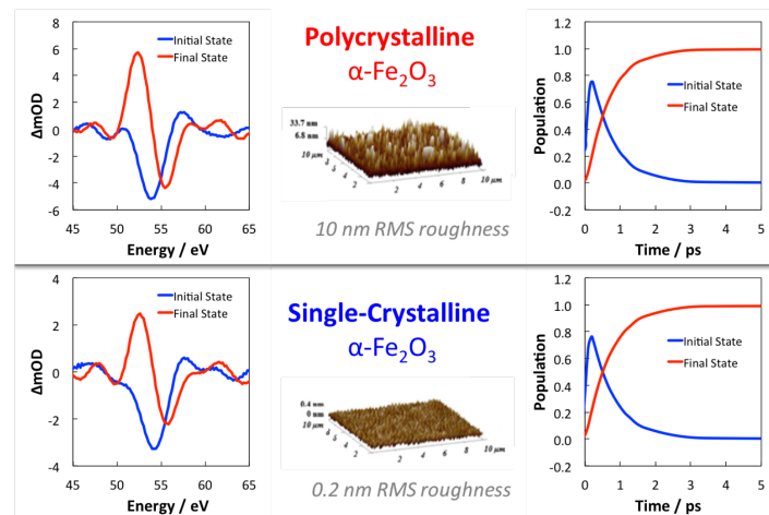
Figure 7: Comparison of transient electron dynamics for polycrystalline (top) and single crystalline (bottom) \text{Fe}_2\text{O}_3 .
