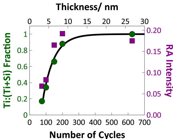
Figure 5: The experimentally determined probe depth for XUV-RA spectroscopy and XPS. Fitting an exponential rise to the XPS data points yields a probe depth of 2.8 nm (shown by the black line).
