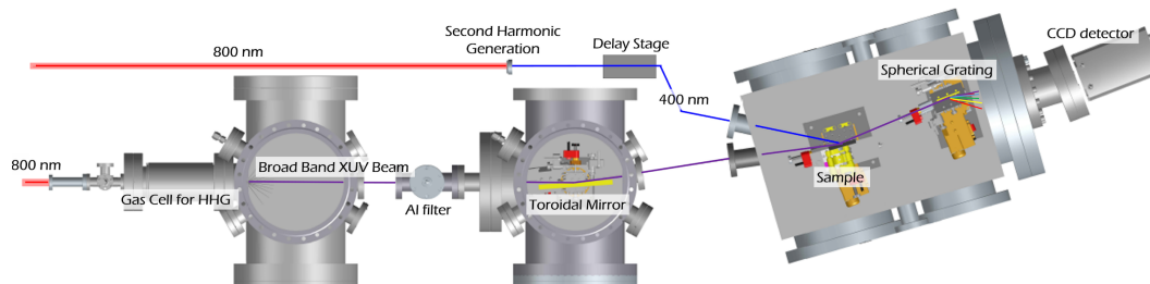
Figure 1: Overview of the XUV-RA spectrometer. Semi-infinite gas cell (40 cm) is used for HHG. Residual driving field is removed with an Al filter. Toroidal mirror is used to focus the XUV radiation onto the sample after which it is spectrally dispersed onto a CCD camera by a spherical grating. The 400 nm pump beam is generated by frequency doubling the 800 nm fundamental.
