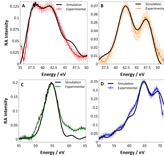
Figure 4: Simulated (black) and experimental (color) static XUV-RA spectra of (A) \text{TiO}_2 , (B) \text{Cr}_2\text{O}_3 , (C) polycrystalline \text{Fe}_2\text{O}_3 and (D) \text{NiO} . The error bars on the experimental spectra are the standard deviation associated with each data point.
