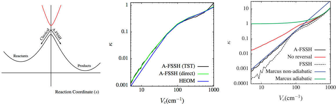
Figure 2: ( left ) A schematic diagram highlighting how we calculate nonadiabatic rates with a combination of transition state theory (TST) and augmented surface hopping dynamics (A-FSSH) (from Ref. 7 ): trajectories are run backwards classically (which ignores branching and decoherence) and run forwards with surface hopping dynamics (which includes branching and decoherence). ( middle ) A-FSSH results for the spin-boson model; we plot the electron transfer transmission factor ( \kappa ) as a function of the diabatic coupling ( V_c ). Despite the many approximations in our algorithm, note that our TST surface hopping results do agree with direct A-FSSH calculations as well as exact hierarchical equation of motion (HEOM), which is a strong endorsement of our heuristic approach. ( right ) Here, without friction, we compare the A-FSSH transmission factor versus classical Marcus theory in the nonadiabatic and adiabatic limits. Note that A-FSSH interpolates correctly between the two different limits, outperforming FSSH (which ignores decoherence) and again endorsing the TST-AFSSH approach. Note also another discovery of Ref. 7 : surface hopping results without velocity reversal upon a forbidden hop can yield quite erroneous answers.
