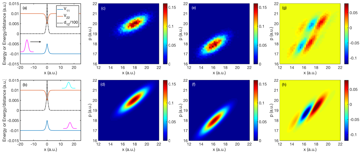
Figure 1: Understanding Tully’s FSSH algorithm through a partial Wigner transform. (a) The setup for Tully model problem #1: A nuclear wavepacket (in pink) approaches an avoided crossing from the left coming in along the lower adiabat ( V_{11} in blue). This wavepacket can either remain on the lower adiabat or jump to the upper adiabat ( V_{22} in red). The derivative coupling d_{12} is plotted in black. (b) The wavepackets on the lower and upper adiabatic surfaces are slightly separated at a later time. (c) – (h): The partial Wigner transforms for the system at that later time. (c) A_{11}^{FSSH} , (d) A_{11}^{exact} , (e) A_{22}^{FSSH} , (f) A_{22}^{exact} , (g) \text{Real}((A_{12}^{FSSH})) , (h) \text{Real}((A_{12}^{exact})) . Note that surface hopping calculations do recapitulate partial Wigner transforms for the populations on surfaces 1 and 2: this agreement endorses surface-hopping as an approximate solution to the QCLE. That being said, there are errors in the 1-2 coherences, which present a difficulty for the surface-hopping ansatz when analyzing spectroscopy. 13
