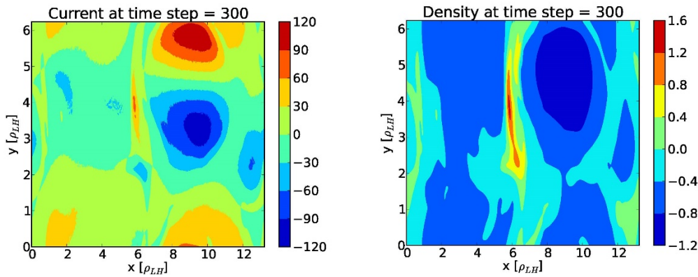
Fig. 7a. Large scale structures in density (right) and electric current (left), From Ref. 1
