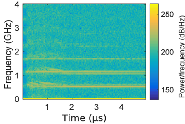
Figure 15. Development of multiple unstable cyclotron modes of the \mathbf{E} \times \mathbf{B} instability as a function of time. Amplitude of higher harmonics reduces with time.
