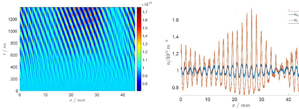
Fig. 8. Coherent density structure generated by ExB instability (left). Nonlinear modulational instability resulting in inverse cascade and energy transfer to long wavelengths (right) in nonlinear kinetic simulations. From Ref. 7.
