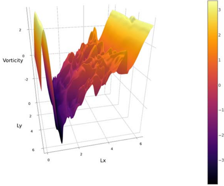
Fig. 9. The dimensionless amplitude of the vorticity from 2D nonlinear simulations. The small scale modes exist on the background of large axial mode, L_x is axial direction, and L_y is azimuthal direction of the Hall thruster.
