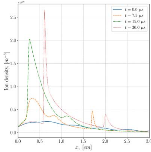
Figure 11. Axial propagation of the ion density structures in the model with ionization effects.
