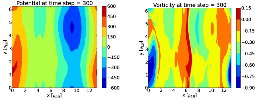
Fig. 7b. Large scale structures in potential (left) and vorticity(right), From Ref. 1
