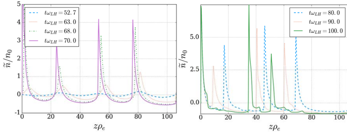
Fig. 10. Nonlinear development and axial motion of large scale (axial) modes (plasma density); compare with Fig 8. Here, z is the axial direction of the Hall thruster, From Ref.6.
