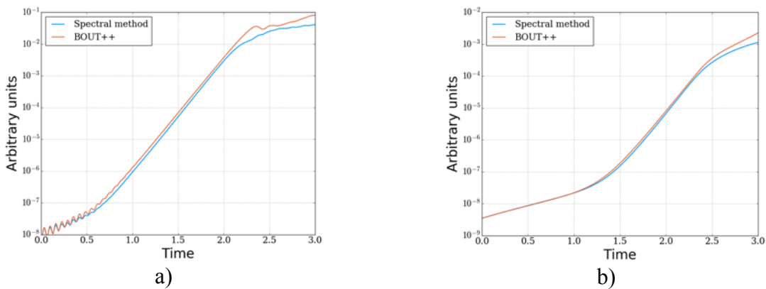
Fig. 5. Comparison of density a) and potential fluctuations b) in nonlinear simulations with BOUT++ and pseudo-spectral code.
