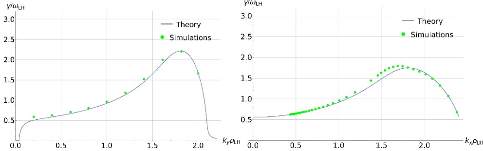
Fig 4. Linear benchmark of BOUT++ simulations against the theoretical eigen-value solutions.
