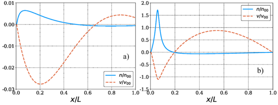
Figure 12. (a) Eigen-functions of density and ion velocity perturbations. (b) Stationary profiles of density and ion velocity.
