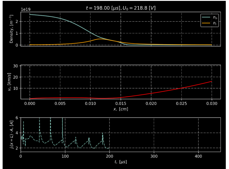
Fig. 14a: Nonlinear development of axial modes taking into account the ionization effects, at time t=198 ms
