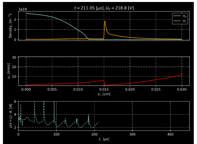
Fig. 14c: Nonlinear development of axial modes taking into account the ionization effects, at time t=211 ms.
