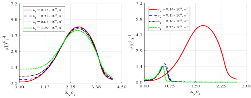
Fig 13. Growth rate of gradient-driven mode as a function of the wave-vector for different ionization frequencies (corresponding to different neutral pressure): direct effect of neutral pressure (left), effect of neutral pressure and temperature reduction are included (right).
