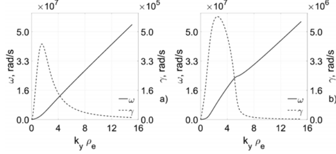
Fig. 1. Effect of the gyro-viscosity and conversion into the ion sound mode, note the almost linear dependence on the wave-vector corresponding to the ion sound dispersion, \omega = k_y c_s . (a) Destabilization of the ion-sound mode by density gradient and collisions; (b) Destabilization by density gradient, \mathbf{E} \times \mathbf{B} drift and collisions.
