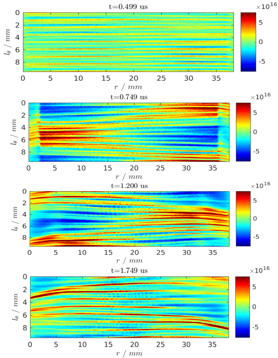
Figure 16. Snapshots of ion density fluctuations in the simulation over four distinct regimes of non-linear evolution. First, modes saturate and assume an amplitude-modulated form, then a strong cascade to low-k occurs. After this, the perturbations penetrate the sheath regions.
