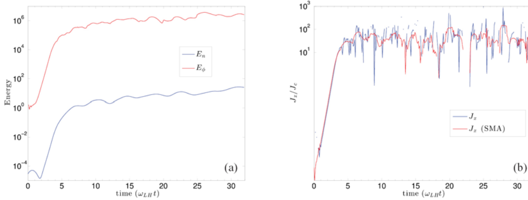
Fig. 6. The time evolution of the density and potential energy integrals (a); the time dependence of the anomalous current (in units of the classical collisional current) (b).
