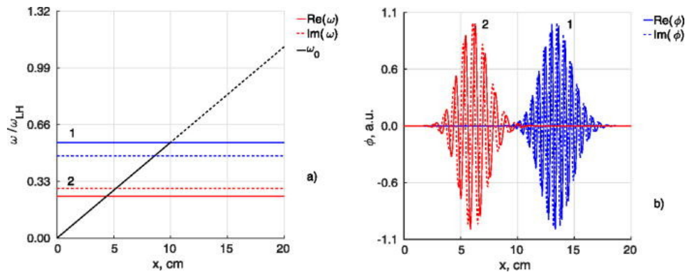
Fig. 3. The localized eigen-functions for the extended domain L=20 \text{ cm} , k_y = 100 \text{ m}^{-1} . The eigen-
