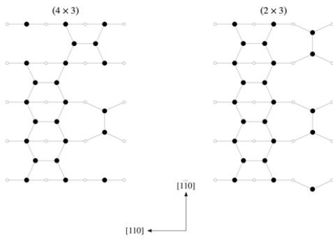
Figure 2.31 Prevailing (001) surface reconstructions during antimonide growth; [001] direction is out of the page. A single surface cell is shown for the (4 \times 3) case, and two consecutive (in the [1\bar{1}0] direction) surface cells shown for the (2 \times 3) case, respectively. Top-layer antimony dimers preferentially align with the [110] direction in both reconstructions. The dimers situated between [110] rows form a 2/3 ML “floating layer” of unincorporated antimony atoms.
