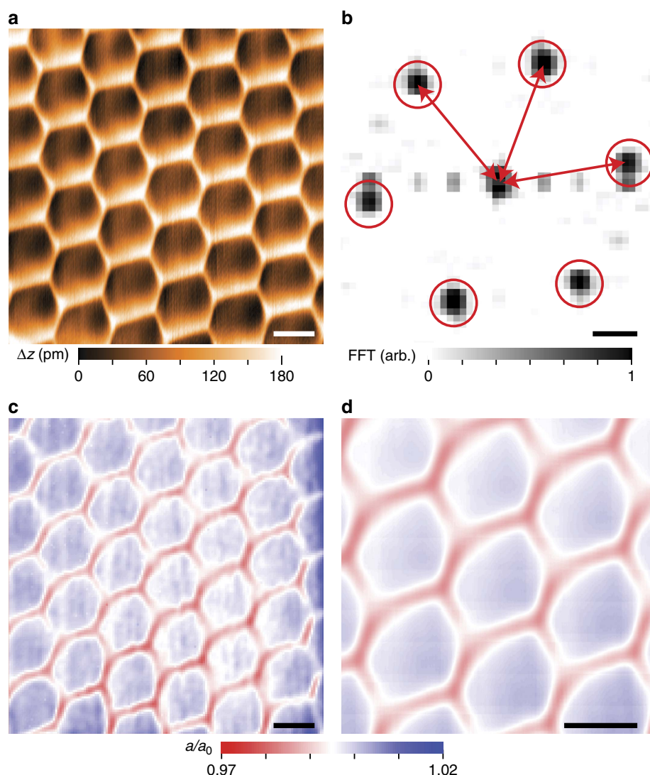
Figure 3 | Method for generating strain maps. (a) Atomically-resolved topography of nearly-aligned graphene on hBN. The topography was acquired with a sample voltage of V_s = 0.3 \text{ V} and a tunnelling current of I_t = 200 \text{ pA} . (b) Fourier transform of a 4 \times 4 \text{ nm}^2 region of (a), showing six resonances representing the hexagonal graphene lattice (red circles). The red arrows depict the measurement of the lattice constant in each direction. (c) Plot of the average length of the three lattice directions, as measured in (b) for each point in the topographic map. The points are normalized by the equilibrium graphene lattice constant a_0 . (d) Spatially-averaged strain map, generated by averaging (c) over a few moiré unit cells. The scale bars are 10 \text{ nm} for (a,c,d) and 10 \text{ nm}^{-1} for (b).
