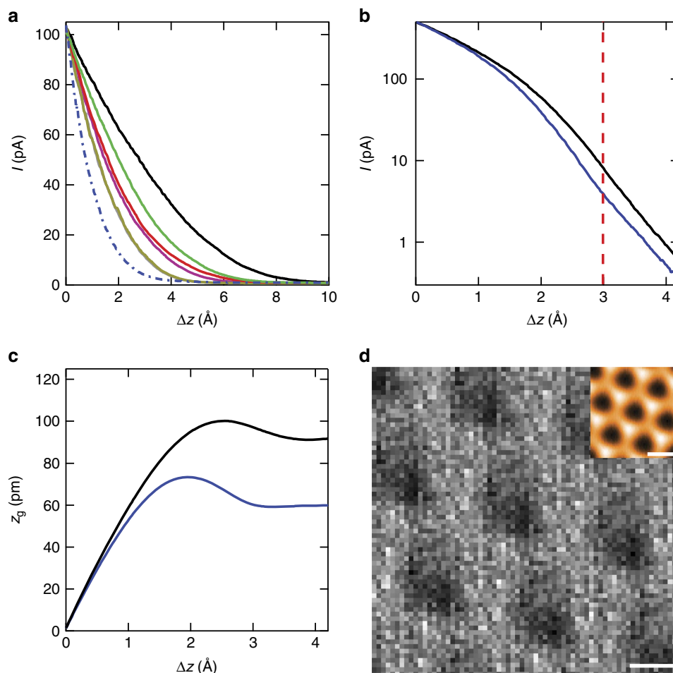
Figure 2 | Tunneling current as a function of tip-sample separation. (a) Measurement of the tunnel current I versus tip retraction distance \Delta z for nearly-aligned graphene on hBN, starting with the tip in close proximity to the sample. The dot-dashed blue curve is taken on graphene on SiO 2 for reference, and exhibits the anticipated exponential decay. The remaining curves, from gold to black, represent decreasing sample bias (that is, moving the tip closer to the surface), from 1 to 0.05 V. The decay is initially parabolic, and the crossover point to exponential decay grows to larger \Delta z as the sample bias is lowered. (b) Similar decay measurement plotted on a log scale on a CB (blue) and CN/AA (black) region. The transition from parabolic to linear occurs at \Delta z of about 2 Å. (c) Out-of-plane graphene movement relative to the hBN ( z_g ) as a function of tip separation \Delta z . As the tip is initially retracted, the graphene moves with it, lifting away from the hBN. At just over 2 Å, a maximum pulling distance is reached, and on further tip retraction the graphene slowly relaxes back towards the hBN. (d) Spatial map of the tunnelling current (dark is low and bright is high). The data are taken from the same set as in (b), at \Delta z = 3 Å. The inset displays the simultaneously acquired topography. The tunnelling current is smaller in the moiré centres than along the boundaries, suggesting a spatial modulation in the ability of the tip to pull the graphene off the hBN substrate. The maps have been spatially-averaged (see main text). Note that a similar pattern is exhibited at all \Delta z , as the blue curve is always below the black in (b). The scale bar is 5 nm for the main panel and 10 nm for the inset.
