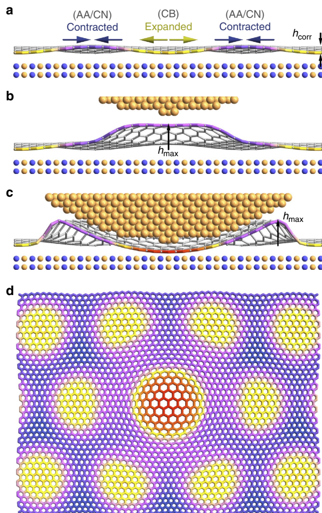
Figure 1 | Schematic of graphene on hBN and the influence of an STM tip.
