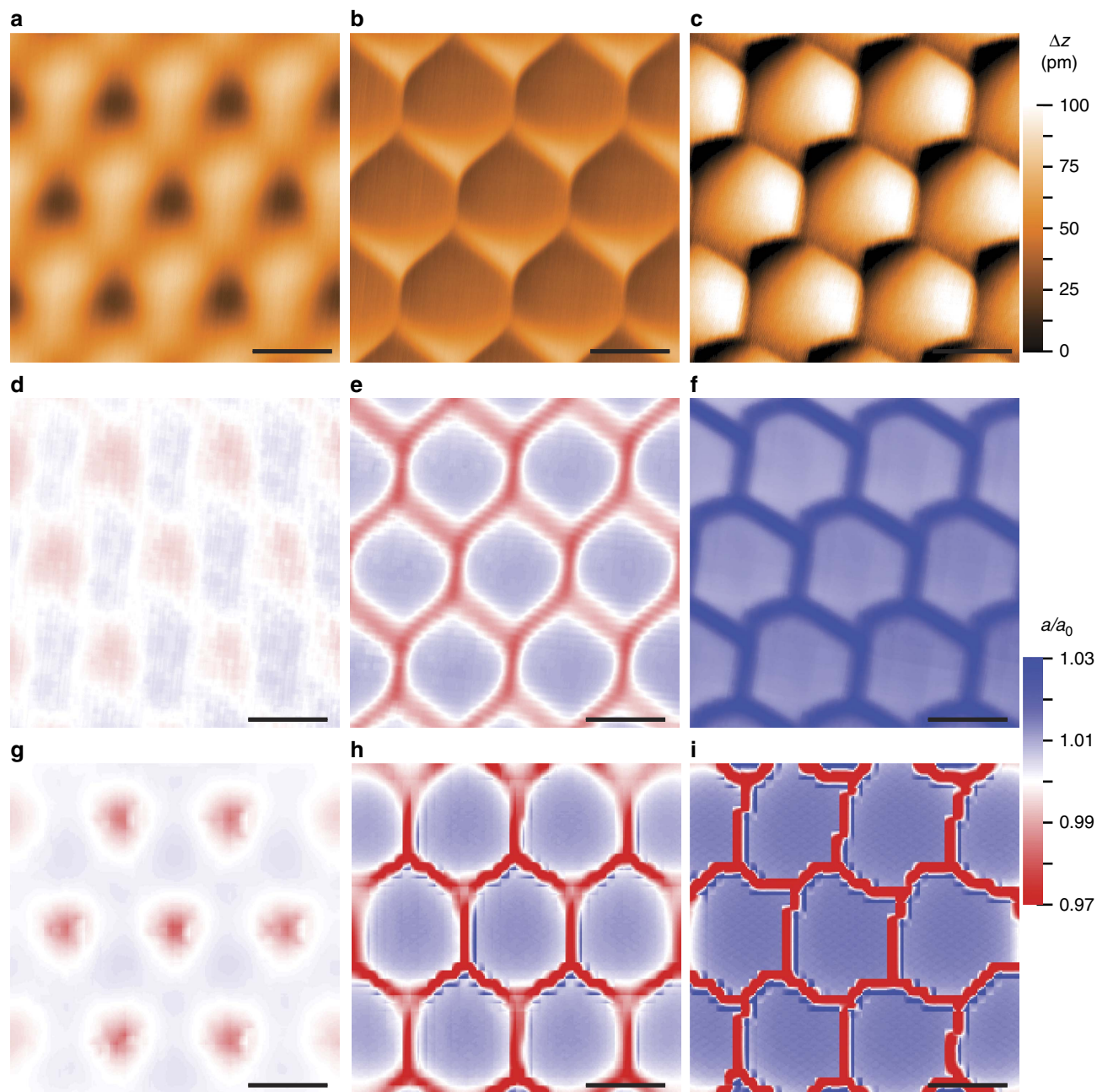
Figure 4 | Topography and strain maps in different interaction regimes. (a–c) Spatially-averaged topography maps acquired over the same region of a nearly-aligned sample, with the tip moving progressively closer to the sample. The appearance of the stacking boundaries becomes sharper as the tip moves closer, and becomes hysteretic and asymmetric in (c). (d–f) Experimental spatially-averaged strain maps generated from the topographic maps of (a–c). In (d) the graphene lattice is compressed in the moiré centres and expanded along the boundaries. The opposite behaviour is observed in (e). In (f), the graphene lattice constant for the entire map is expanded, as the system is in a strongly interacting, hysteretic regime. (g–i) Simulated strain maps, showing excellent agreement with the experimental results. The disagreement in the dynamical strain at the stacking boundaries between (f) and (i) is attributed to the absence of out-of-plane buckling in the simulation. The tunnelling parameters are (a) V_s = 0.5 V and I_t = 50 pA, (b) V_s = 0.5 V and I_t = 900 pA and (c) V_s = 0.05 V and I_t = 100 pA. All scale bars are 10 nm.
