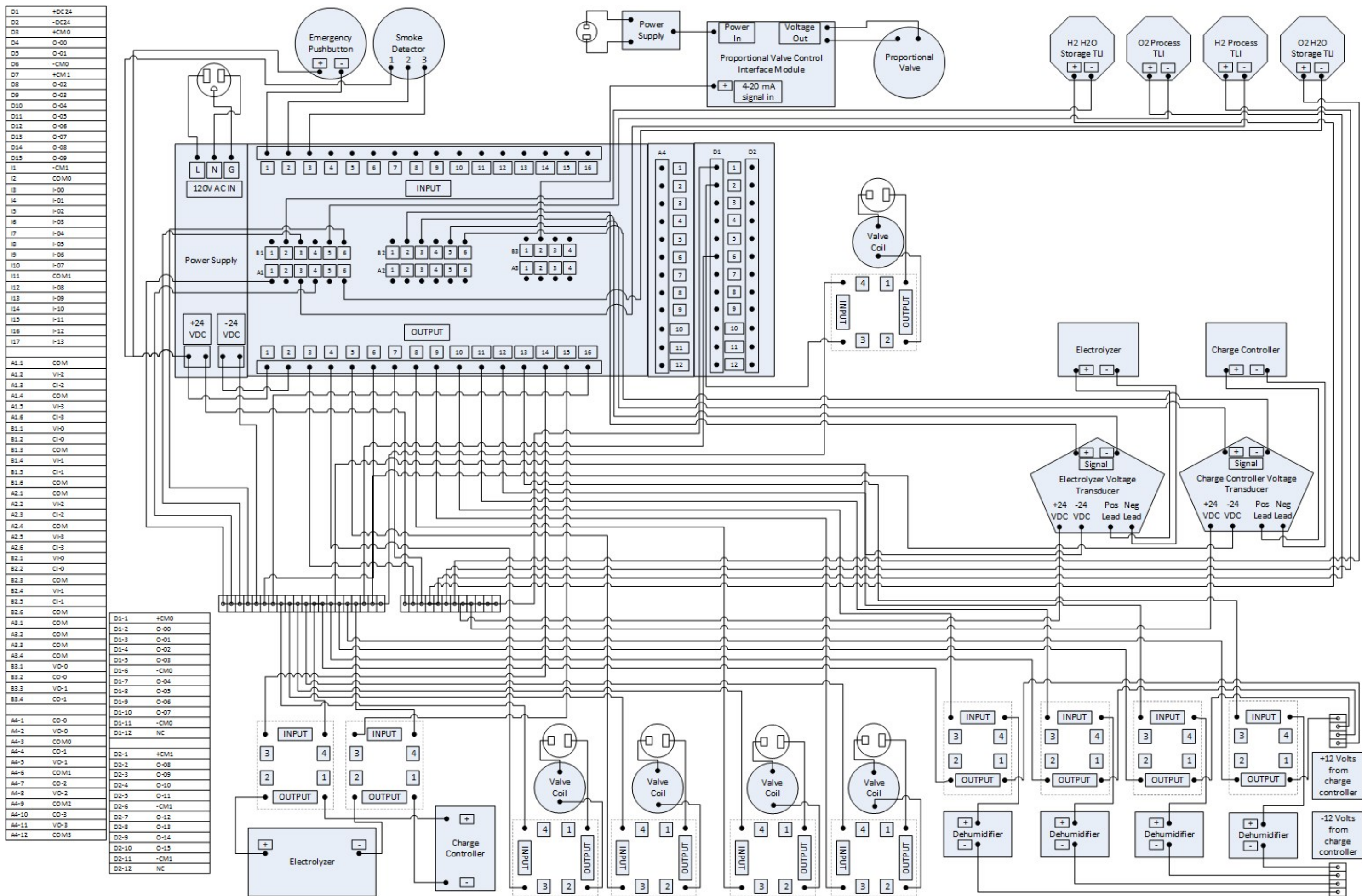
Figure 25. Hydrogen production facility automation electrical diagram.
