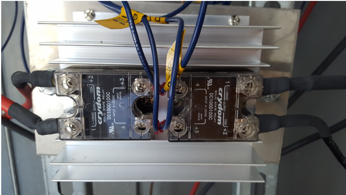
Figure 12. Crydom solid state relays used for electrolyzer control.
