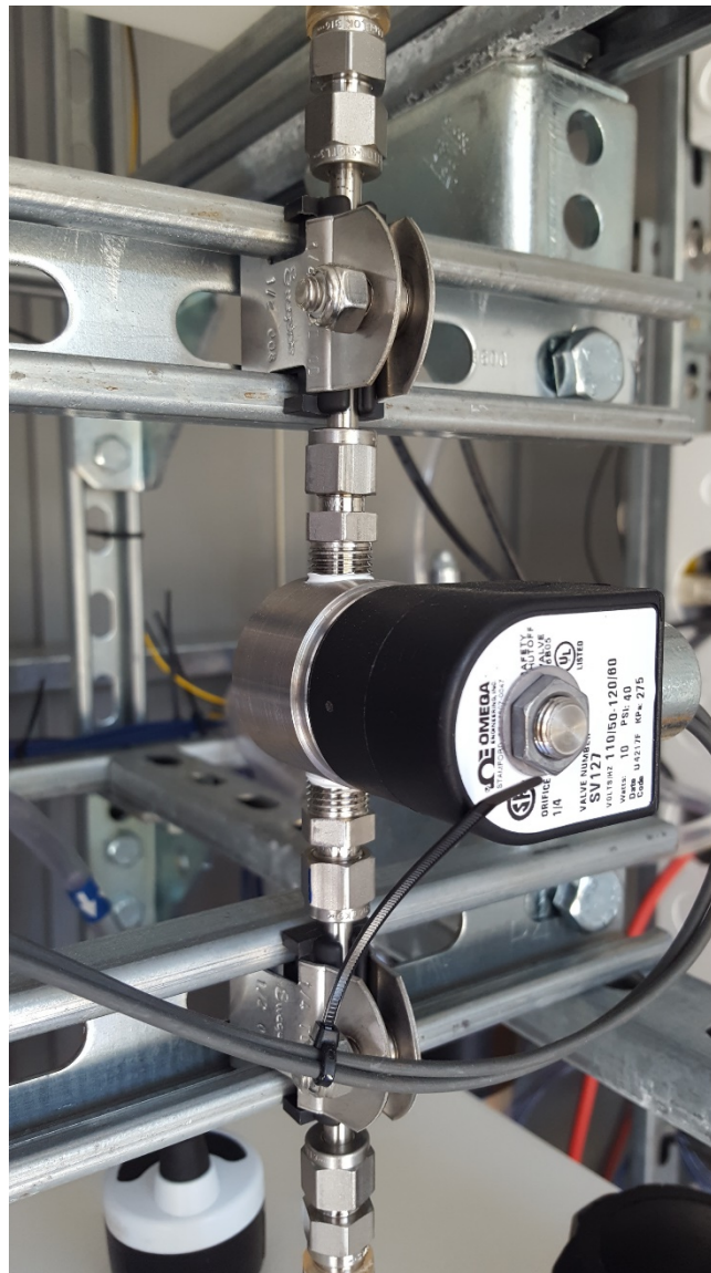
Figure 16. Omega SV127 normally closed fluid control valve.
